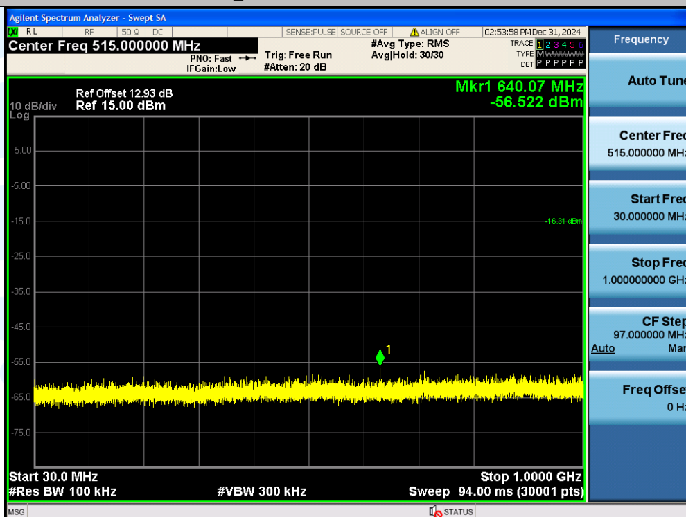
BLE_1M-Ant1-2480-30~1000-PASS
