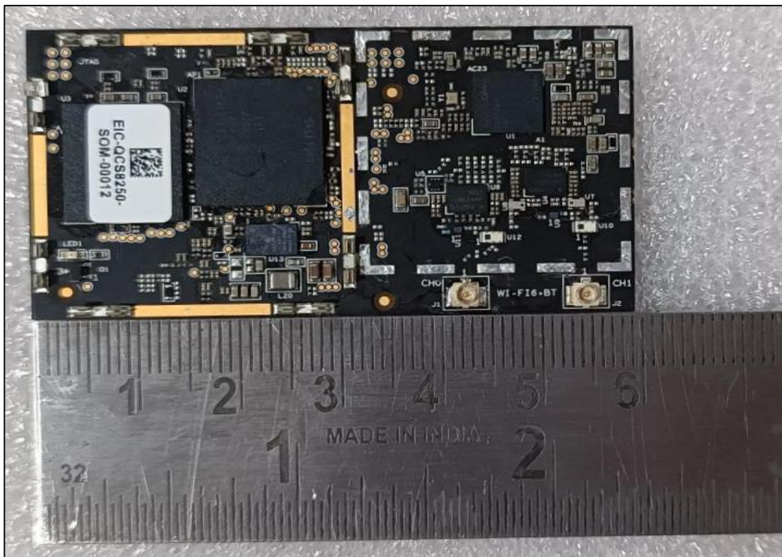
Module Front with Dimensional View
