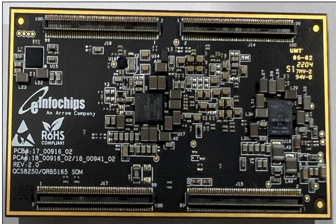
Module Rear View
