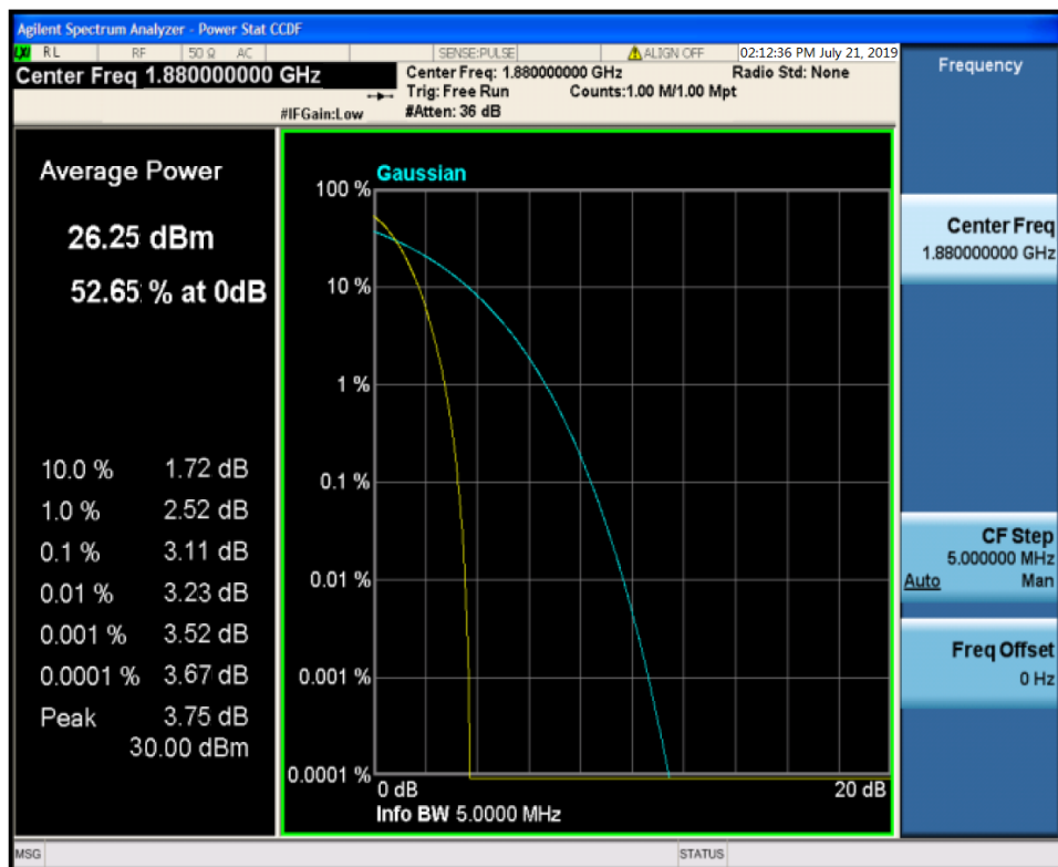
GSM1900 CHANNEL 661
