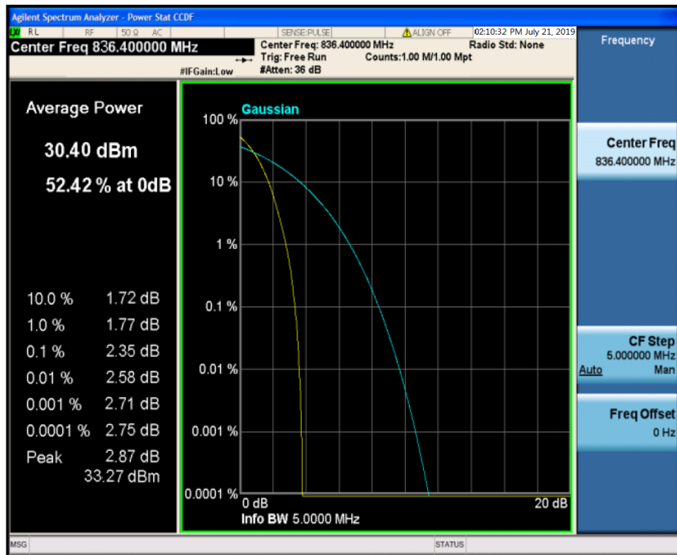
GSM850 CHANNEL 189
