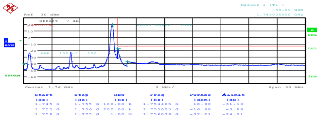
10MHz_High_QPSK_1@49 99.00dBm
