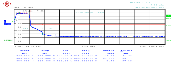
1.4MHz_High_16QAM_6@0 99.00dBm
