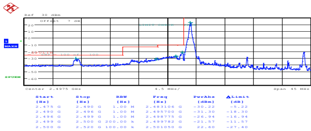
20MHz_Low_16QAM_1@0 99.00dBm
