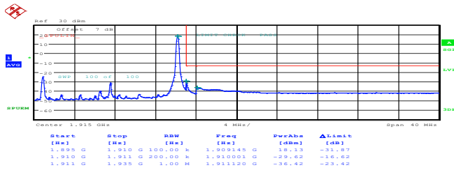
15MHz_High_16QAM_1@74 99.00dBm
