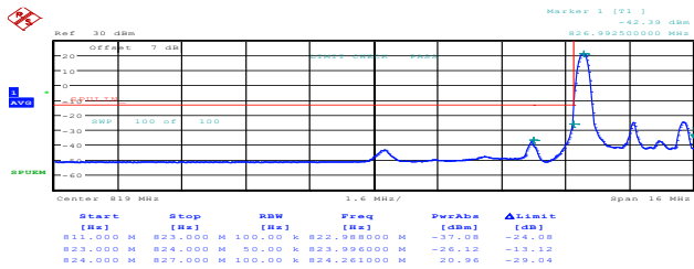
3MHz_Low_16QAM_1@0 99.00dBm
