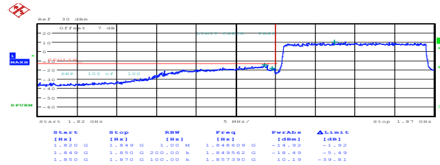
20MHz_Low_QPSK_100@0 99.00dBm
