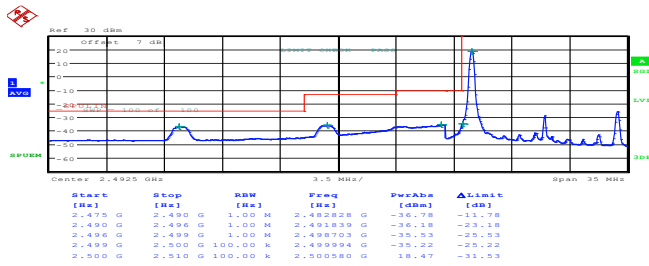
10MHz_Low_QPSK_1@0 99.00dBm
