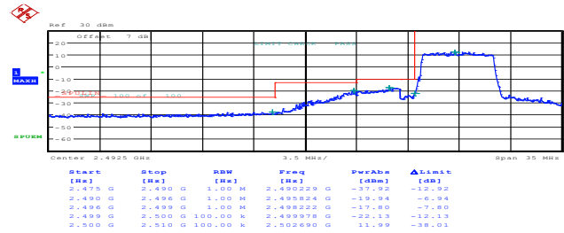
10MHz_Low_16QAM_27@0 99.00dBm
