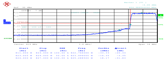
3MHz_Low_16QAM_15@0 99.00dBm
