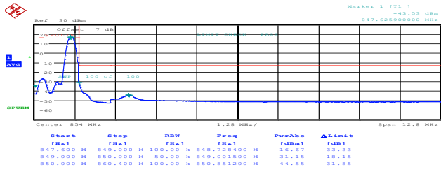
1.4MHz_High_16QAM_1@5 99.00dBm
