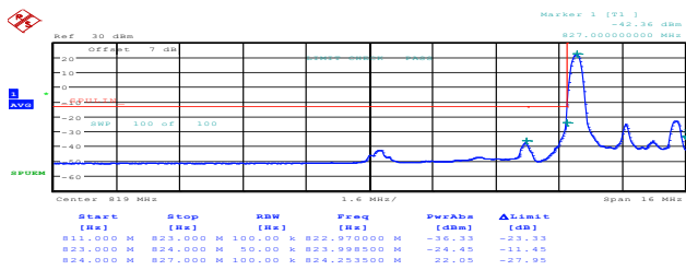
3MHz_Low_QPSK_1@0 99.00dBm
