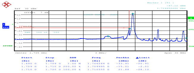
10MHz_Low_QPSK_1@0 99.00dBm
