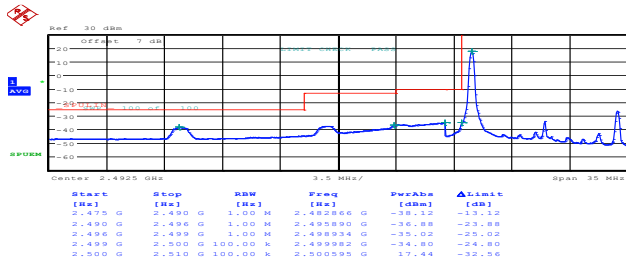
10MHz_Low_16QAM_1@0 99.00dBm
