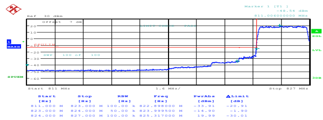
3MHz_Low_QPSK_15@0 99.00dBm
