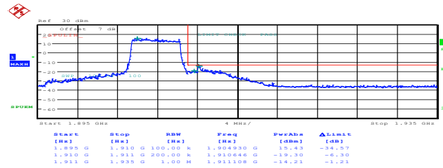
15MHz_High_16QAM_27@48 99.00dBm
