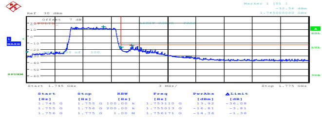
10MHz_High_16QAM_27@23 99.00dBm
