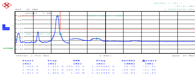
5MHz_High_16QAM_1@24 99.00dBm
