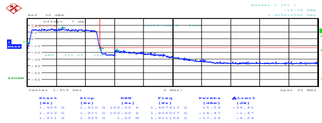
5MHz_High_16QAM_25@0 99.00dBm
