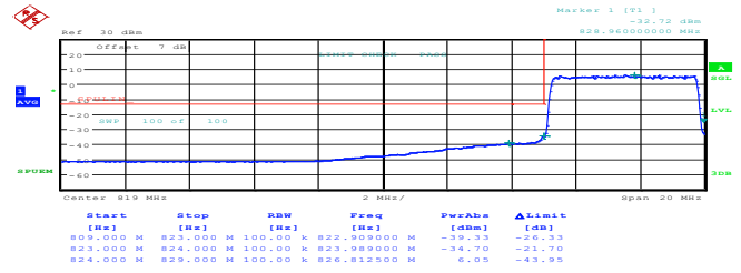
5MHz_Low_16QAM_25@0 99.00dBm
