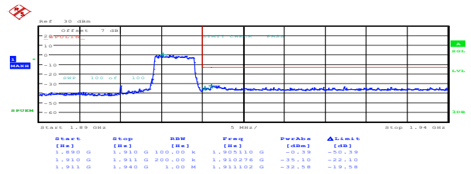
20MHz_High_16QAM_27@73 99.00dBm
