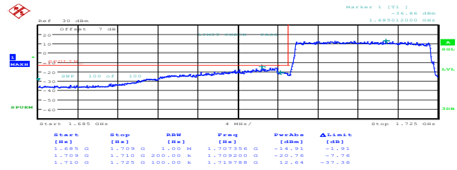
15MHz_Low_QPSK_75@0 99.00dBm
