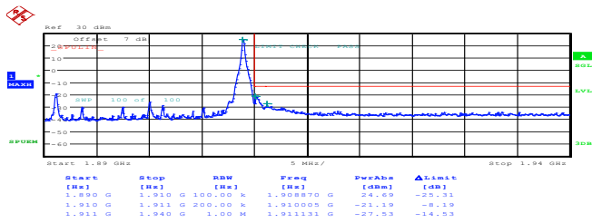
20MHz_High_16QAM_1@99 99.00dBm
