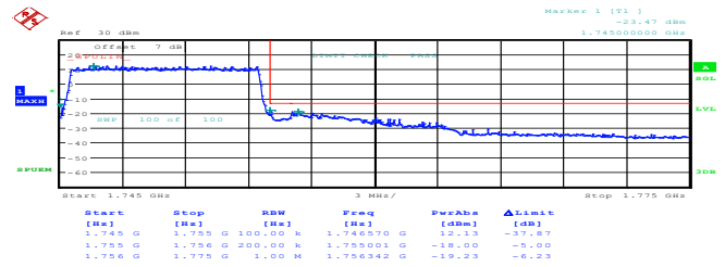
10MHz_High_QPSK_50@0 99.00dBm
