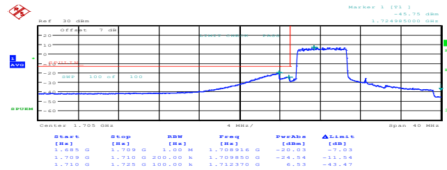
15MHz_Low_16QAM_27@0 99.00dBm
