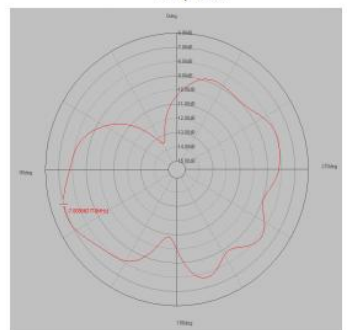
H plane
