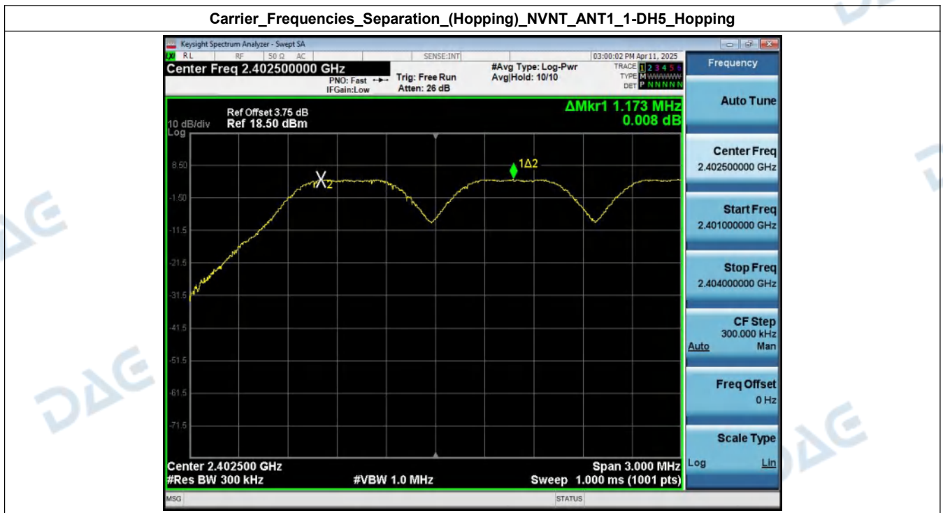
Carrier_Frequencies_Separation_(Hopping)_NVNT_ANT1_1-DH5_Hopping
