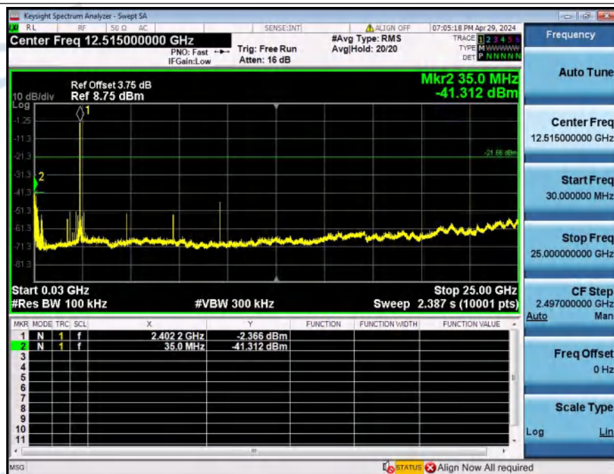
2_Spurious_Emissions_NVNT_ANT1_1-DH5_2402
