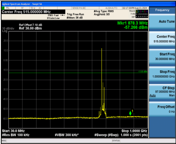
Band71_20MHz_16QAM_133372_1RB#0_30~1000_30~1000
