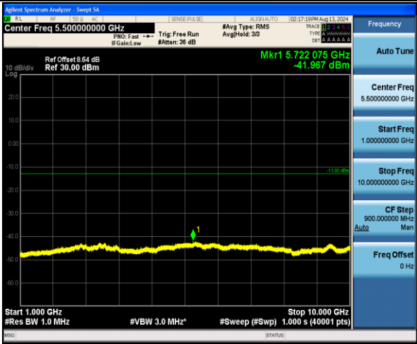
Band71_20MHz_QPSK_133372_1RB#0_1000~10000_1000~10000
