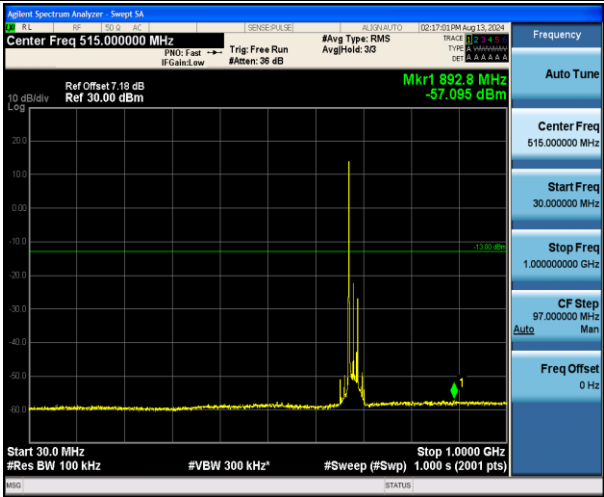
Band71_20MHz_QPSK_133372_1RB#0_30~1000_30~1000
