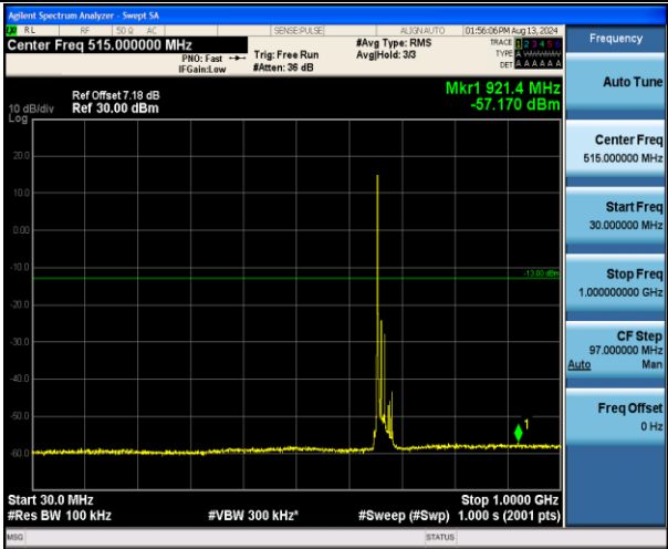
Band71_15MHz_QPSK_133197_1RB#0_30~1000_30~1000
