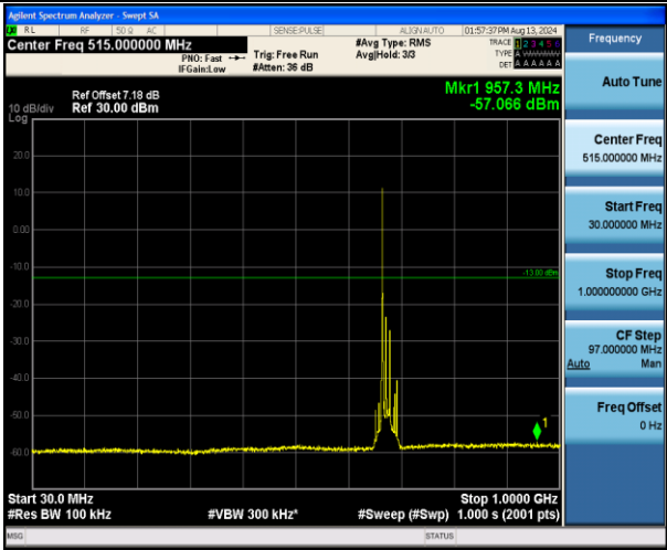
Band71_15MHz_16QAM_133297_1RB#0_30~1000_30~1000
