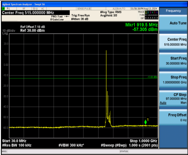
Band71_15MHz_16QAM_133197_1RB#0_30~1000_30~1000
