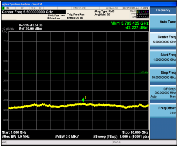
Band71_10MHz_QPSK_133422_1RB#0_1000~10000_1000~10000
