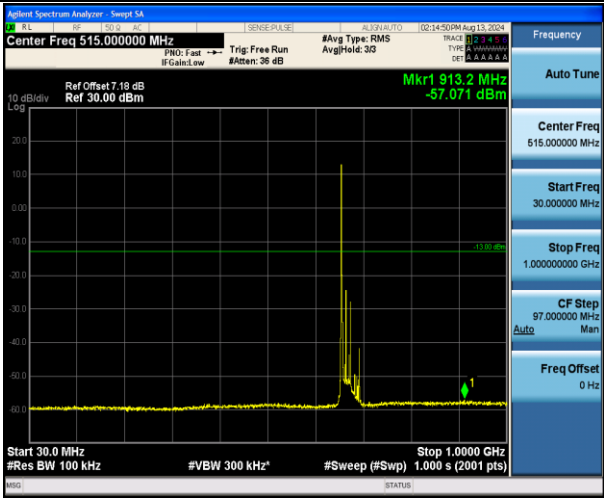
Band71_20MHz_QPSK_133222_1RB#0_30~1000_30~1000
