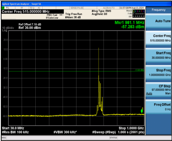
Band71_15MHz_QPSK_133297_1RB#0_30~1000_30~1000
