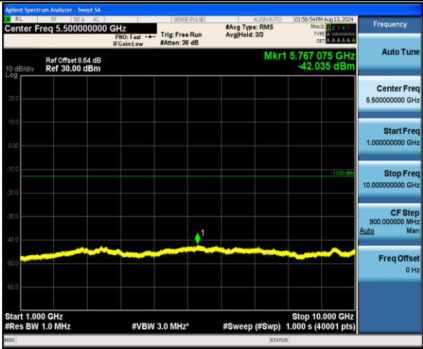
Band71_15MHz_16QAM_133197_1RB#0_1000~10000_1000~10000
