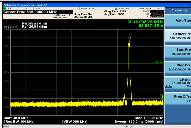
Band13-10MHz-16QAM-23230-50RB#0-30~1000MHz
