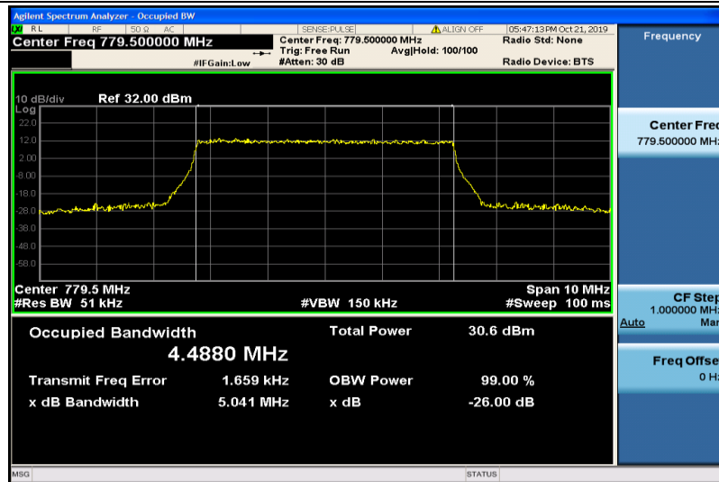
Band13-5MHz-16QAM-23205-25RB#0-4.4880
