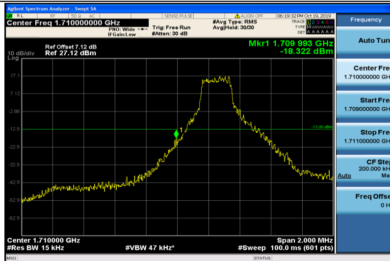
Band4-1.4MHz-16QAM-19957-1RB#0
