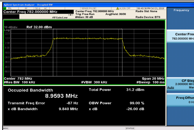
Band13-10MHz-16QAM-23230-50RB#0-8.9593
