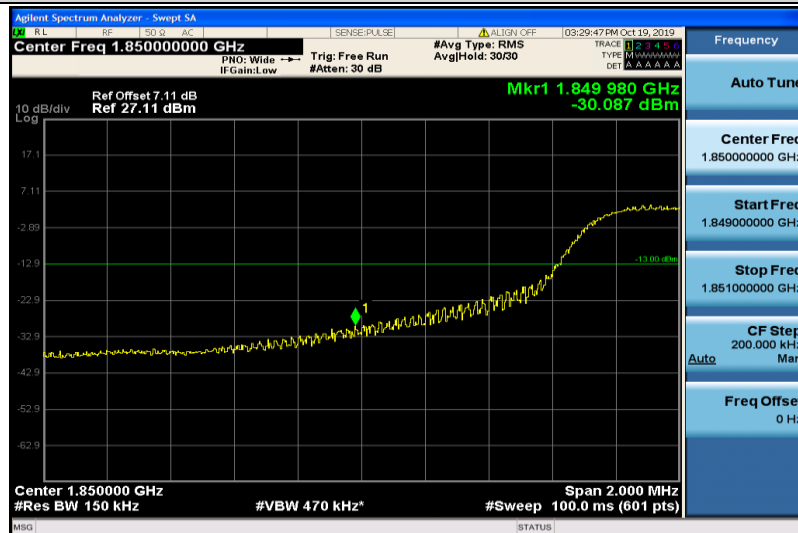
Band2-15MHz-16QAM-18675-75RB#0
