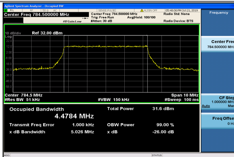
Band13-5MHz-QPSK-23255-25RB#0-4.4784
