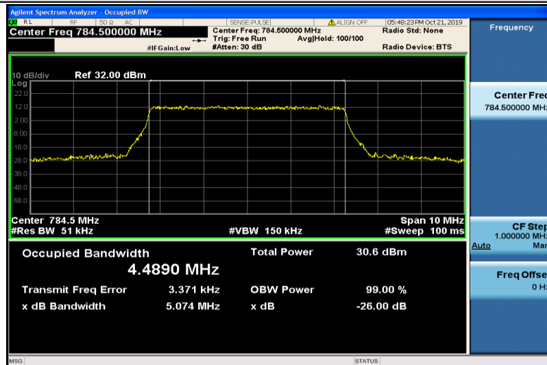
Band13-5MHz-16QAM-23255-25RB#0-4.4890
