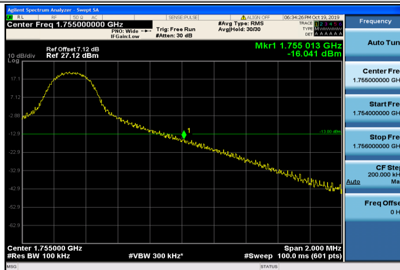
Band4-10MHz-16QAM-20350-1RB#49
