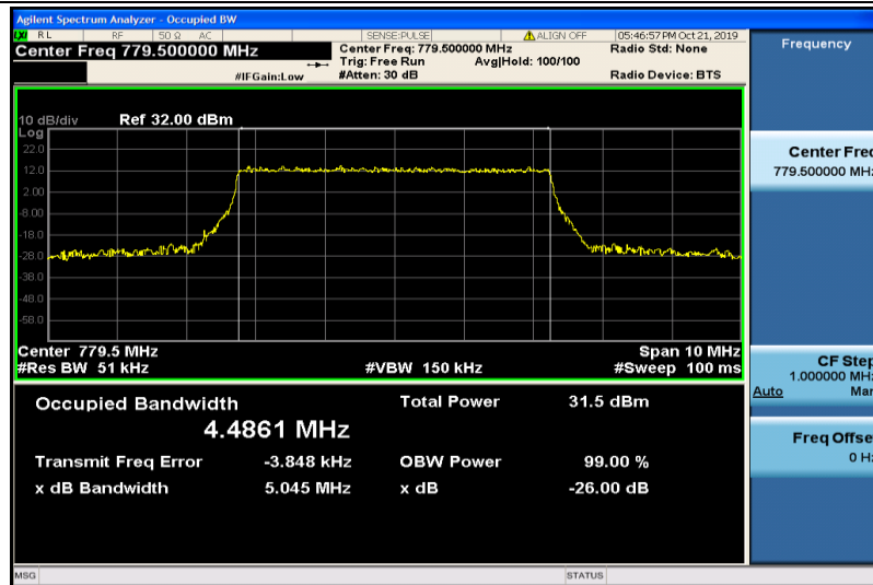
Band13-5MHz-QPSK-23205-25RB#0-4.4861
