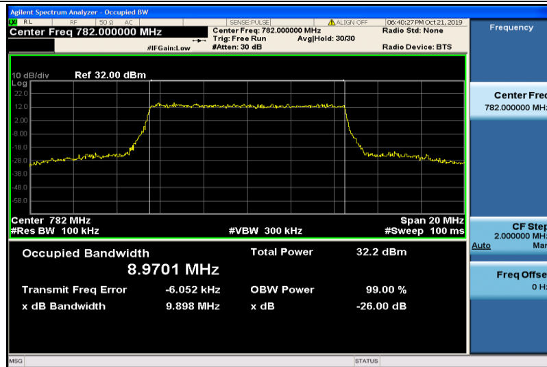
Band13-10MHz-QPSK-23230-50RB#0-8.9701
