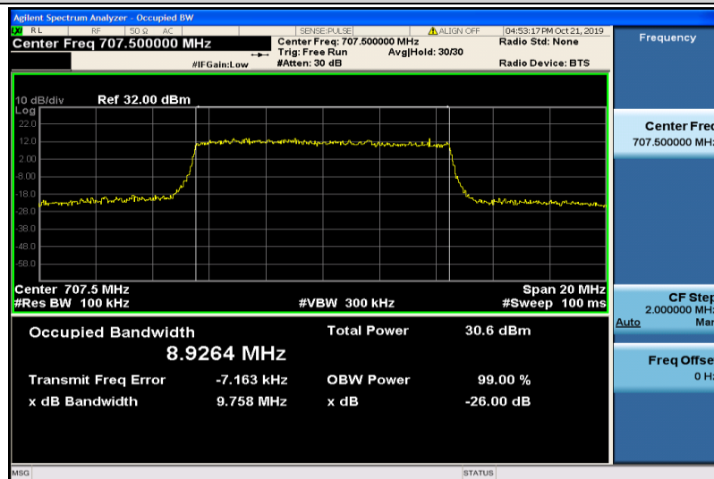
Band12-10MHz-16QAM-23095-50RB#0-8.9264
