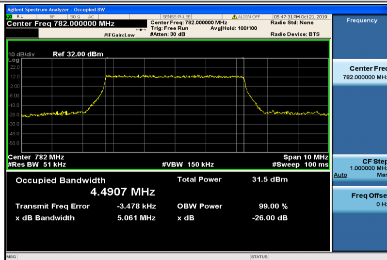
Band13-5MHz-QPSK-23230-25RB#0-4.4907
