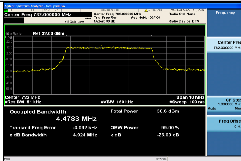
Band13-5MHz-16QAM-23230-25RB#0-4.4783
