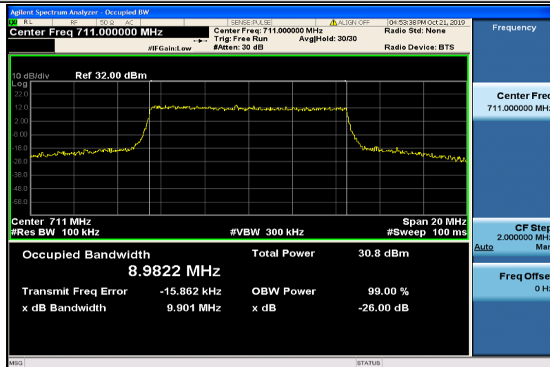
Band12-10MHz-16QAM-23130-50RB#0-8.9822
