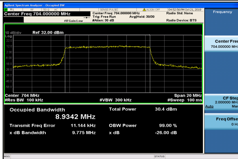
Band12-10MHz-16QAM-23060-50RB#0-8.9342
