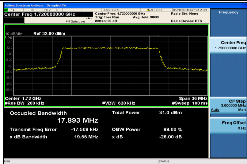
Band4-20MHz-QPSK-20050-100RB#0-17.893
