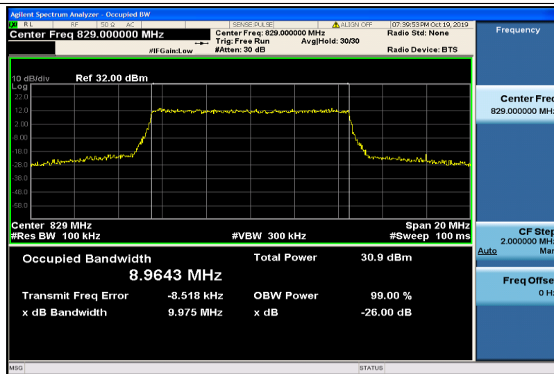
Band5-10MHz-QPSK-20450-50RB#0-8.9643
