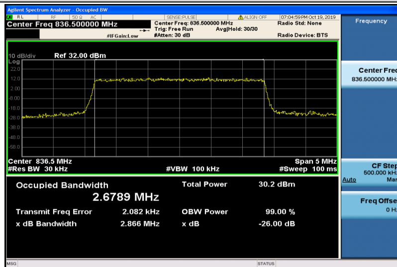
Band5-3MHz-QPSK-20525-15RB#0-2.6789
