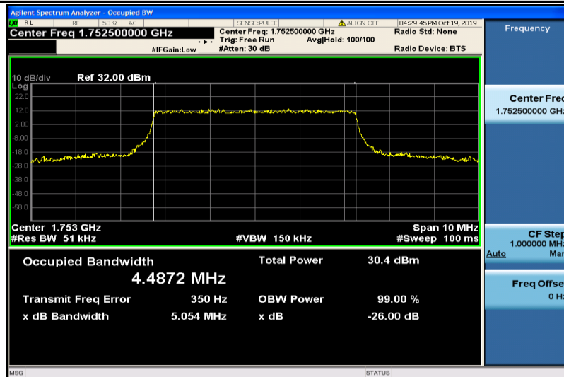
Band4-5MHz-QPSK-20375-25RB#0-4.4872
