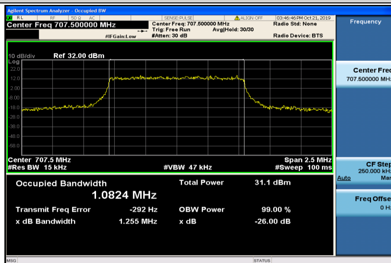
Band12-1.4MHz-QPSK-23095-6RB#0-1.0824
