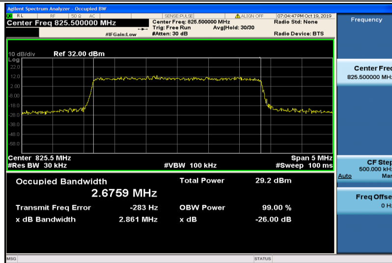
Band5-3MHz-16QAM-20415-15RB#0-2.6759
