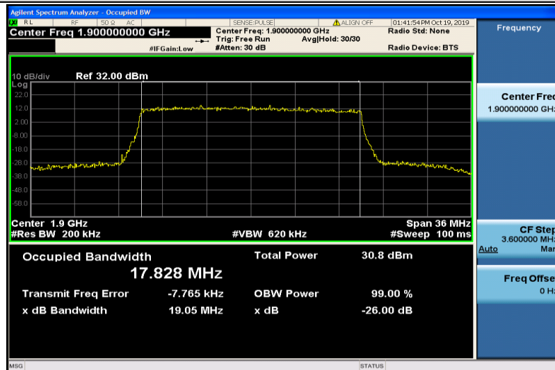
Band2-20MHz-QPSK-19100-100RB#0-17.828
