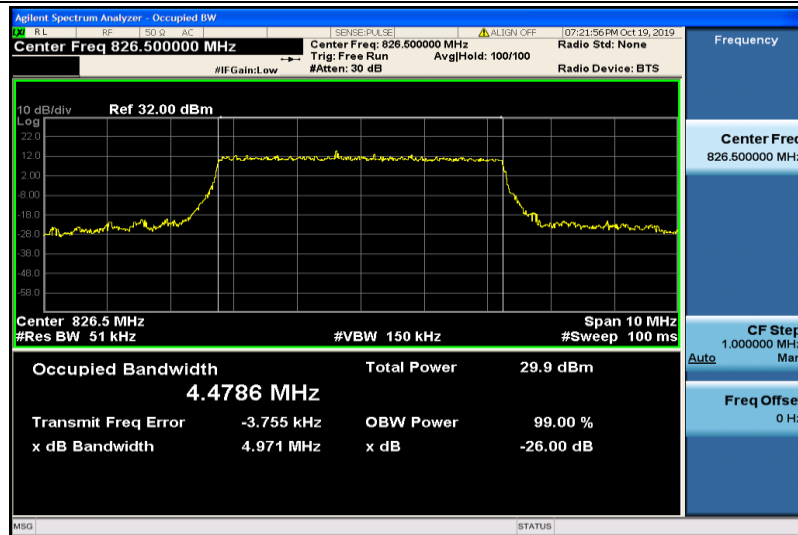
Band5-5MHz-16QAM-20425-25RB#0-4.4786
