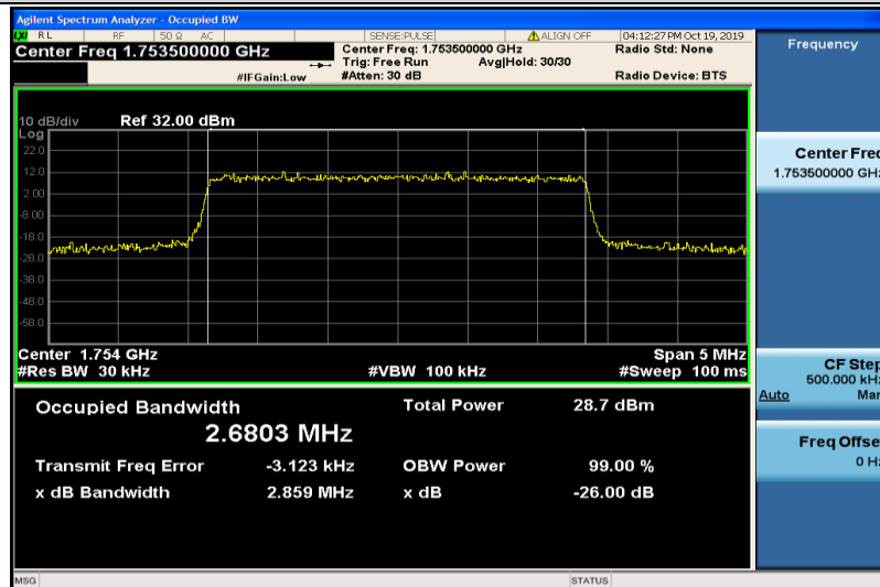
Band4-3MHz-16QAM-20385-15RB#0-2.6803
