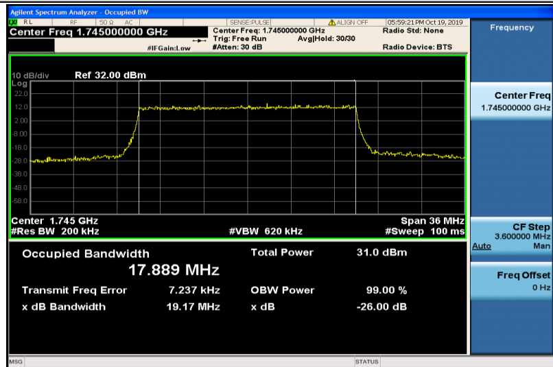
Band4-20MHz-QPSK-20300-100RB#0-17.889
