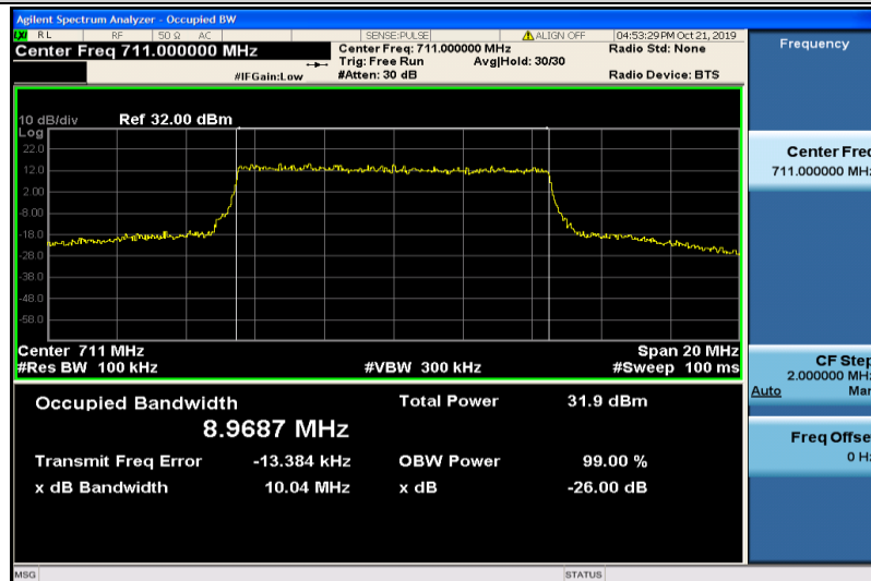
Band12-10MHz-QPSK-23130-50RB#0-8.9687
