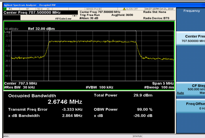
Band12-3MHz-16QAM-23095-15RB#0-2.6746
