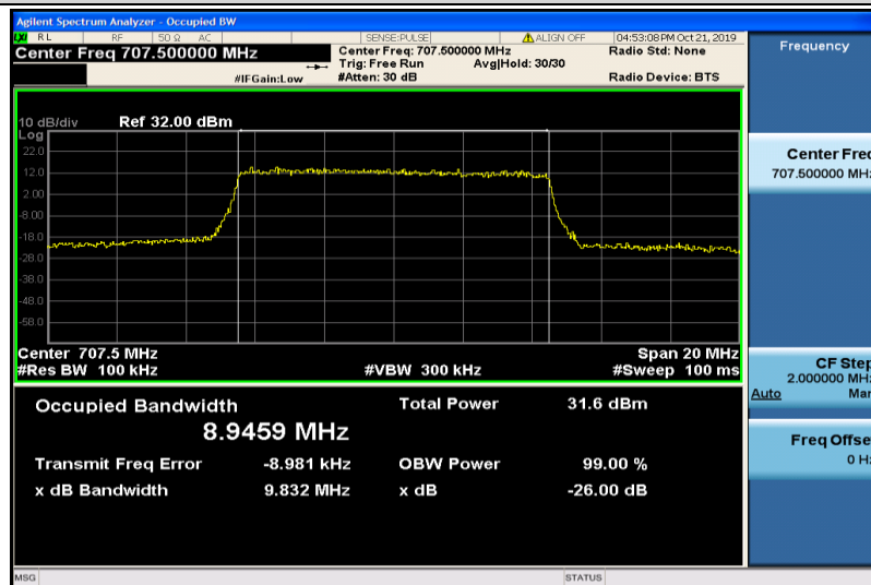
Band12-10MHz-QPSK-23095-50RB#0-8.9459
