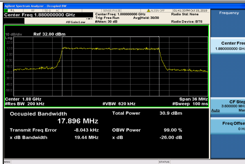
Band2-20MHz-QPSK-18900-100RB#0-17.896
