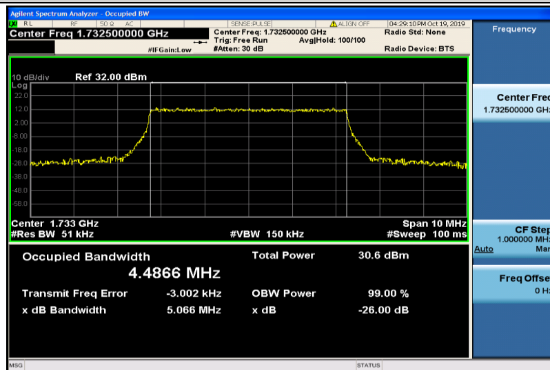
Band4-5MHz-QPSK-20175-25RB#0-4.4866
