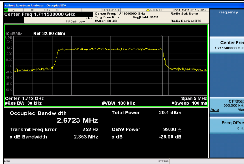
Band4-3MHz-16QAM-19965-15RB#0-2.6723
