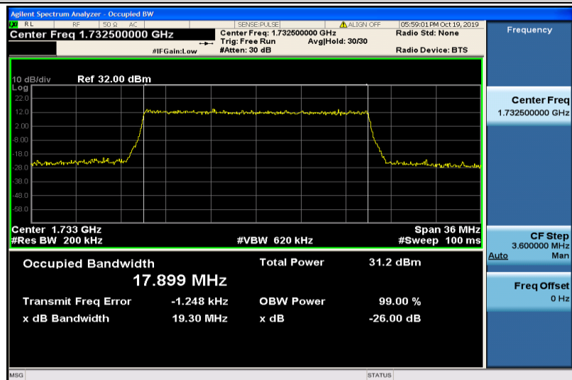
Band4-20MHz-QPSK-20175-100RB#0-17.899
