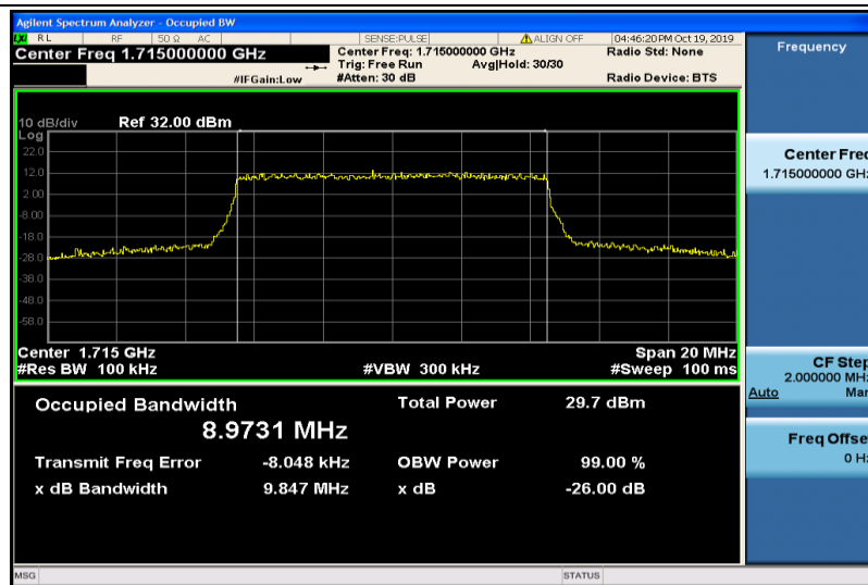
Band4-10MHz-16QAM-20000-50RB#0-8.9731
