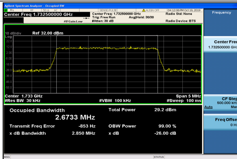
Band4-3MHz-16QAM-20175-15RB#0-2.6733
