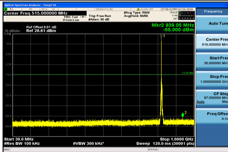
Band5-3MHz-16QAM-20415-1RB#0-30~1000MHz
