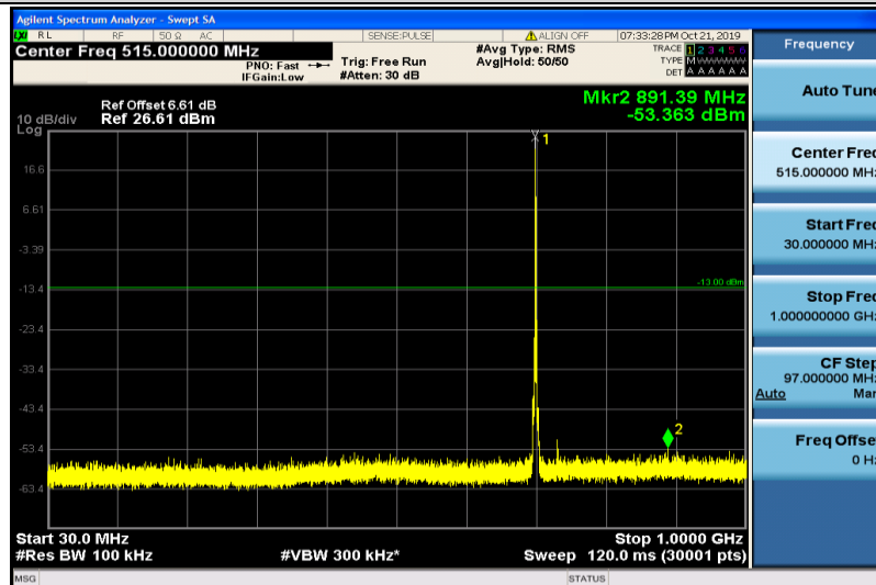
Band12-1.4MHz-QPSK-23095-1RB#0-30~1000MHz
