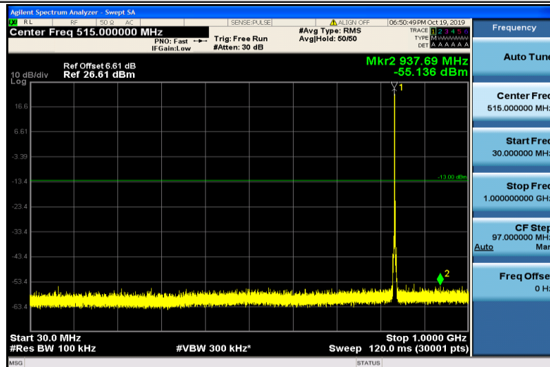
Band5-1.4MHz-16QAM-20525-1RB#0-30~1000MHz
