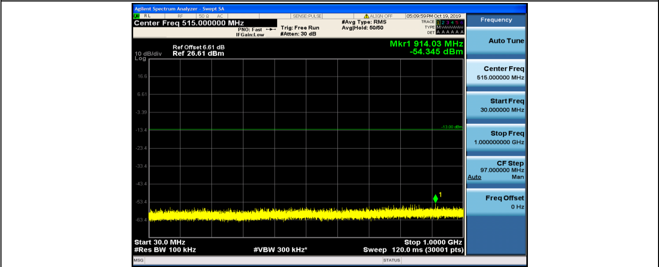
Band4-15MHz-16QAM-20325-1RB#0-30~1000MHz
