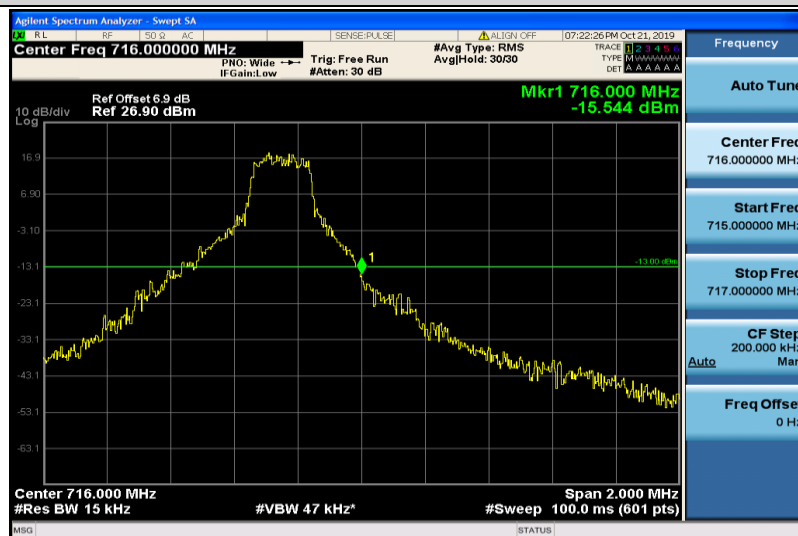
Band12-1.4MHz-QPSK-23173-1RB#5
