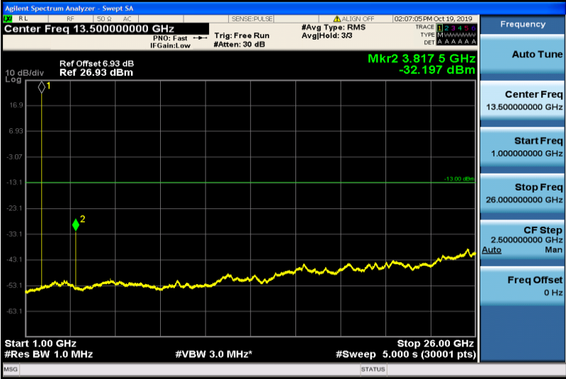
Band2-1.4MHz-QPSK-19193-1RB#0-1000~26000MHz
