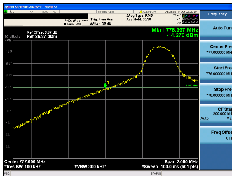
Band13-10MHz-QPSK-23230-1RB#0
