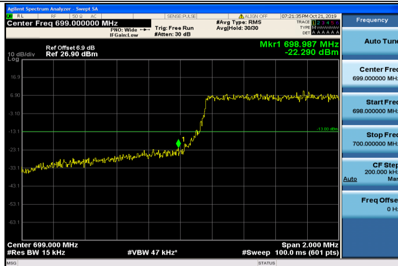
Band12-1.4MHz-16QAM-23017-6RB#0
