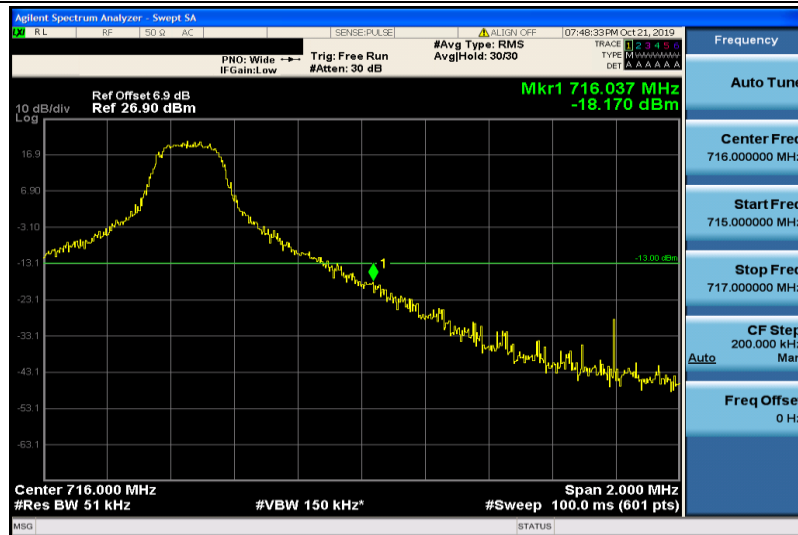
Band12-5MHz-QPSK-23155-1RB#24
