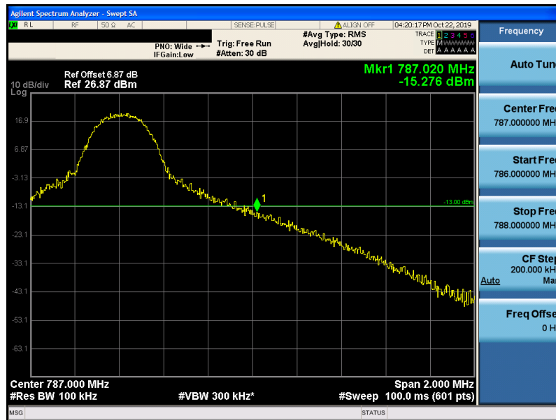
Band13-10MHz-16QAM-23230-1RB#49
