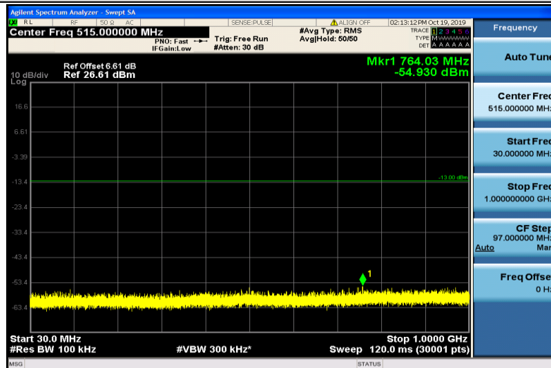
Band2-3MHz-16QAM-18900-1RB#0-30~1000MHz
