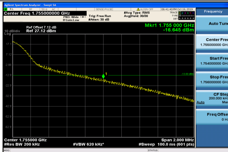
Band4-20MHz-16QAM-20300-1RB#99
