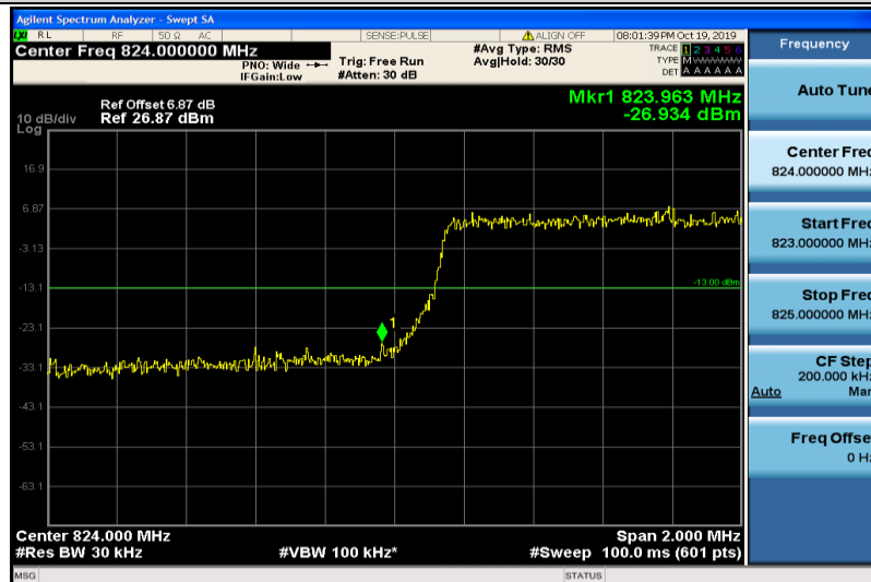
Band5-3MHz-16QAM-20415-15RB#0
