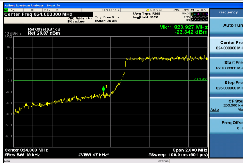
Band5-1.4MHz-QPSK-20407-6RB#0
