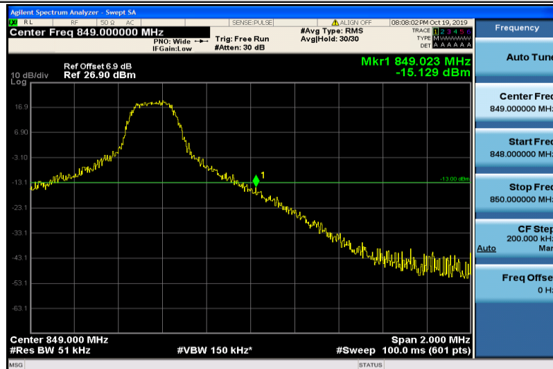
Band5-5MHz-16QAM-20625-1RB#24
