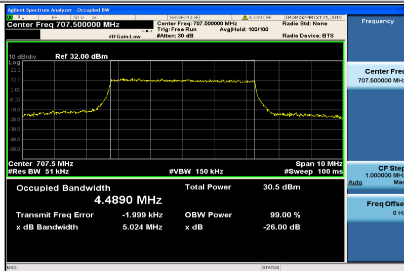
Band12-5MHz-16QAM-23095-25RB#0-4.4890
