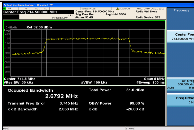
Band12-3MHz-QPSK-23165-15RB#0-2.6792
