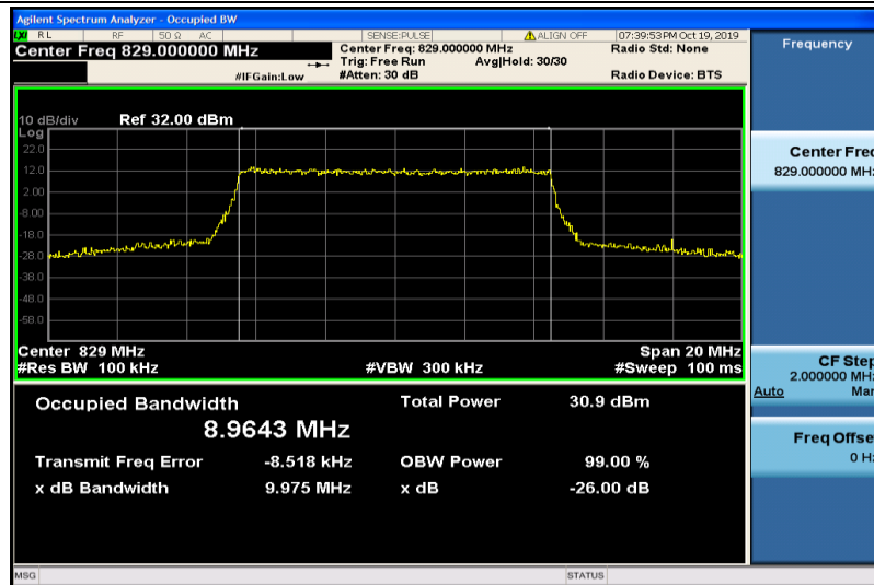
Band5-10MHz-QPSK-20450-50RB#0-8.9643
