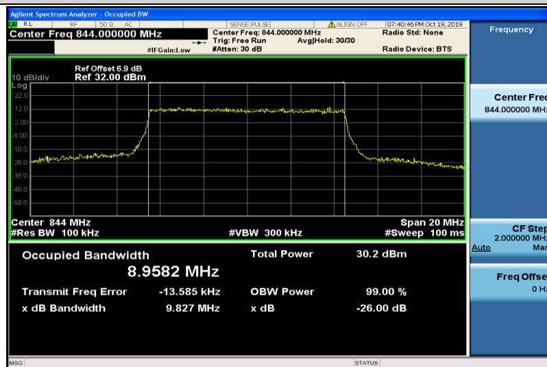
Band5-10MHz-16QAM-20600-50RB#0-8.9582
