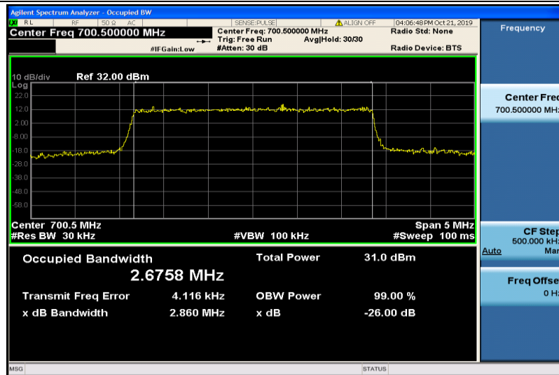
Band12-3MHz-QPSK-23025-15RB#0-2.6758
