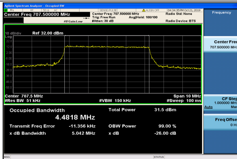
Band12-5MHz-QPSK-23095-25RB#0-4.4818
