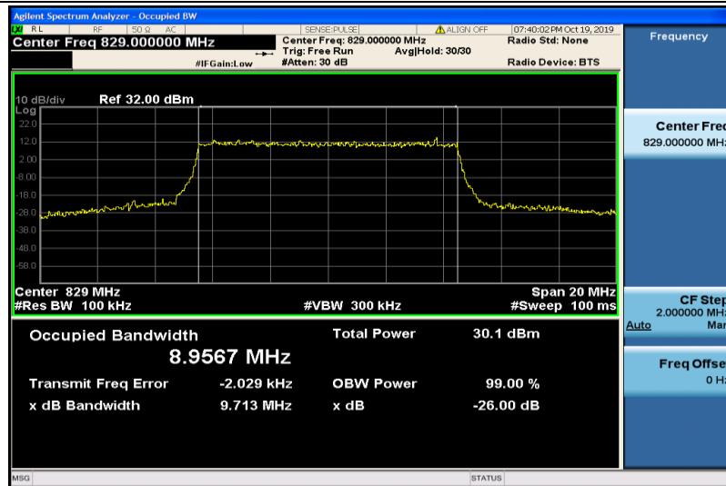
Band5-10MHz-16QAM-20450-50RB#0-8.9567
