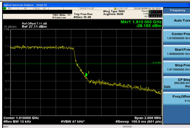
Band2-1.4MHz-16QAM-1913-6RB#0
