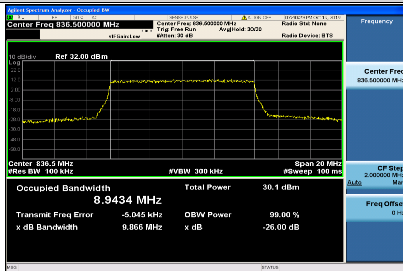
Band5-10MHz-16QAM-20525-50RB#0-8.9434
