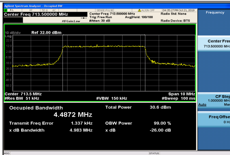
Band12-5MHz-16QAM-23155-25RB#0-4.4872
