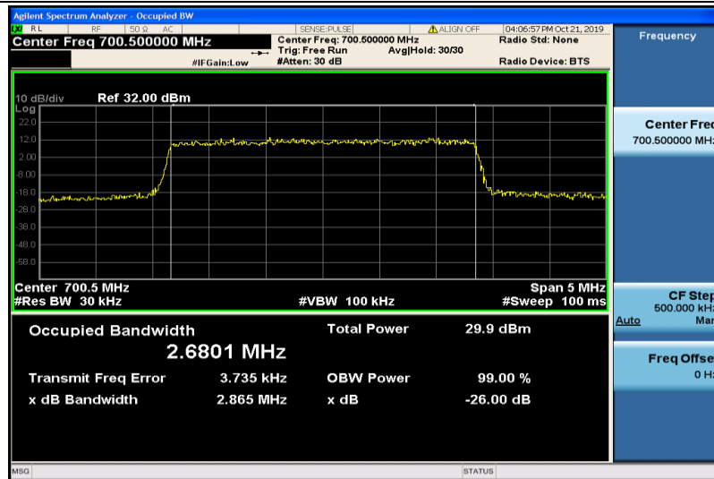
Band12-3MHz-16QAM-23025-15RB#0-2.6801
