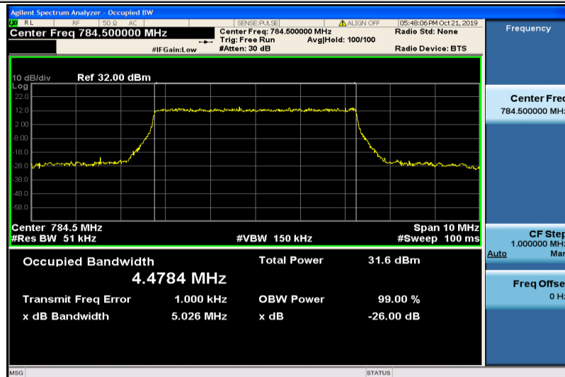
Band13-5MHz-QPSK-23255-25RB#0-4.4784
