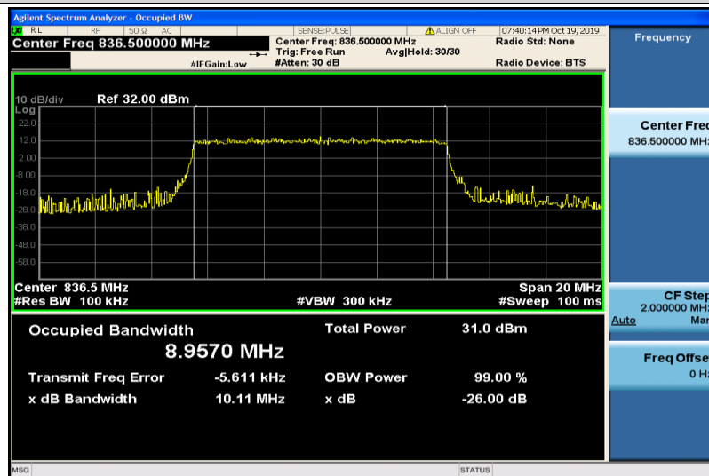
Band5-10MHz-QPSK-20525-50RB#0-8.9570
