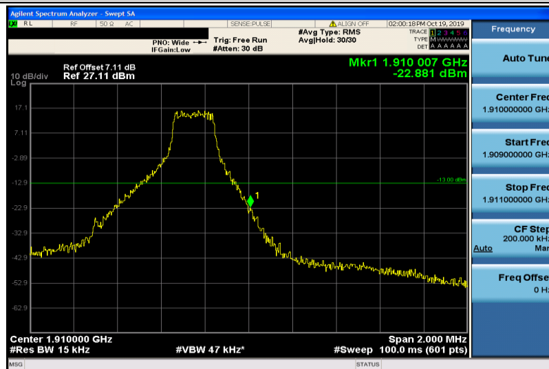
Band2-1.4MHz-16QAM-1913-1RB#5
