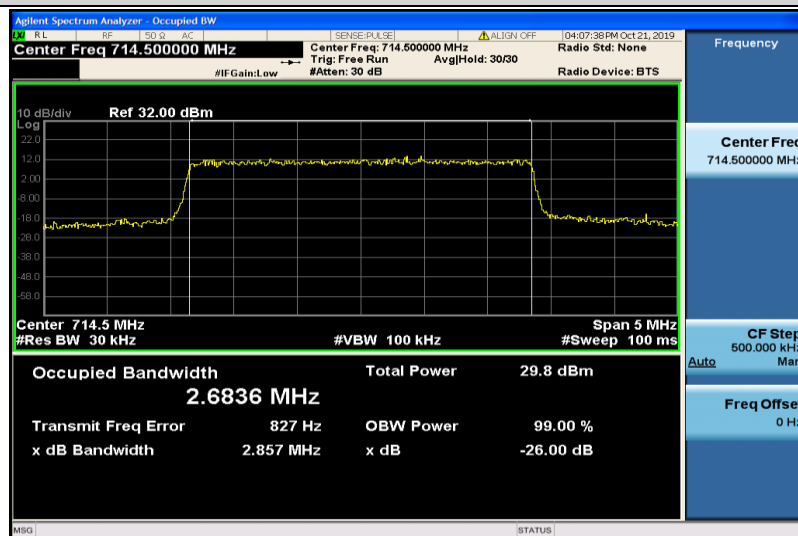
Band12-3MHz-16QAM-23165-15RB#0-2.6836
