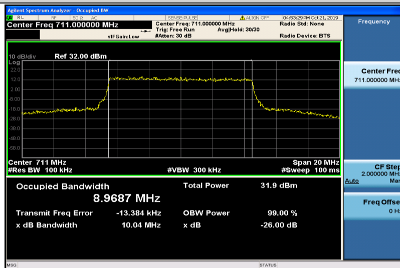
Band12-10MHz-QPSK-23130-50RB#0-8.9687
