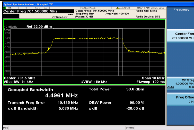
Band12-5MHz-16QAM-23035-25RB#0-4.4961
