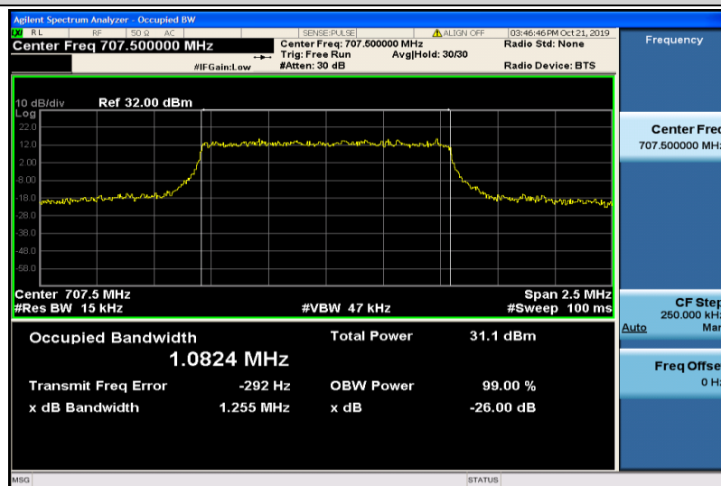
Band12-1.4MHz-QPSK-23095-6RB#0-1.0824
