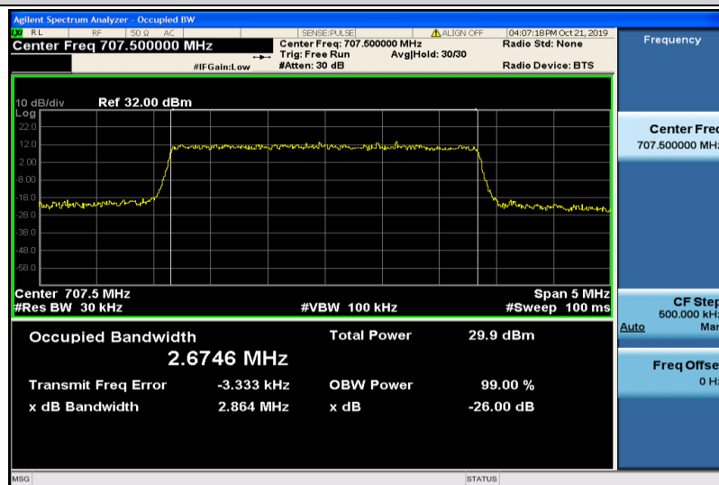
Band12-3MHz-16QAM-23095-15RB#0-2.6746
