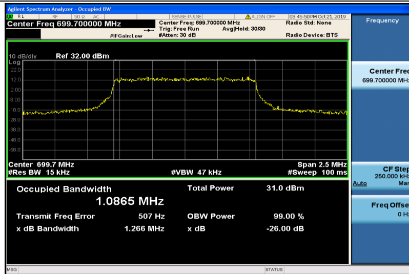
Band12-1.4MHz-QPSK-23017-6RB#0-1.0865
