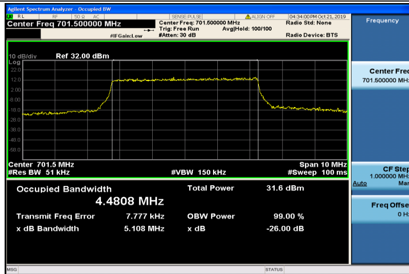
Band12-5MHz-QPSK-23035-25RB#0-4.4808
