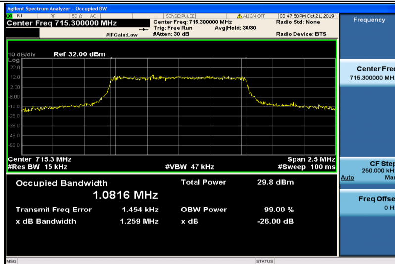
Band12-1.4MHz-16QAM-23173-6RB#0-1.0816
