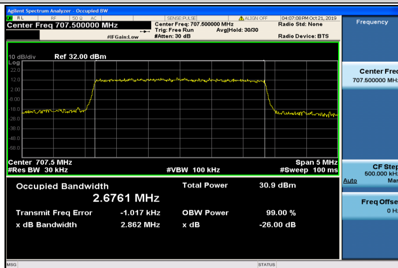
Band12-3MHz-QPSK-23095-15RB#0-2.6761
