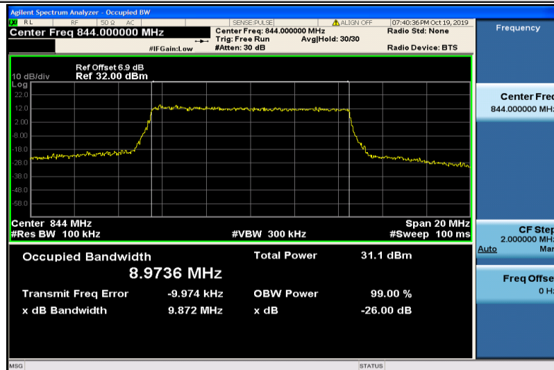
Band5-10MHz-QPSK-20600-50RB#0-8.9736
