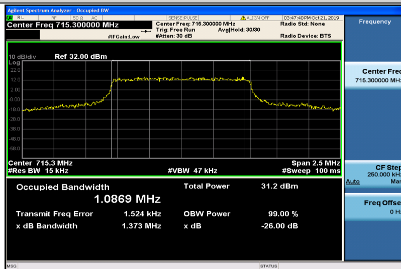
Band12-1.4MHz-QPSK-23173-6RB#0-1.0869
