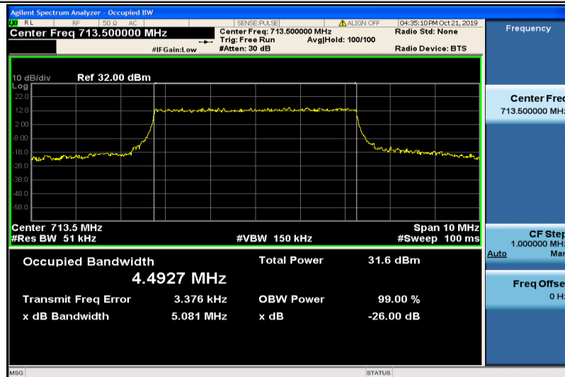
Band12-5MHz-QPSK-23155-25RB#0-4.4927
