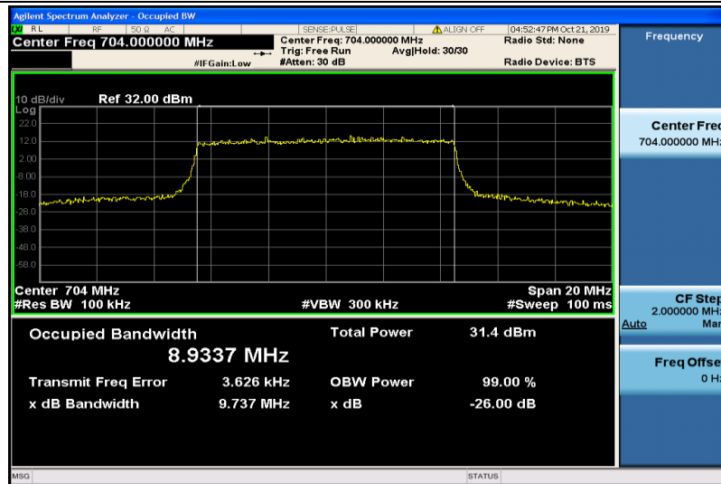
Band12-10MHz-QPSK-23060-50RB#0-8.9337
