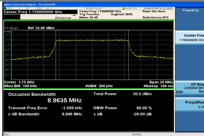
Band4-10MHz-QPSK-20350-50RB#0-8.9635
