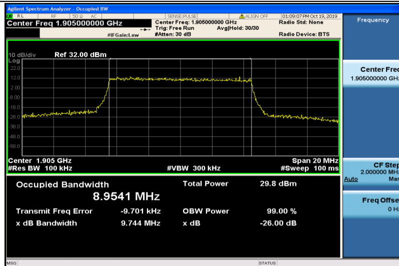
Band2-10MHz-16QAM-19150-50RB#0-8.9541
