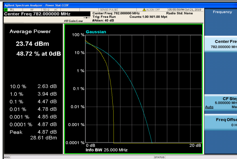
Band13-5MHz-QPSK-23230-1RB#0
