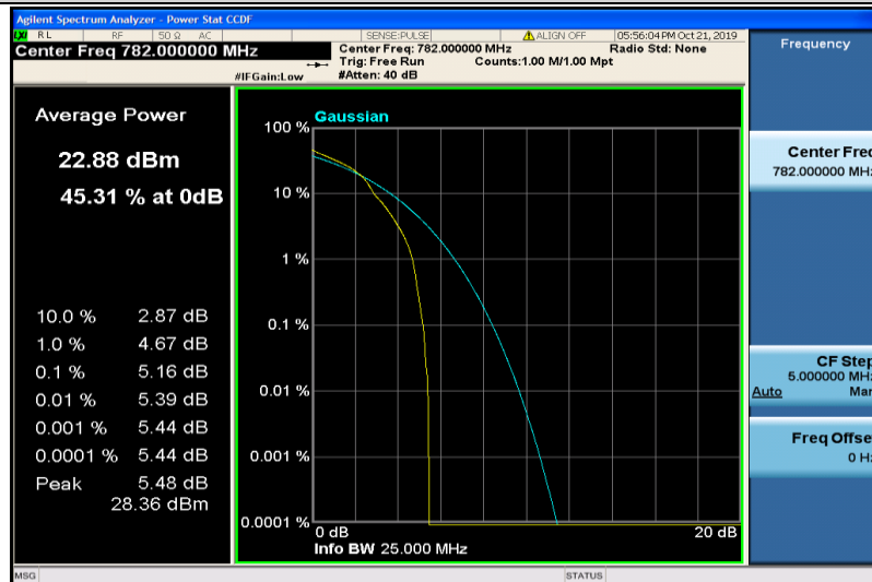
Band13-5MHz-16QAM-23230-1RB#0
