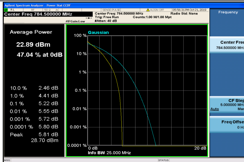
Band13-5MHz-QPSK-23255-25RB#0
