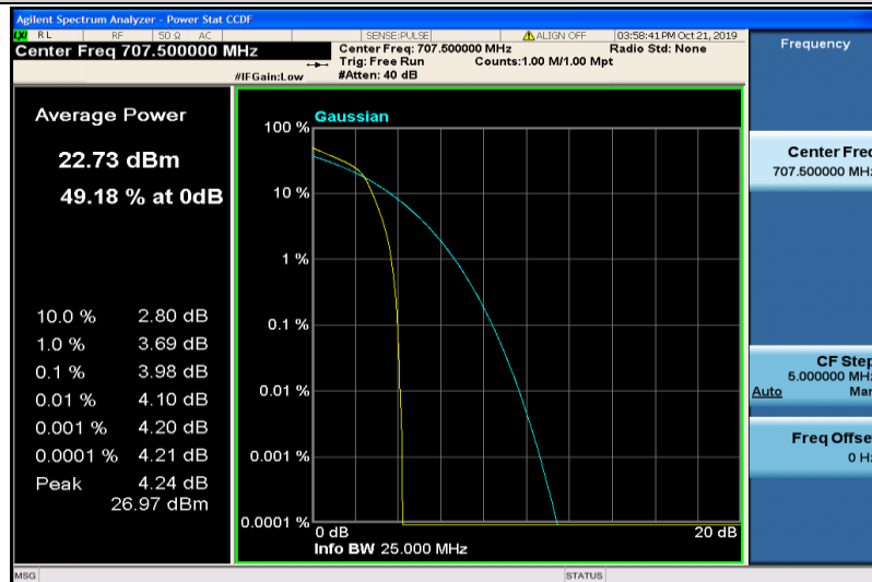
Band12-1.4MHz-16QAM-23095-1RB#0
