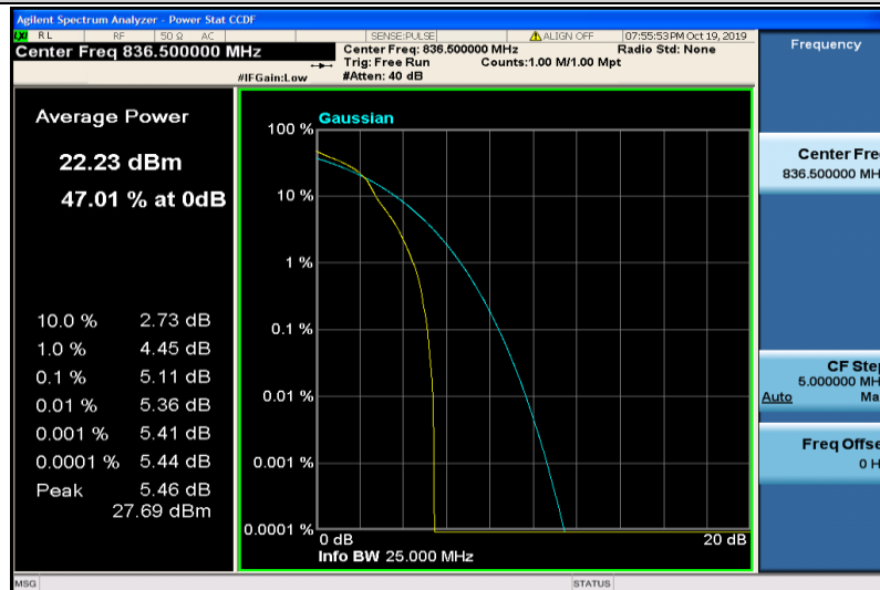
Band5-10MHz-16QAM-20525-1RB#0
