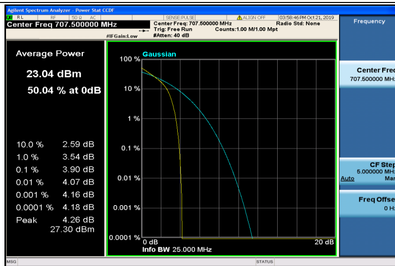
Band12-1.4MHz-QPSK-23095-6RB#0
