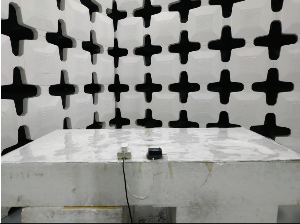
Radiated emission Test Setup (back side)
