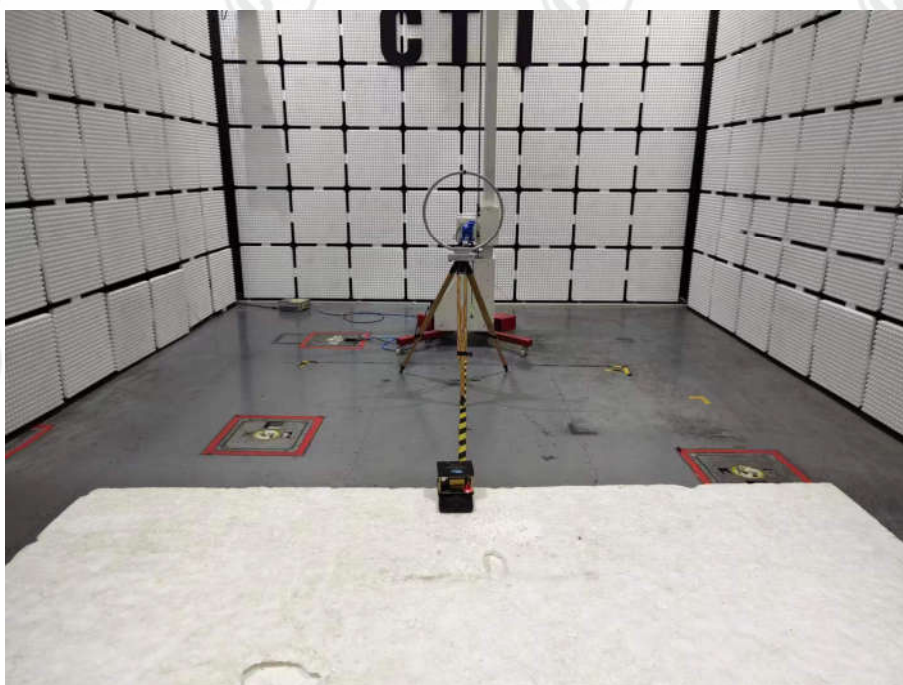
Radiated Emissions Test Setup (9kHz-30MHz) Mode b to Mode e
