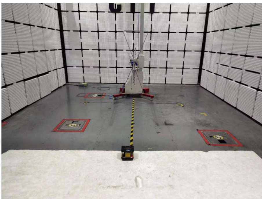
Radiated Emissions Test Setup (30MHz-1GHz)Mode b to Mode e
