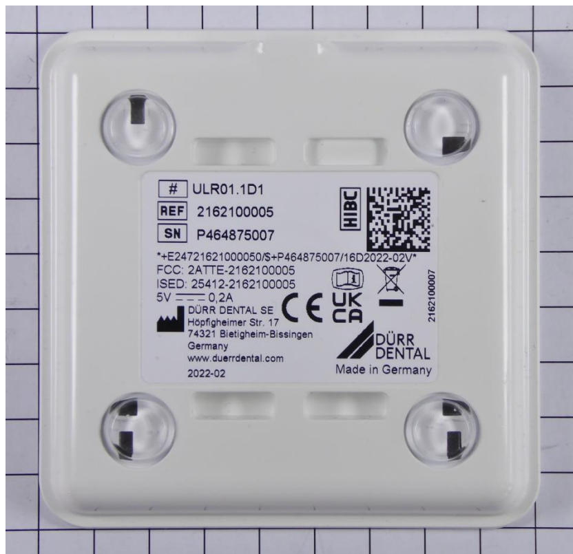
Bottom view
