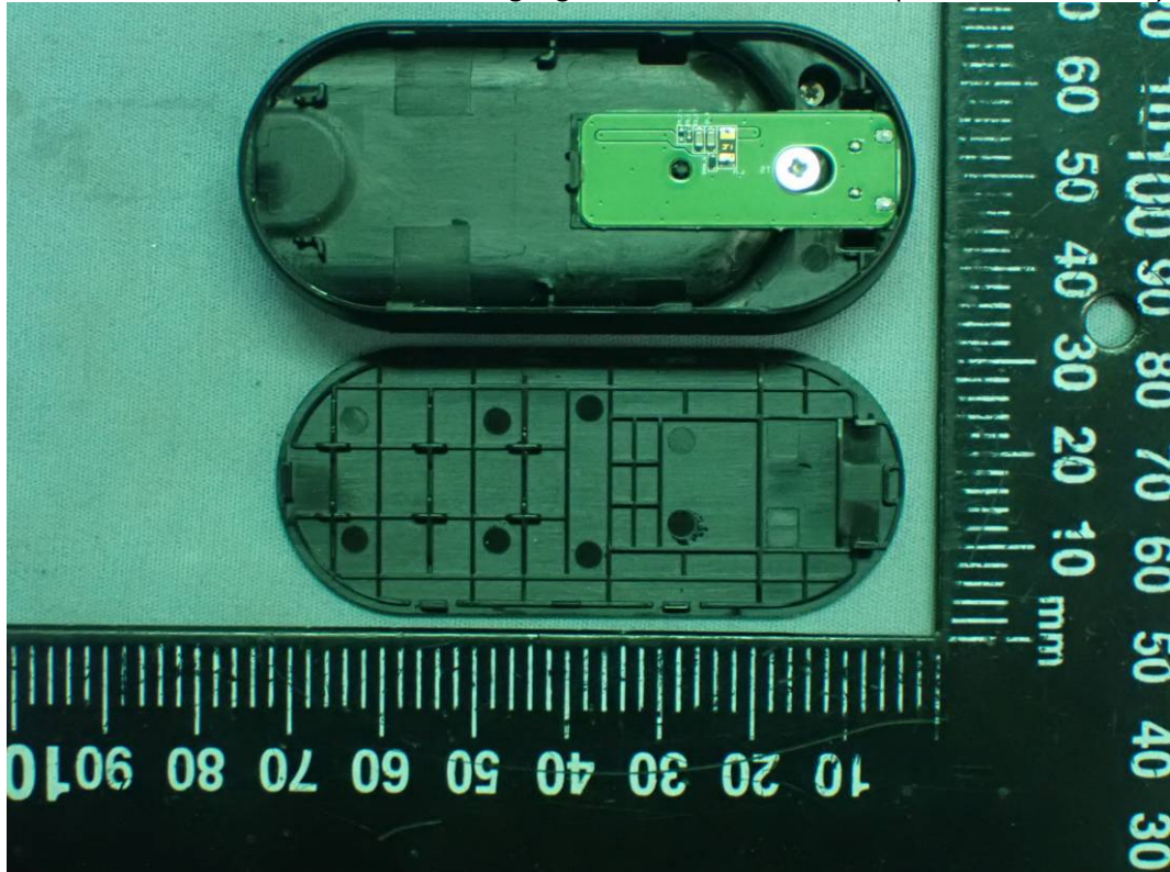
Figure 30 Charging dock, Internal View (Removed Cover)
