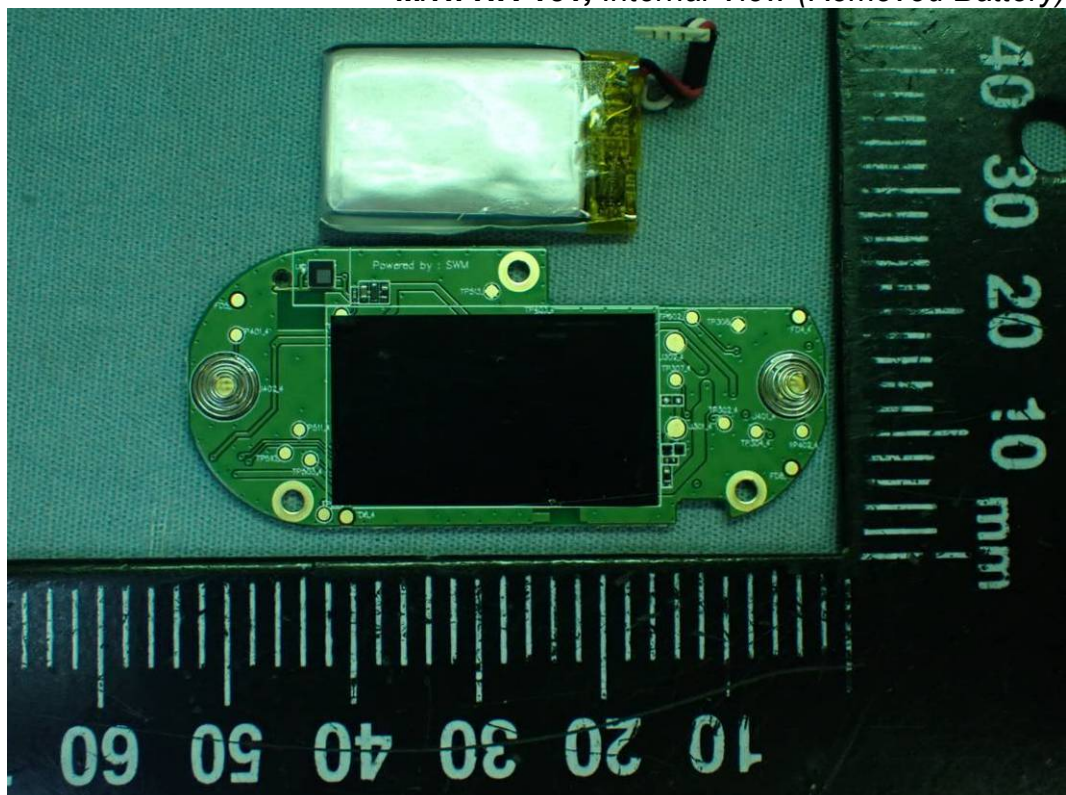
Figure 35 M/N: HR-131, Internal View (Removed Battery)
