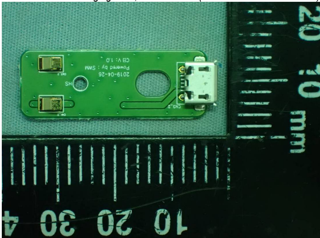
Figure 31 Charging dock, Internal View (Internal Board / Front View)
