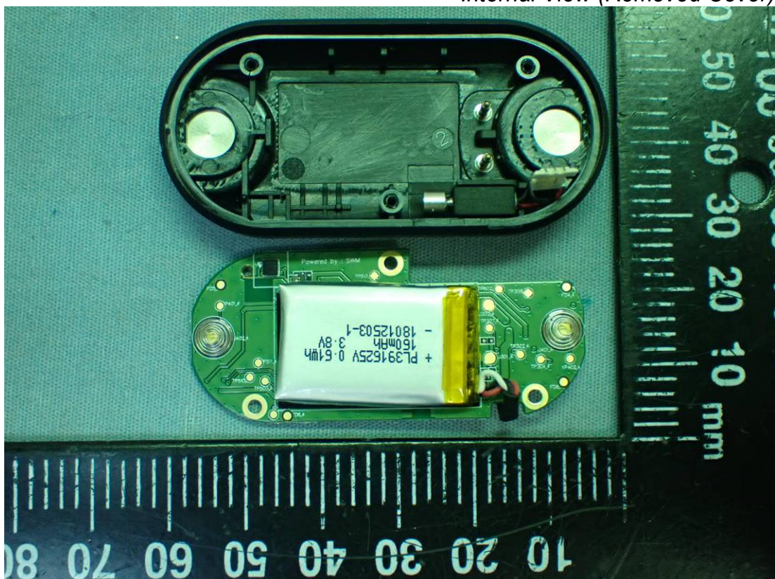
Figure 33 Internal View (Removed Cover)
