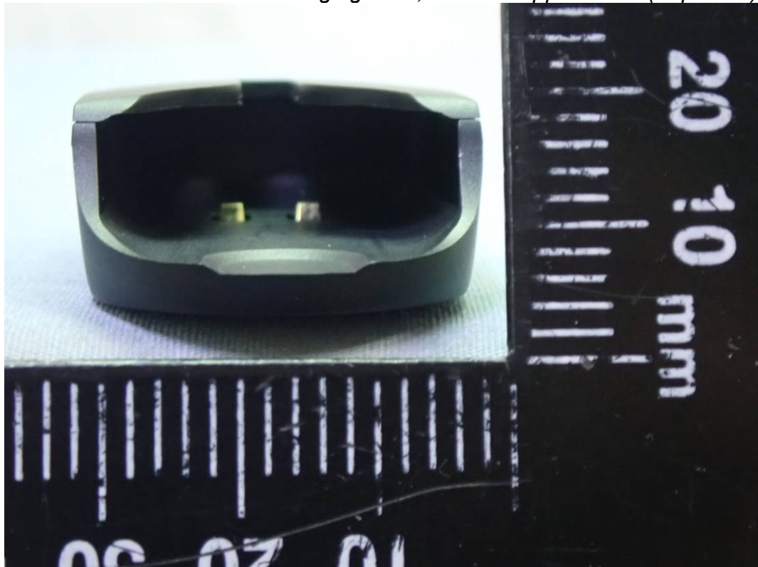
Figure 5 Black Charging dock, General Appearance (Top View)
