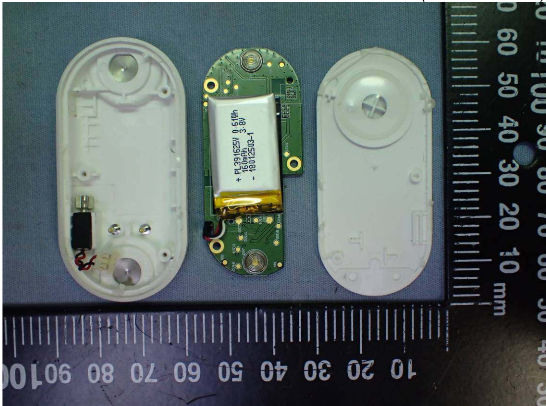
Figure 32 Internal View (Removed Cover)
