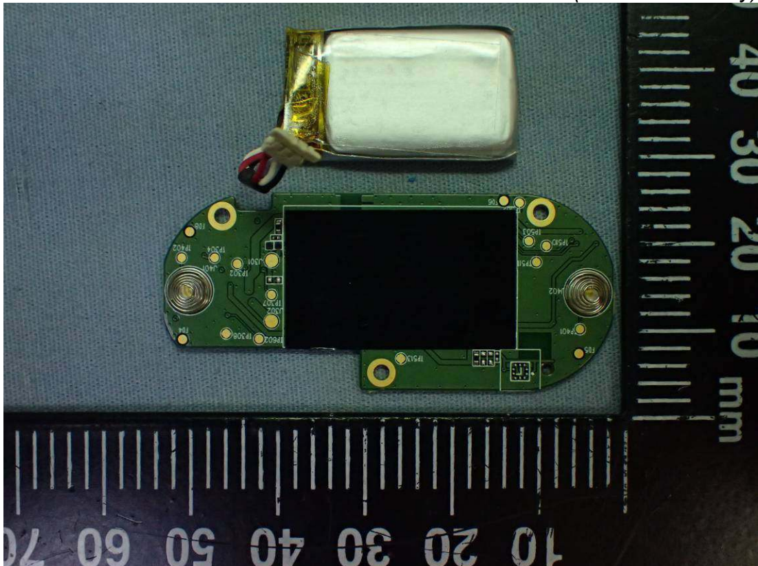
Figure 36 Internal View (Removed Battery)
