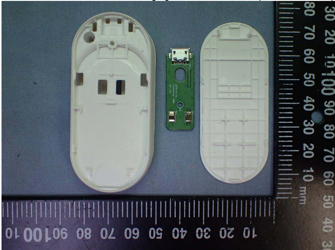
Figure 29 Charging dock, Internal View (Removed Cover)
