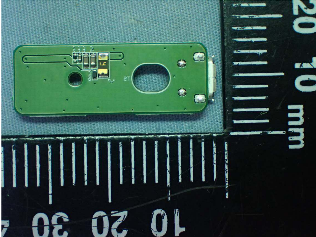
Figure 31 Charging dock, Internal View (Internal Board / Back View)
