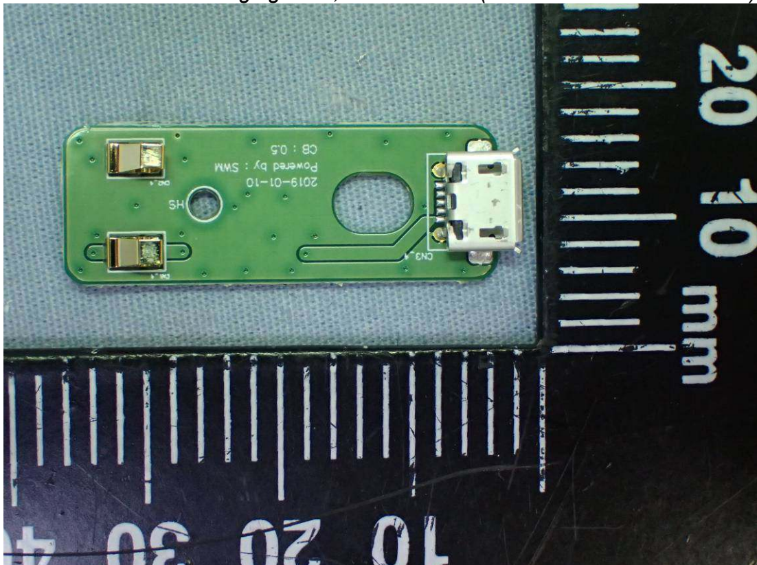
Figure 30 Charging dock, Internal View (Internal Board / Front View)
