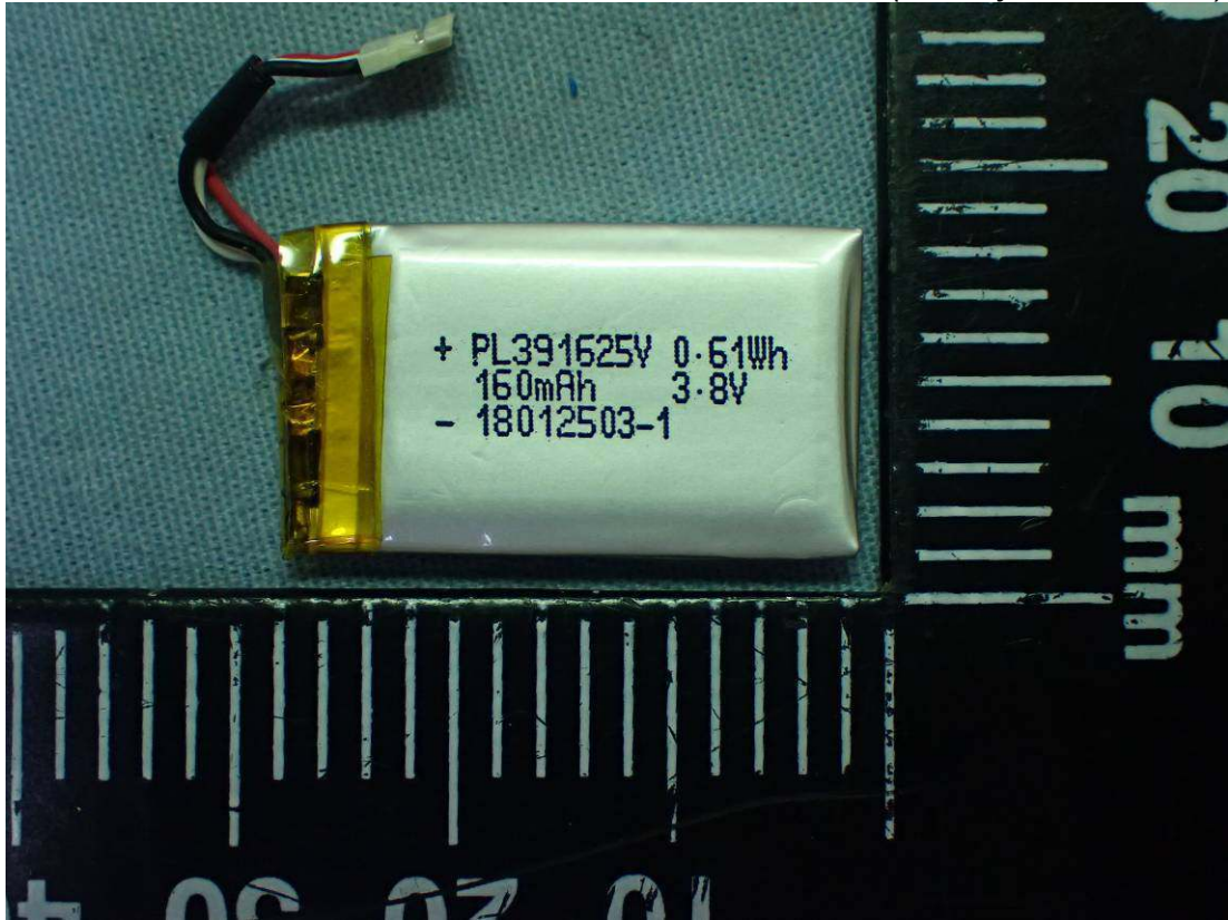
Figure 37 Internal View (Battery / Front View)
