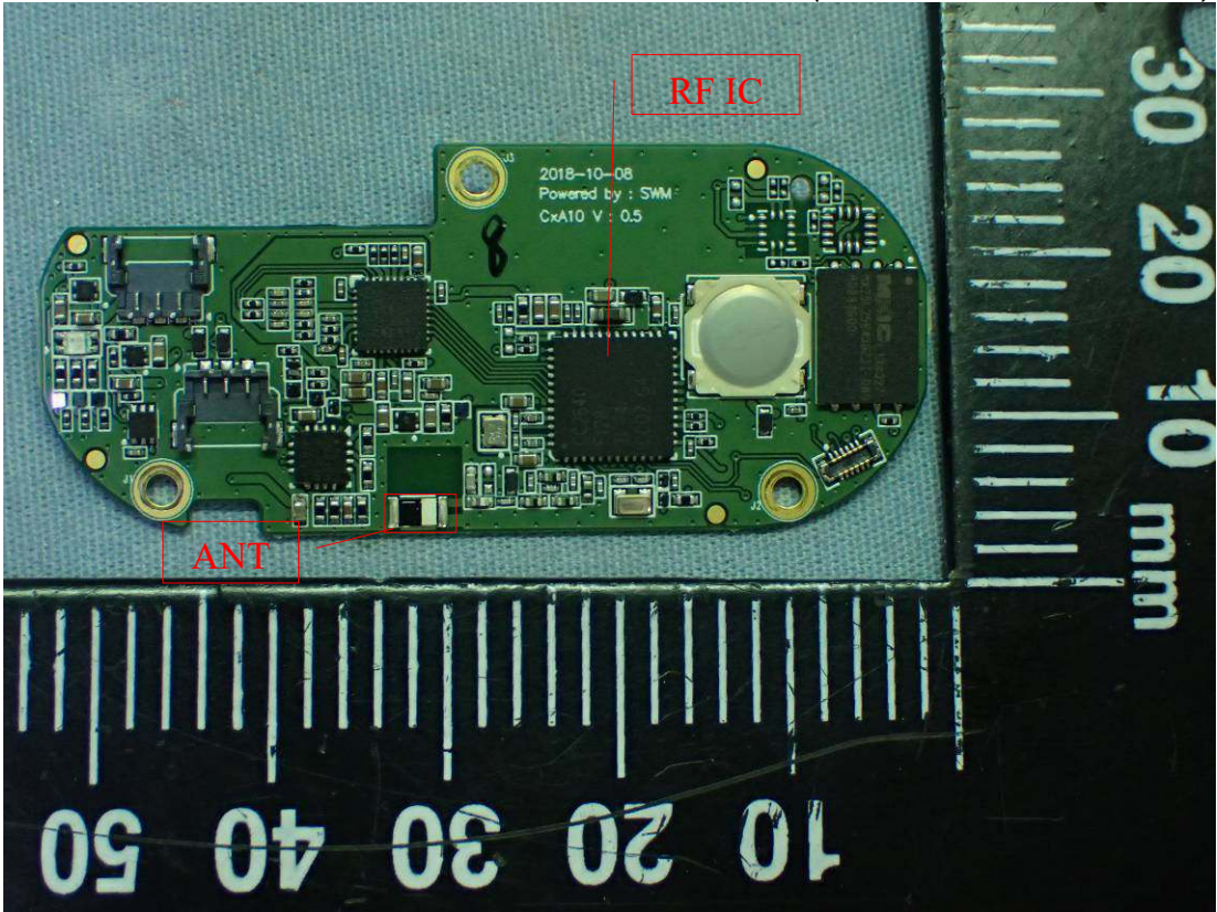
Figure 33 Internal View (Main Board / Front View)
