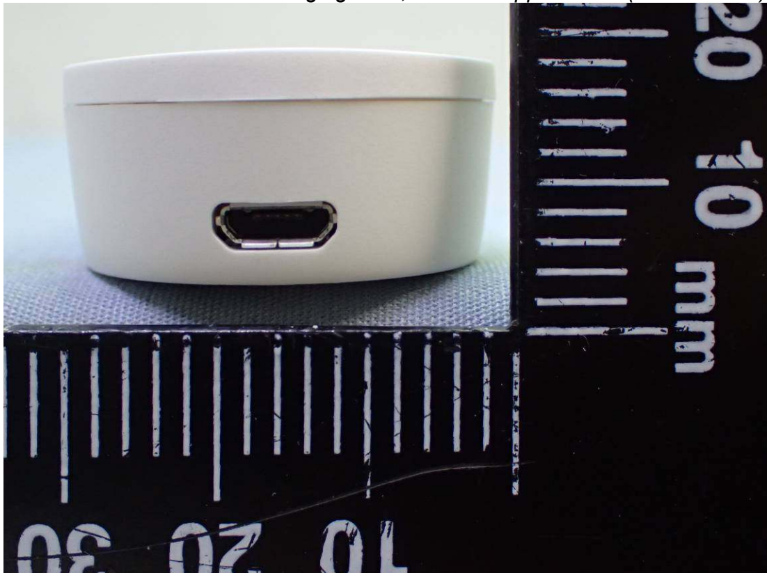
Figure 6 Charging dock, General Appearance (Bottom View)
