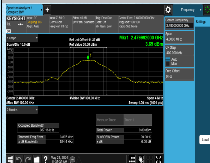
GFSK-Ant3-2480-PASS
