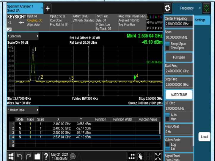
GFSK-Ant3-2480-PASS
