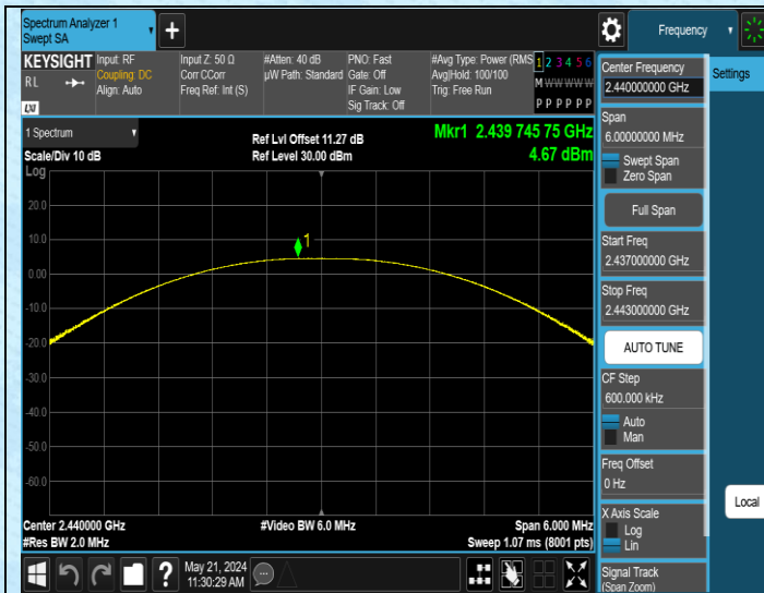
GFSK-Ant2-2440-PASS
