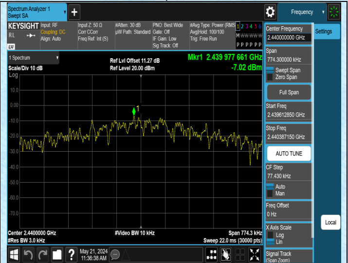
GFSK-Ant3-2440-PASS
