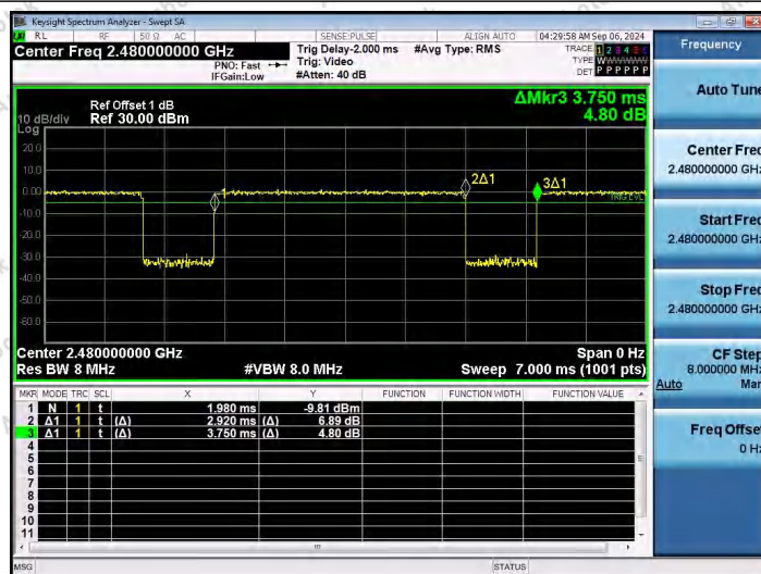
NTVN-3DH5-Ant1-2480
