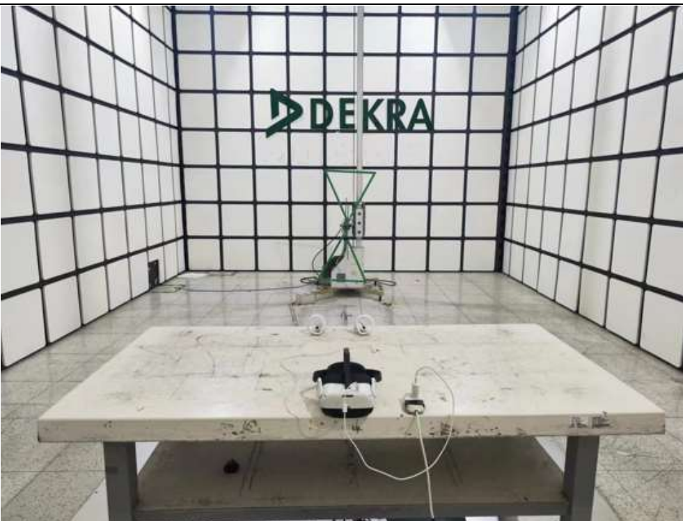
Description: Rear View of Radiated Disturbance Test Setup (Below 1 GHz)
