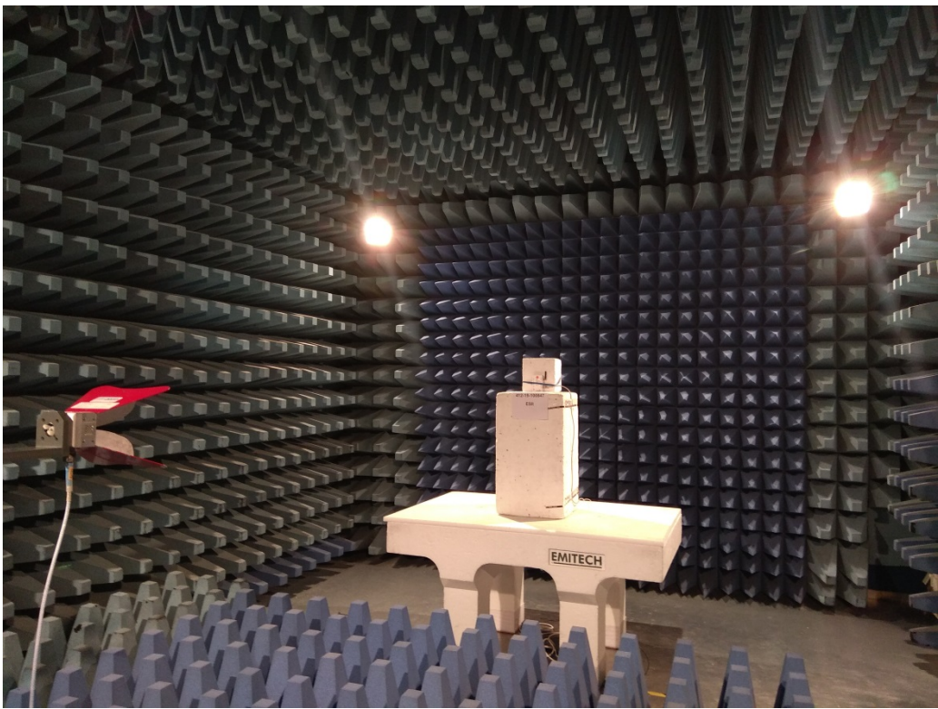
TEST SETUP PHOTO(S) - SPURIOUS – > 1GHZ
