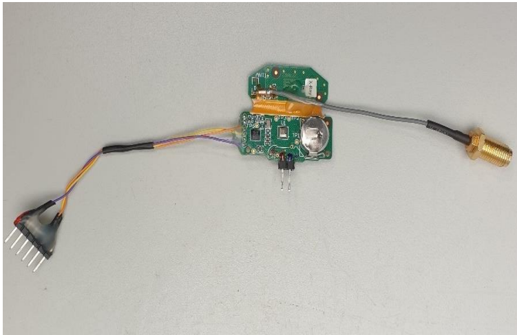
Photo 4. Printed circuit board (top side) with temporary antenna connector.
