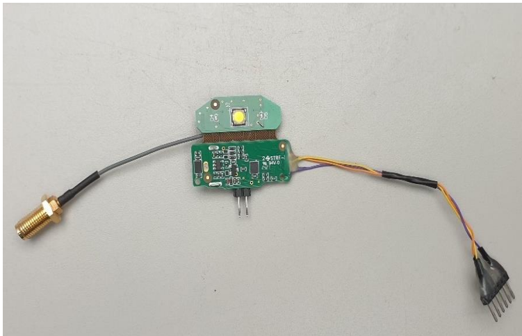
Photo 5. Printed circuit board (bottom side) with temporary antenna connector.
