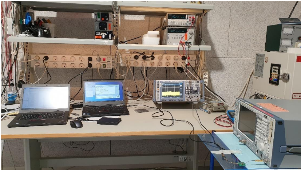
Photo 7. Conducted measurements test set up.
