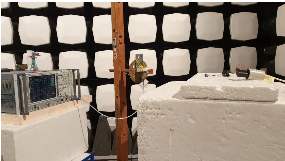
Photo 10. Radiated emission test setup for 13.5 – 25 GHz.
