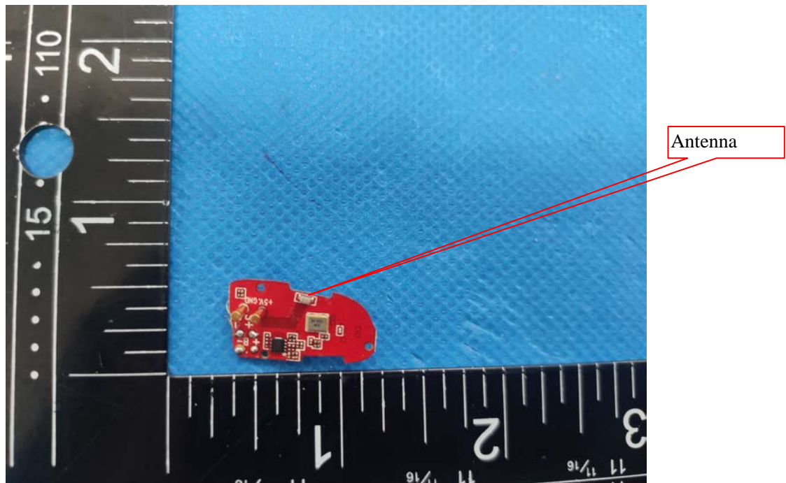
EUT Housing and Board View 7 (Left )
