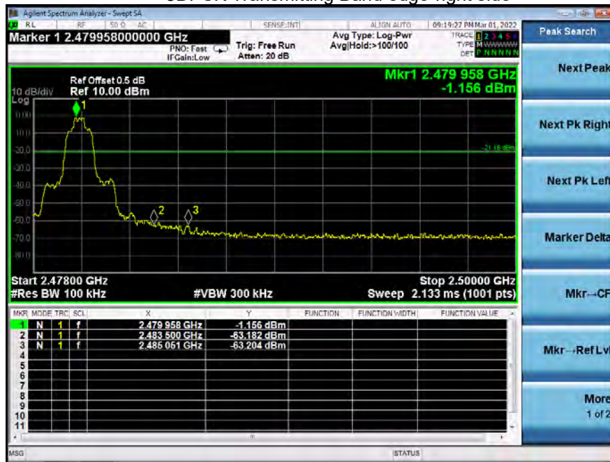
8DPSK Transmitting Band edge-right side
