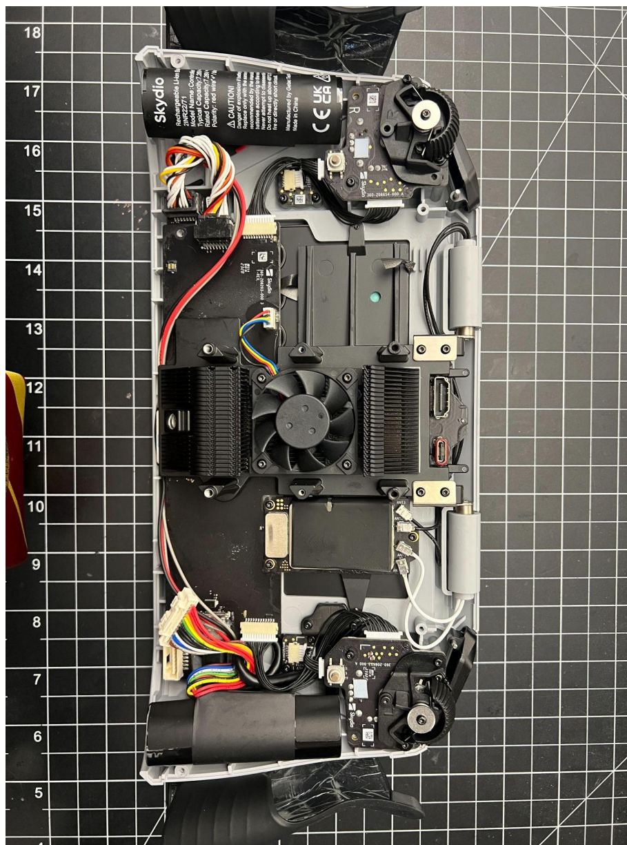
Photo 1: Main Assembly with RF Module
