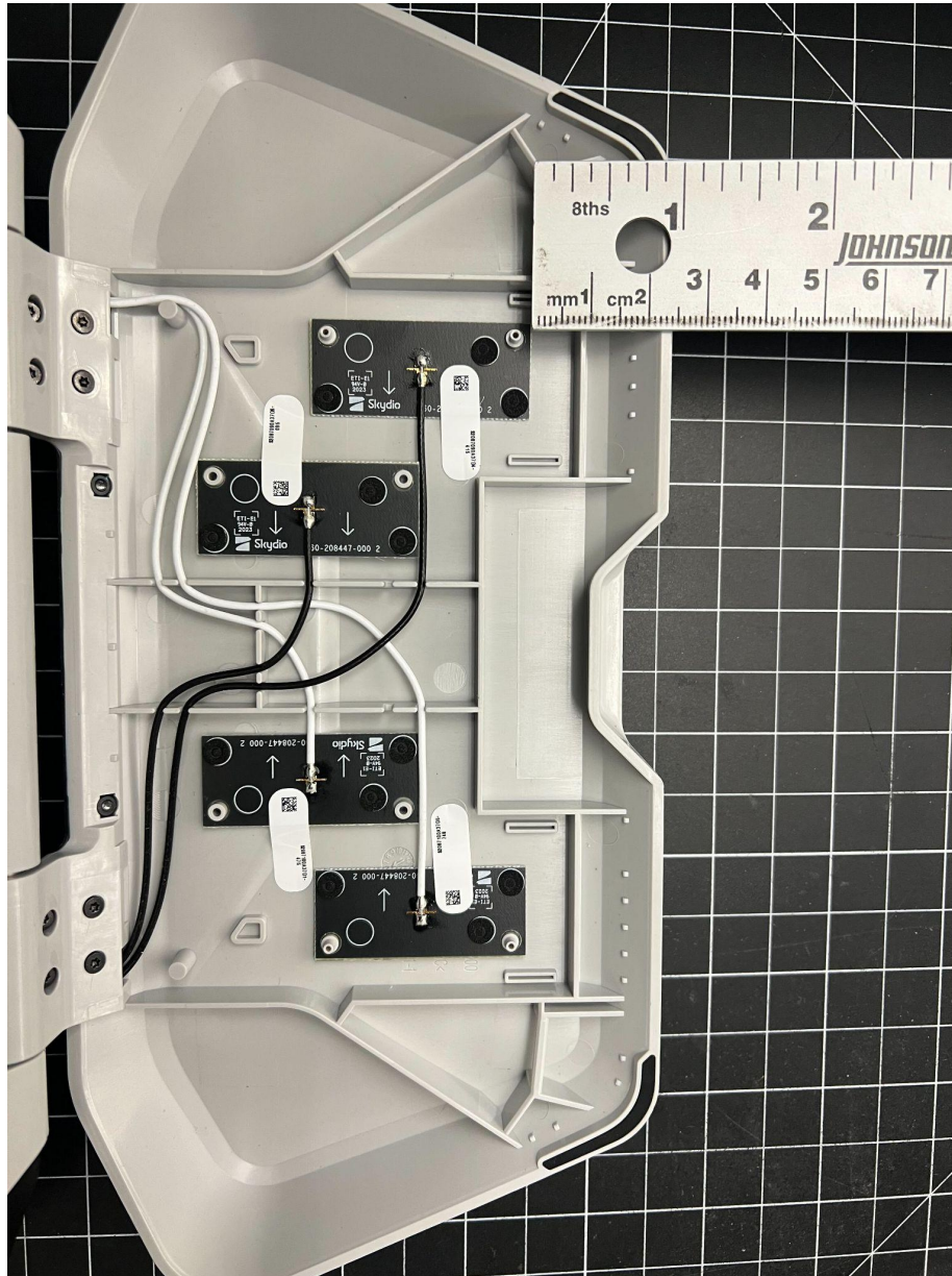
Photo 2: Top Cover with Antennas
