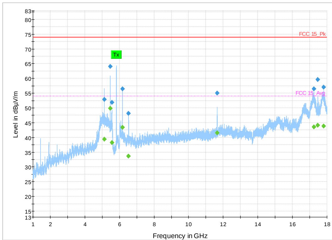
Figure 14: 1-18 GHz 802.11a Mode 10 MHz, High Channel
