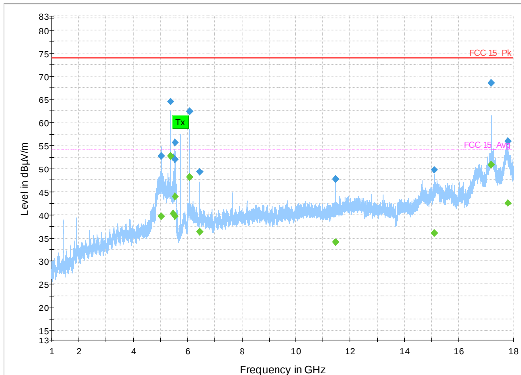
Figure 22: 1-18 GHz 802.11n HT Mode 5 MHz, Low Channel
