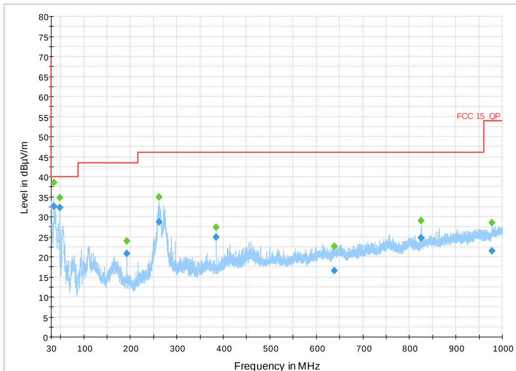
Figure 21: 30 MHz-1 GHz 802.11n HT Mode 5 MHz, Mid Channel
