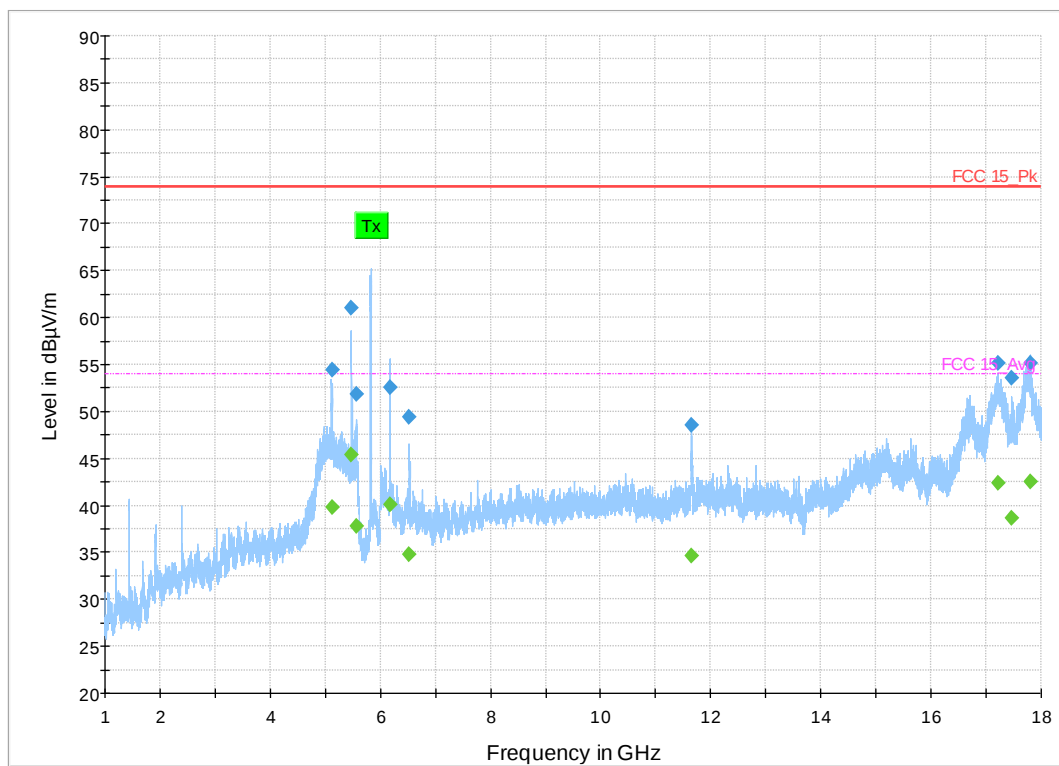
Figure 43: 1-18 GHz 802.11ac VHT Mode 20 MHz, High Channel
