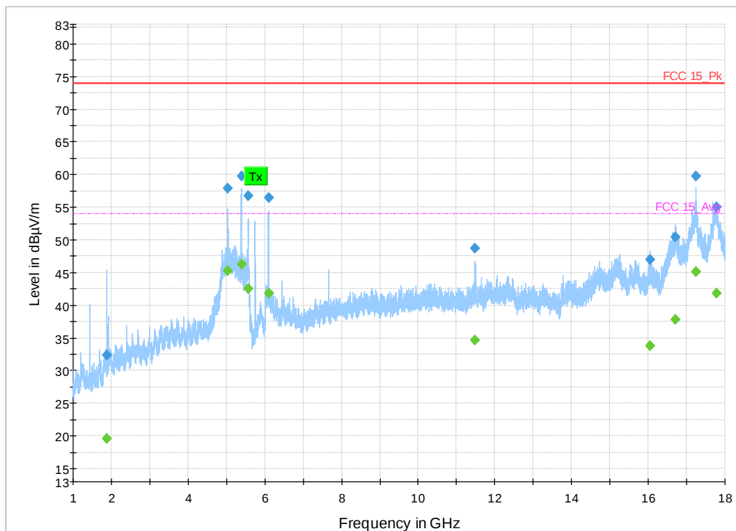
Figure 32: 1-18 GHz 802.11n HT Mode 20 MHz, Low Channel
