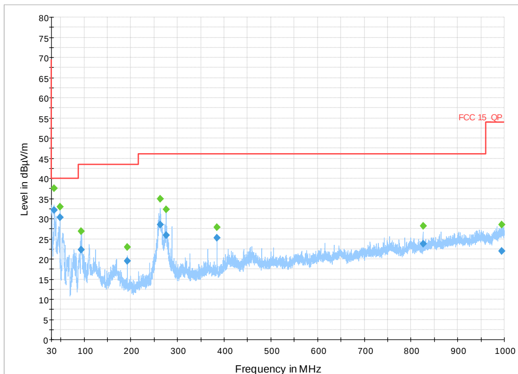
Figure 31: 30 MHz-1 GHz 802.11n HT Mode 20 MHz, Mid Channel
