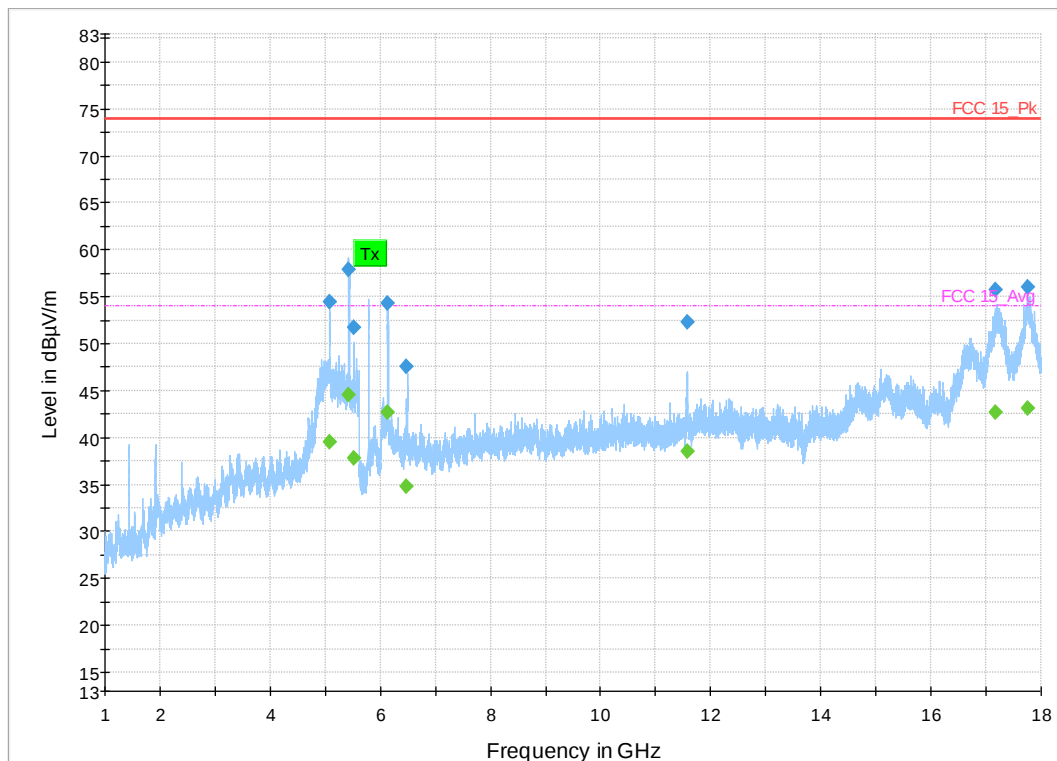
Figure 18: 1-18 GHz 802.11a Mode 20 MHz, Mid Channel
