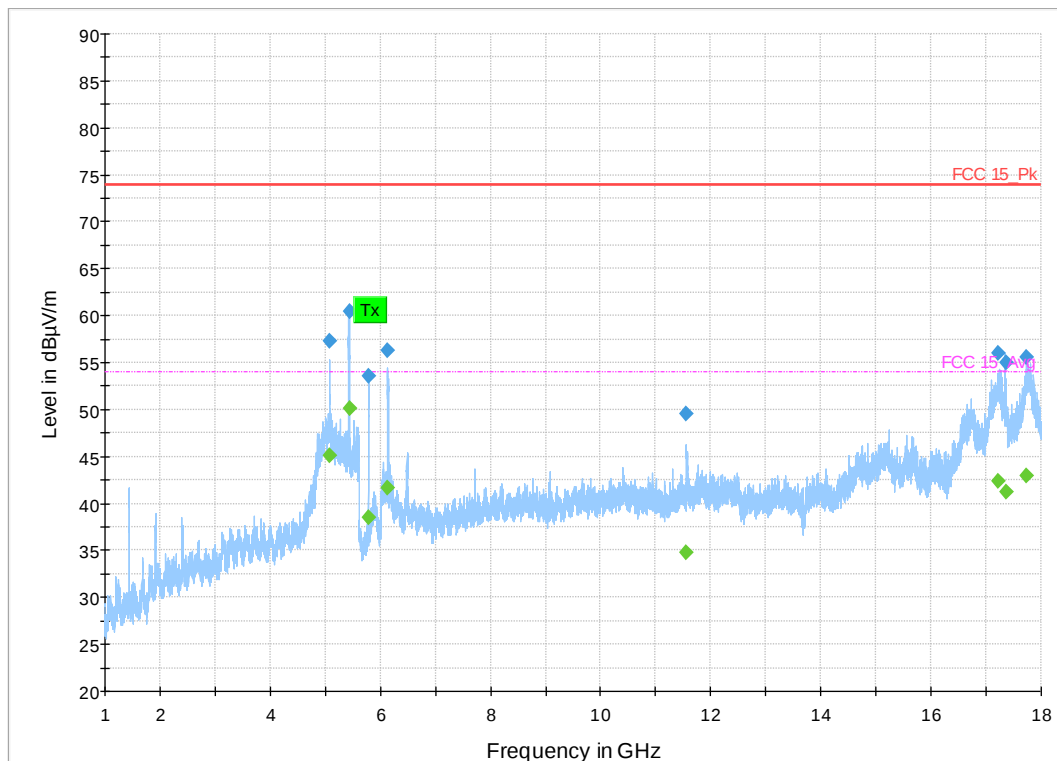
Figure 42: 1-18 GHz 802.11ac VHT Mode 20 MHz, Mid Channel
