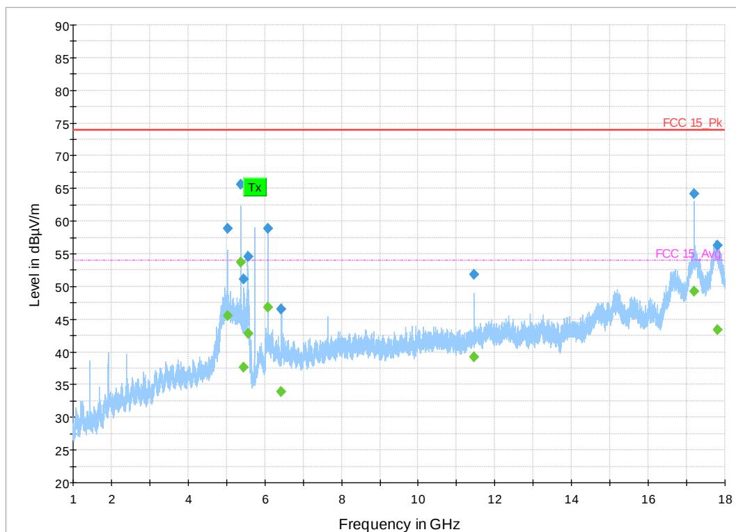
Figure 7: 1-18 GHz 802.11a Mode 5 MHz, Low Channel
