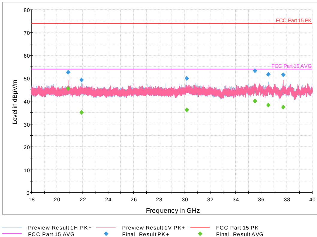
Figure 39: 18-40 GHz 802.11n HT Mode 40 MHz, Low Channel
