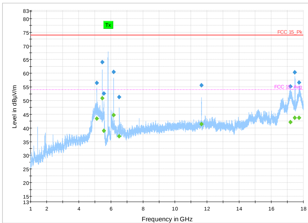
Figure 29: 1-18 GHz 802.11n HT Mode 10 MHz, High Channel
