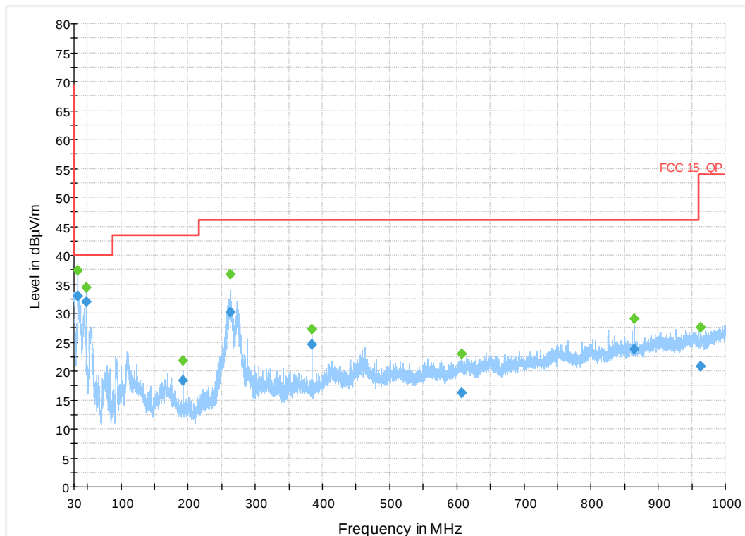
Figure 26: 30 MHz-1 GHz 802.11n HT Mode 10 MHz, Mid Channel
