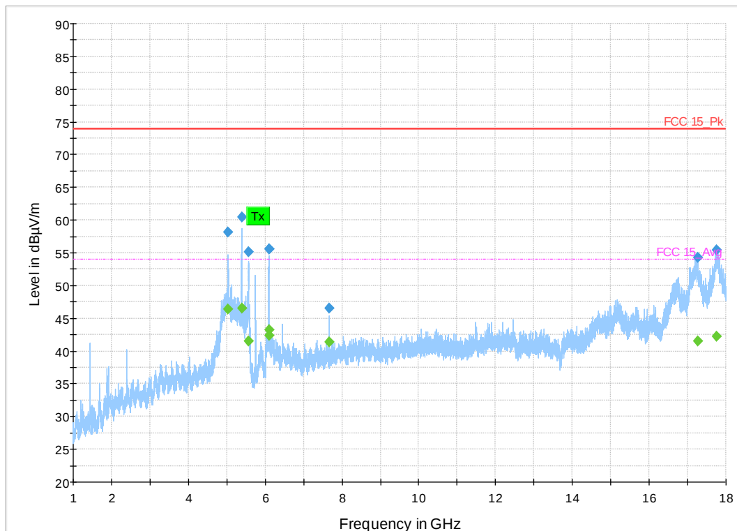
Figure 41: 1-18 GHz 802.11ac VHT Mode 20 MHz, Low Channel
