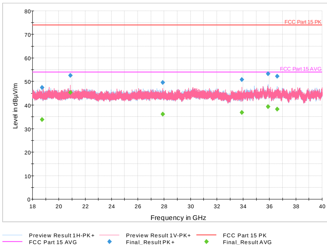
Figure 44: 18-40 GHz 802.11ac VHT Mode 20 MHz, Mid Channel
