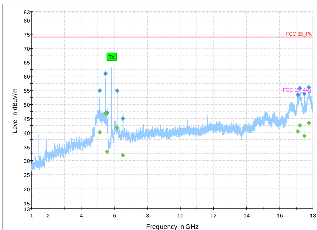
Figure 19: 1-18 GHz 802.11a Mode 20 MHz, High Channel
