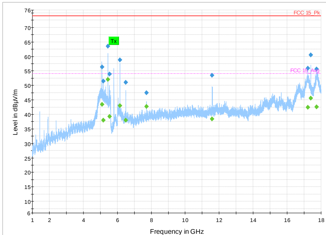
Figure 28: 1-18 GHz 802.11n HT Mode 10 MHz, Mid Channel
