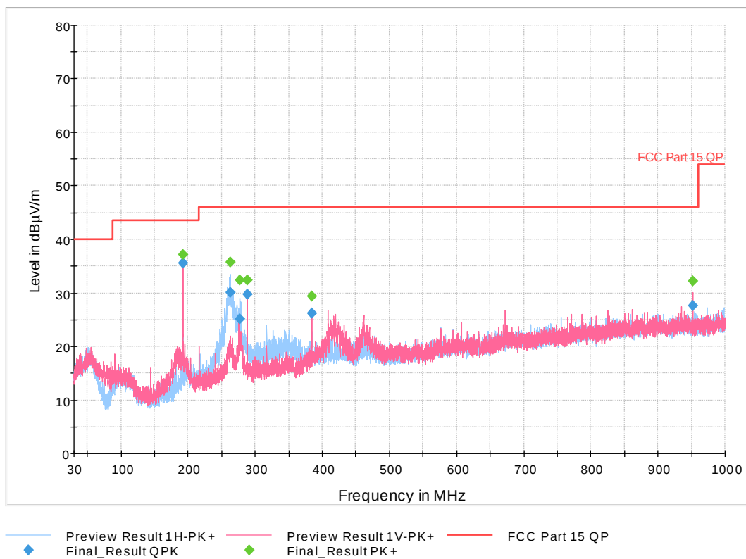
Figure 40: 30 MHz-1 GHz 802.11ac VHT Mode 20 MHz, Mid Channel
