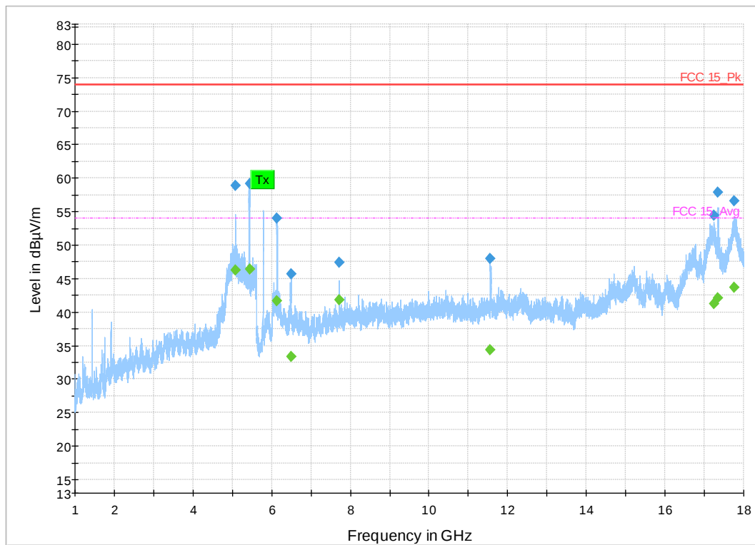
Figure 33: 1-18 GHz 802.11n HT Mode 20 MHz, Mid Channel
