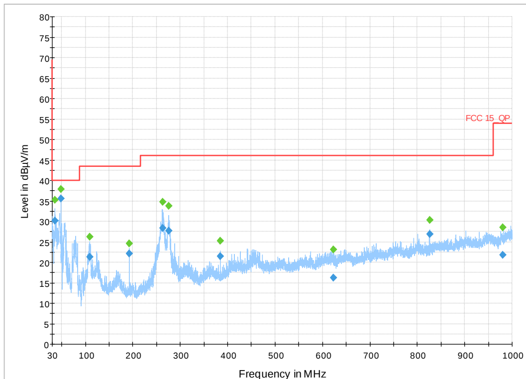
Figure 11: 30 MHz-1 GHz 802.11a Mode 10 MHz, Mid Channel
