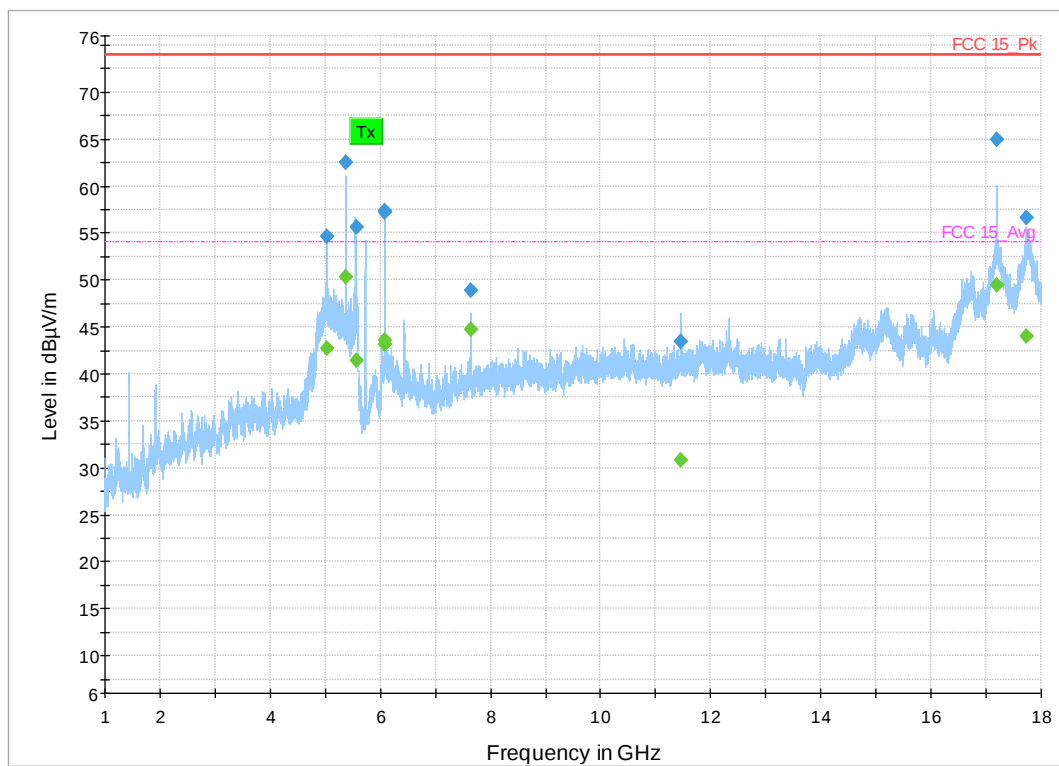
Figure 27: 1-18 GHz 802.11n HT Mode 10 MHz, Low Channel
