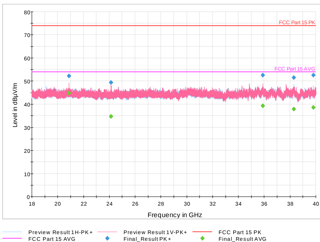
Figure 35: 18-40 GHz 802.11n HT Mode 20 MHz, Mid Channel
