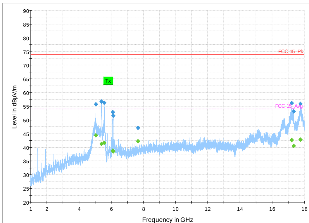
Figure 46: 1-18 GHz 802.11ac VHT Mode 40 MHz, Low Channel
