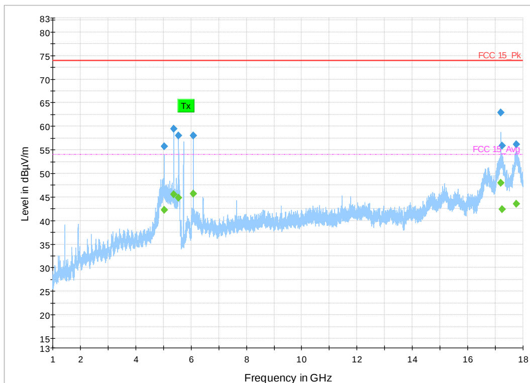
Figure 12: 1-18 GHz 802.11a Mode 10 MHz, Low Channel
