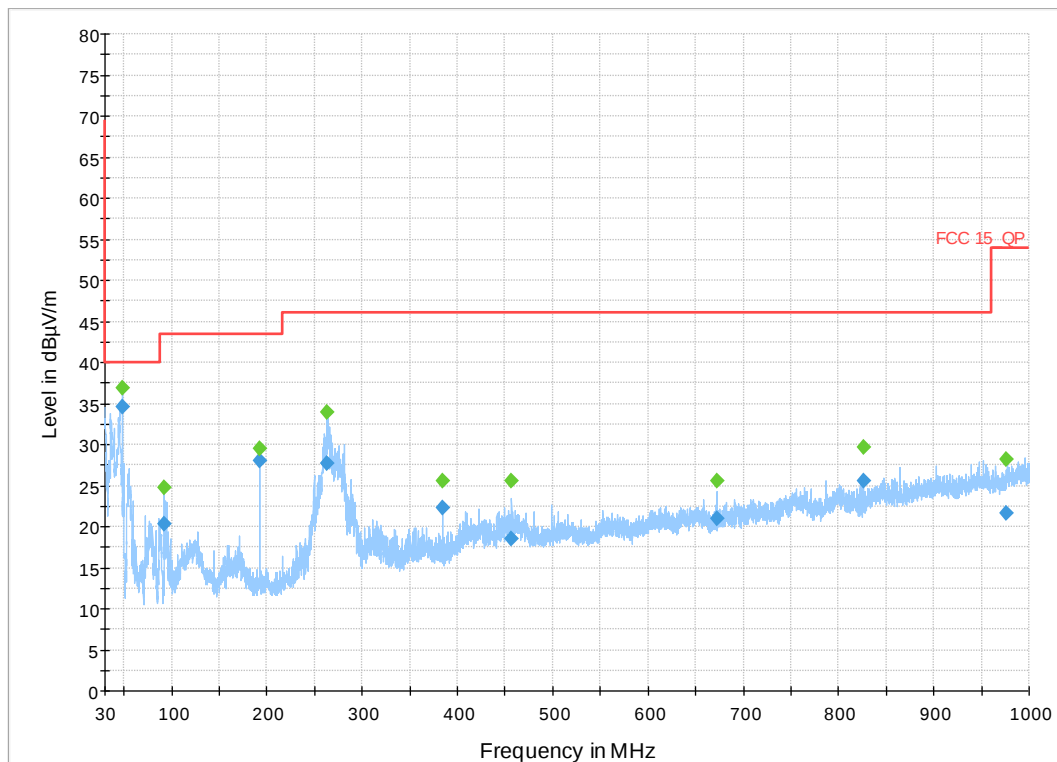
Figure 16: 30 MHz-1 GHz 802.11a Mode 20 MHz, Mid Channel
