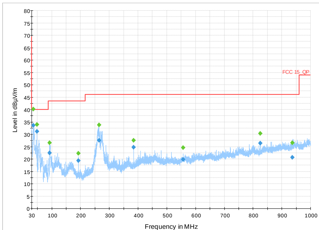
Figure 36: 30 MHz-1 GHz 802.11n HT Mode 40 MHz, Low Channel
