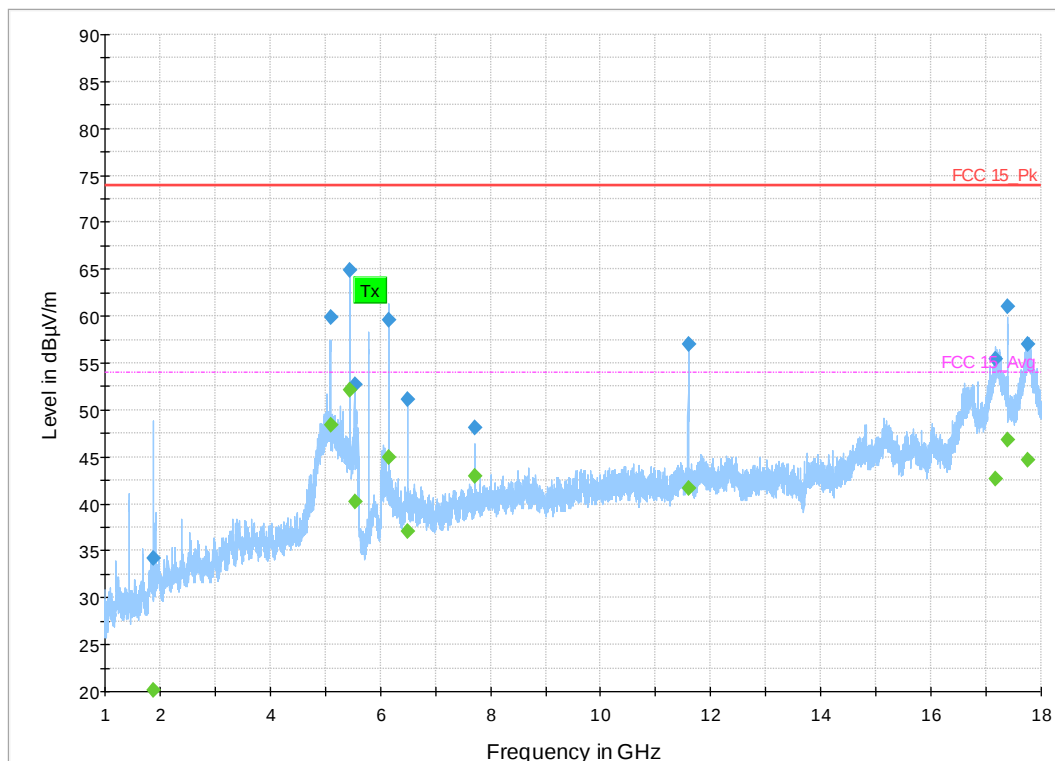
Figure 23: 1-18 GHz 802.11n HT Mode 5 MHz, Mid Channel
