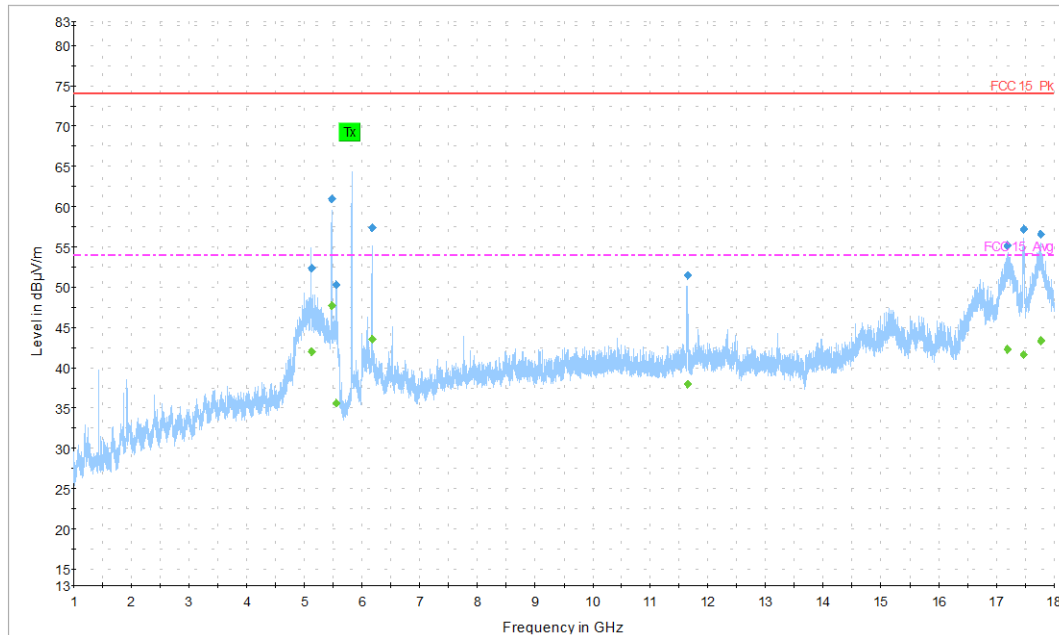
Figure 34: 1-18 GHz 802.11n HT Mode 20 MHz, High Channel
