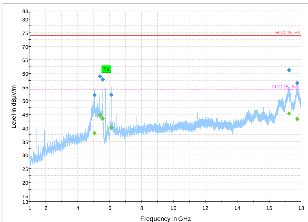
Figure 17: 1-18 GHz 802.11a Mode 20 MHz, Low Channel
