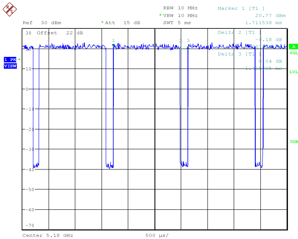
Figure 4: Duty Cycle for 802.11ac VHT20
