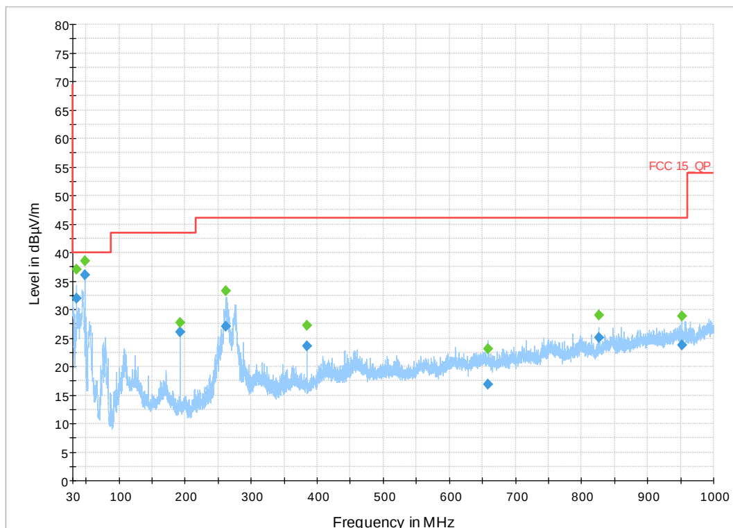
Figure 6: 30 MHz-1 GHz 802.11a Mode 5 MHz, Mid Channel
