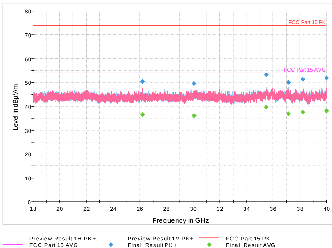
Figure 20: 18-40 GHz 802.11a Mode 20 MHz, Mid Channel
