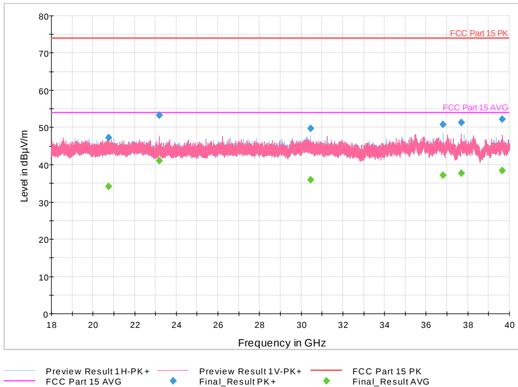
Figure 10: 18-40 GHz 802.11a Mode 5 MHz, Mid Channel
