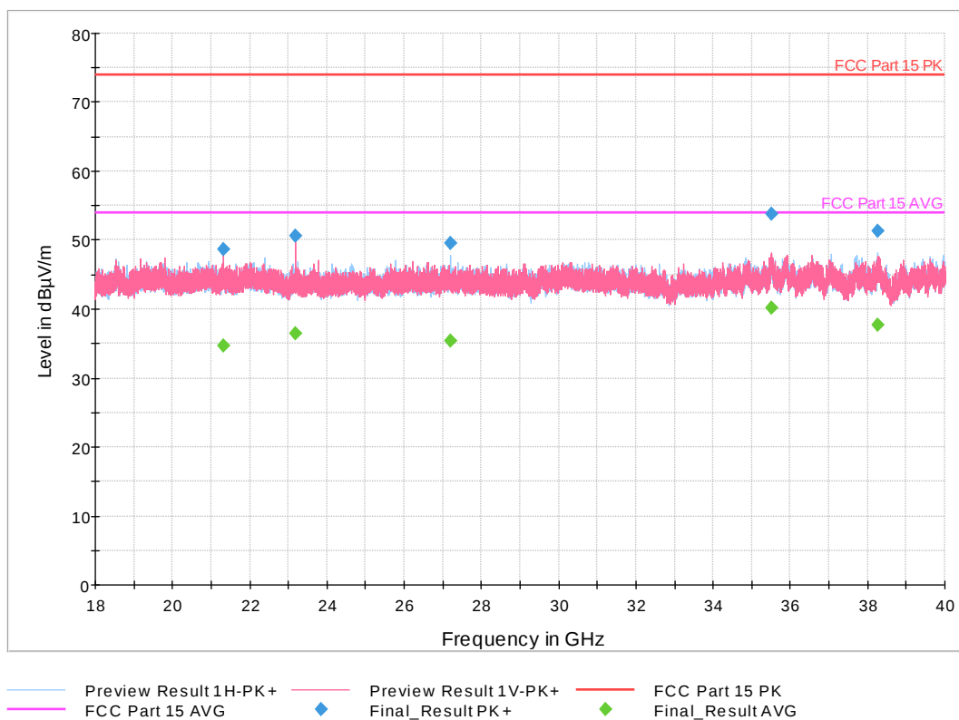
Figure 25: 18-40 GHz 802.11n HT Mode 5 MHz, Mid Channel
