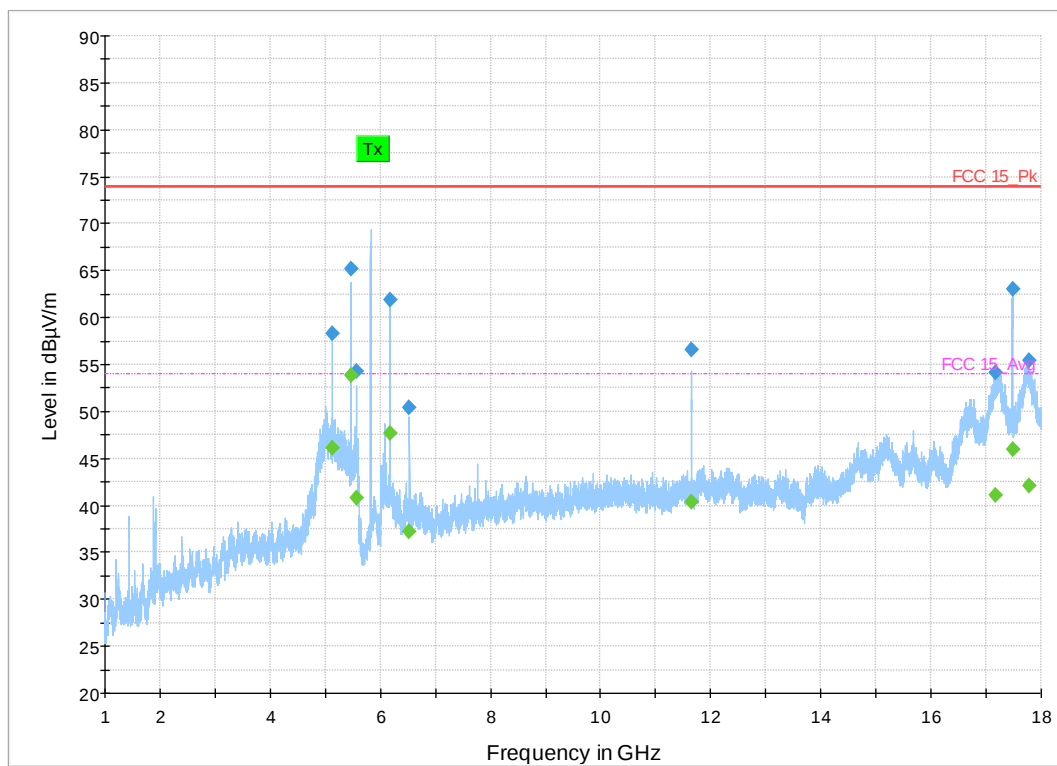
Figure 24: 1-18 GHz 802.1 n HT Mode 5 MHz, High Channel
