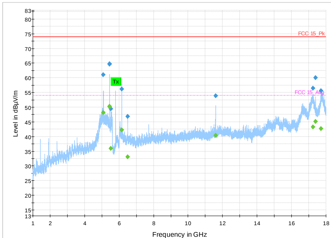
Figure 13: 1-18 GHz 802.11a Mode 10 MHz, Mid Channel
