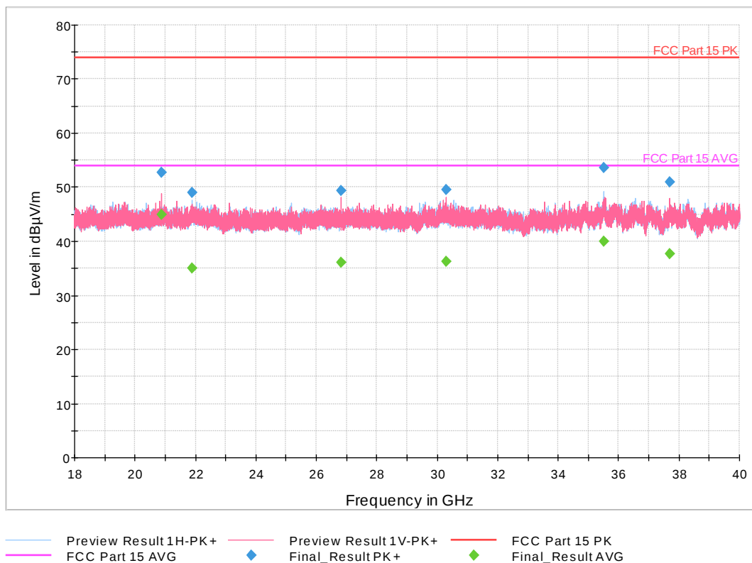
Figure 48: 18-40 GHz 802.11ac VHT Mode 40 MHz, Low Channel
