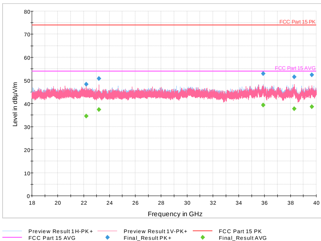
Figure 30: 18-40 GHz 802.11n HT Mode 10 MHz, Mid Channel
