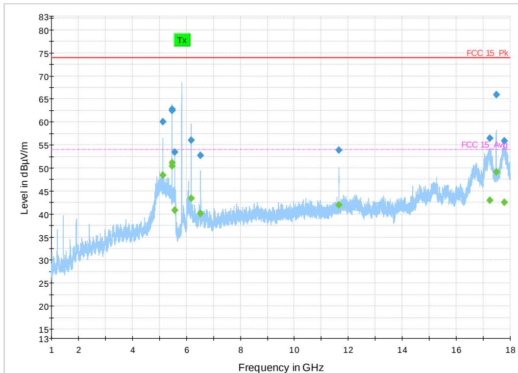
Figure 9: 1-18 GHz 802.11a Mode 5 MHz, High Channel
