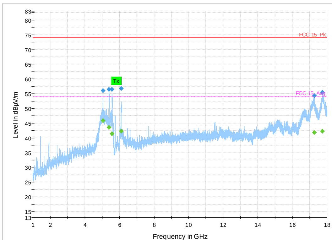
Figure 37: 1-18 GHz 802.11n HT Mode 40 MHz, Low Channel
