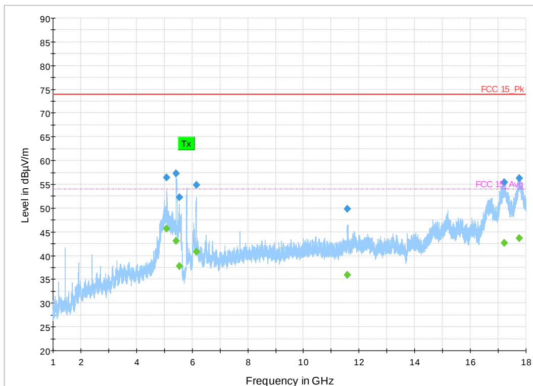
Figure 38: 1-18 GHz 802.11n HT Mode 40 MHz, High Channel
