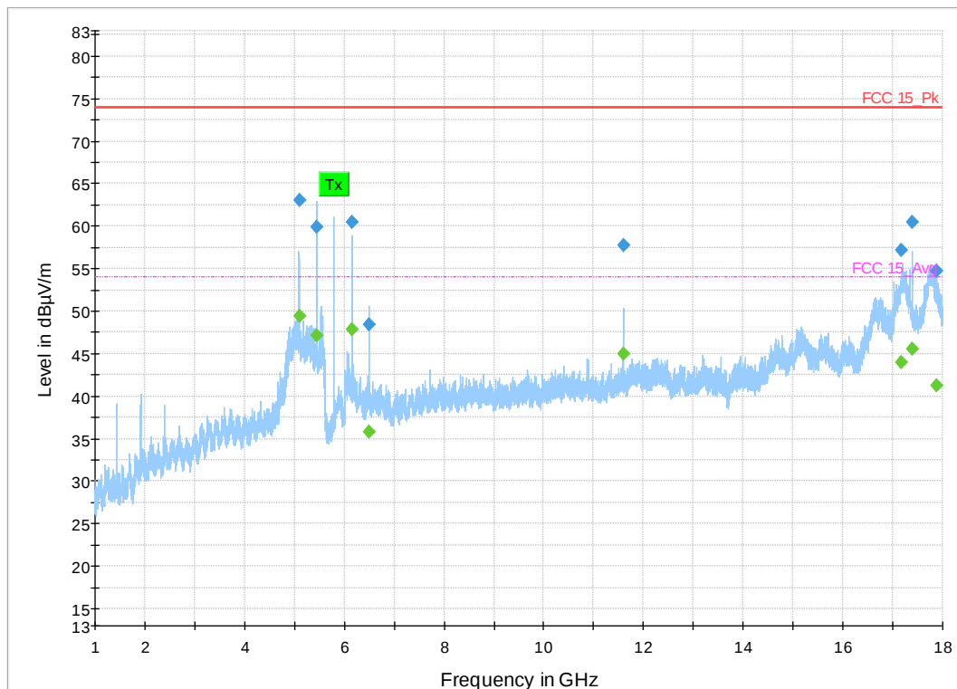
Figure 8: 1-18 GHz 802.11a Mode 5 MHz, Mid Channel
