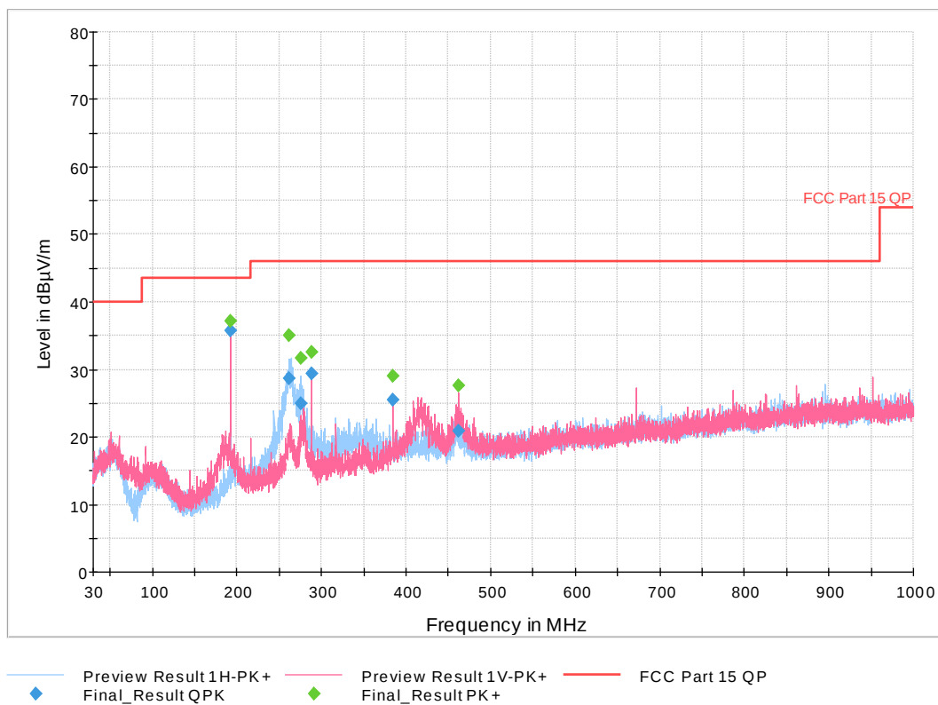
Figure 45: 30 MHz-1 GHz 802.11ac VHT Mode 40 MHz, Low Channel
