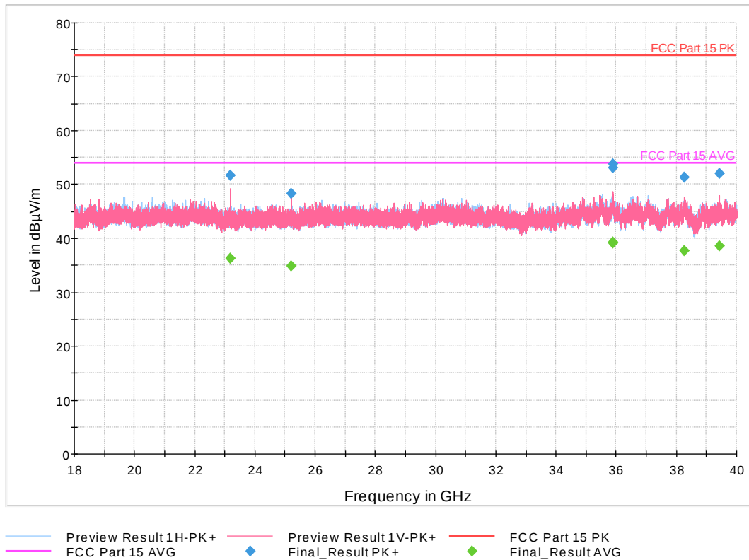
Figure 15: 18-40 GHz 802.11a Mode 10 MHz, Mid Channel
