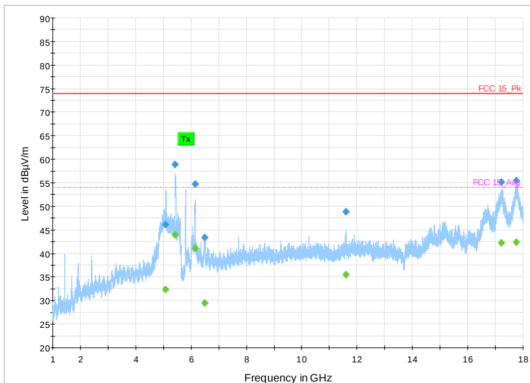
Figure 47: 1-18 GHz 802.11ac VHT Mode 40 MHz, High Channel
