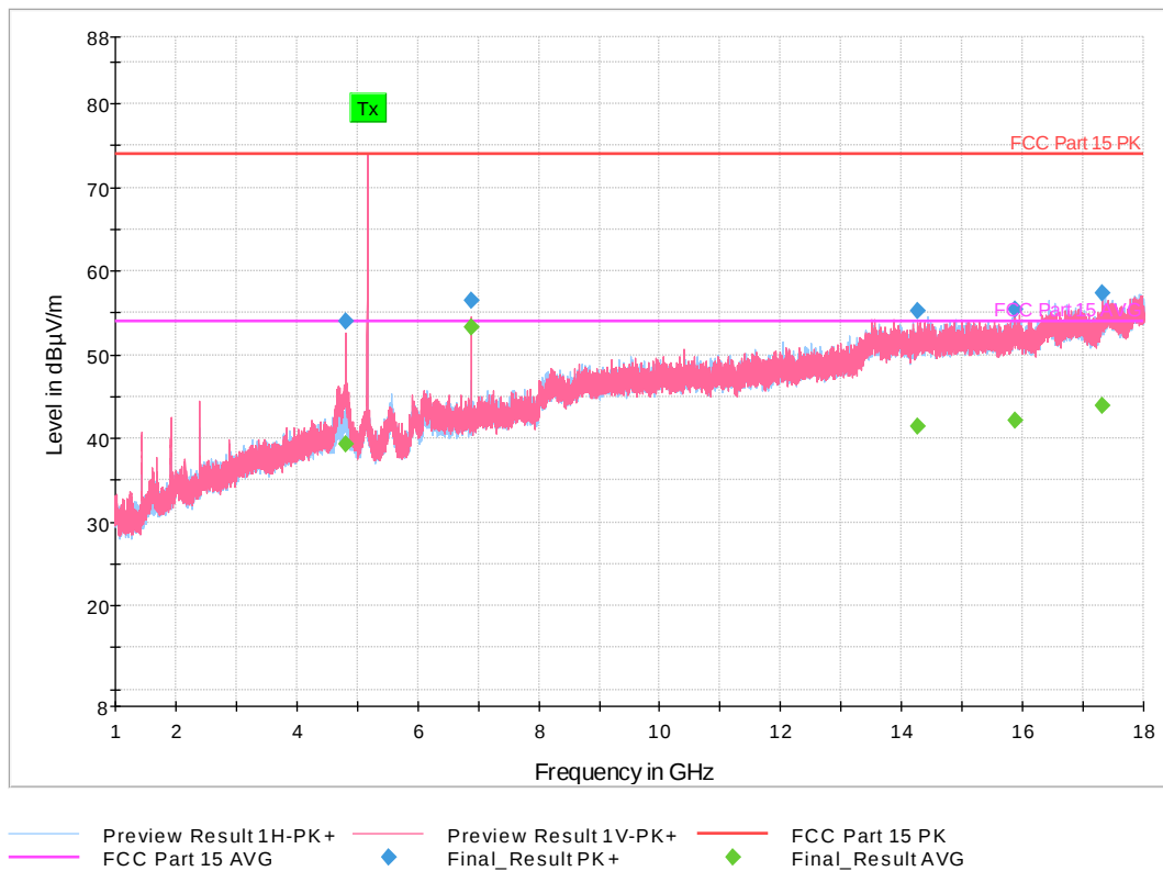
Figure 12: 1-18 GHz 802.11a Mode 10 MHz, Low Channel
