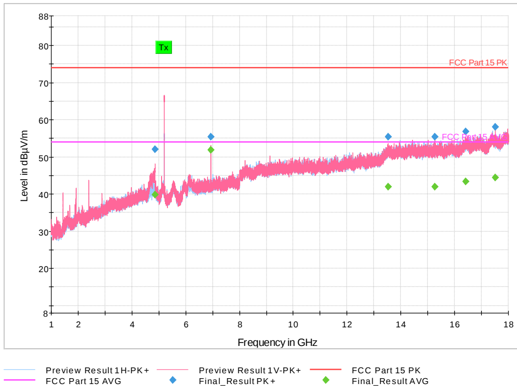
Figure 13: 1-18 GHz 802.11a Mode 10 MHz, Mid Channel
