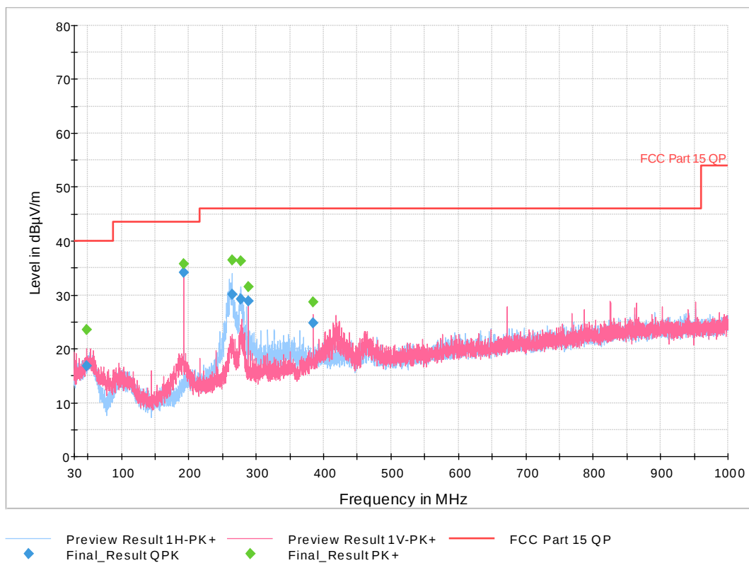
Figure 36: 30 MHz-1 GHz 802.11n HT Mode 40 MHz, High Channel
