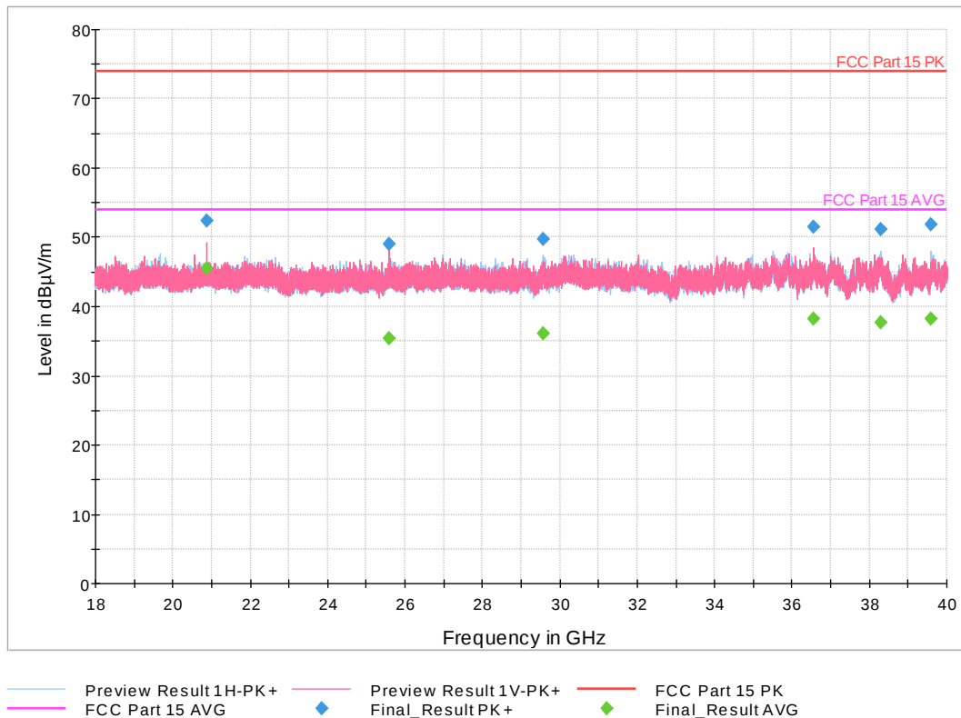
Figure 39: 18-40 GHz 802.11n HT Mode 40 MHz, High Channel
