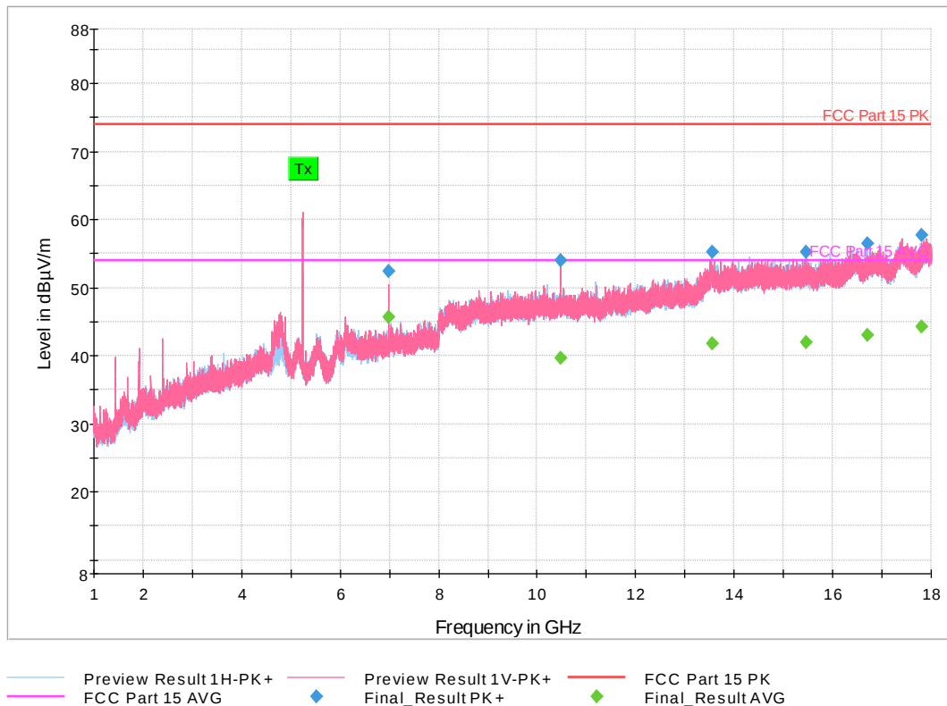
Figure 14: 1-18 GHz 802.11a Mode 10 MHz, High Channel
