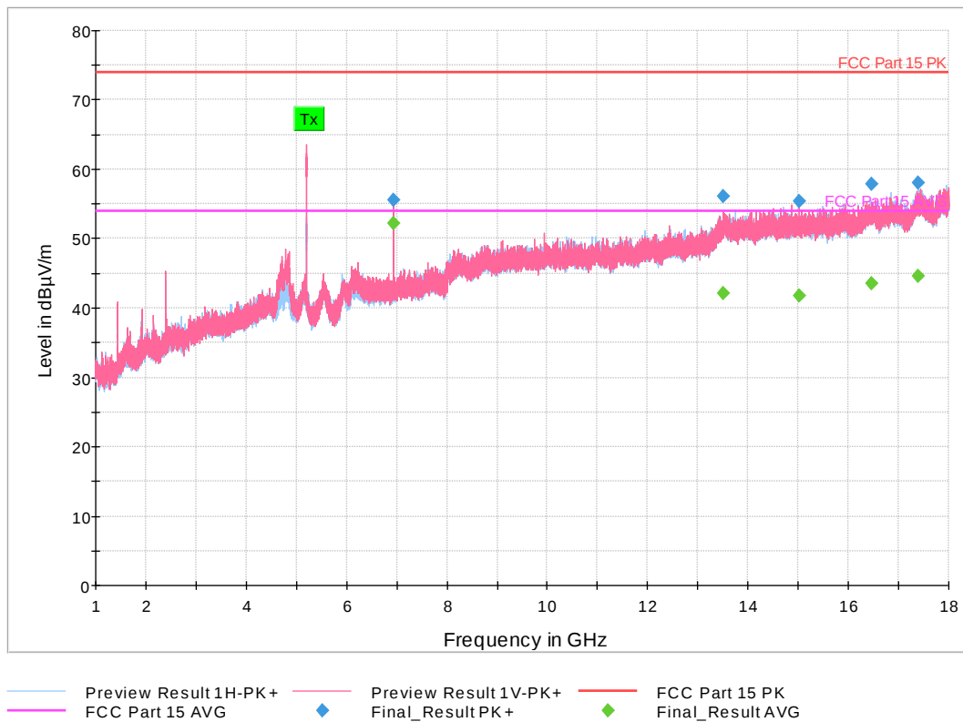
Figure 18: 1-18 GHz 802.11a Mode 20 MHz, Mid Channel
