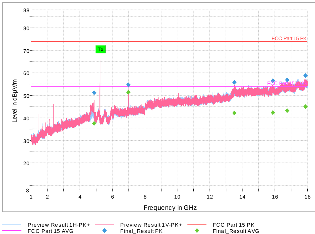
Figure 24: 1-18 GHz 802.1 n HT Mode 5 MHz, High Channel
