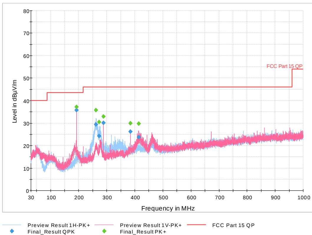
Figure 45: 30 MHz-1 GHz 802.11ac VHT Mode 40 MHz, High Channel
