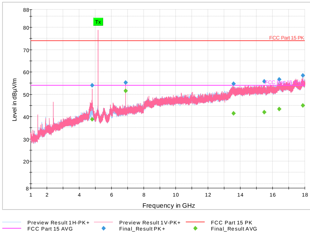
Figure 22: 1-18 GHz 802.11n HT Mode 5 MHz, Low Channel
