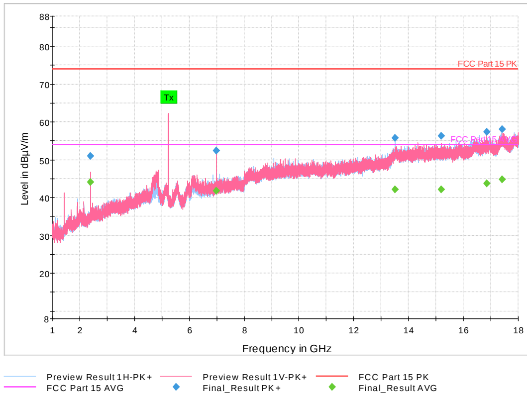
Figure 29: 1-18 GHz 802.11n HT Mode 10 MHz, High Channel
