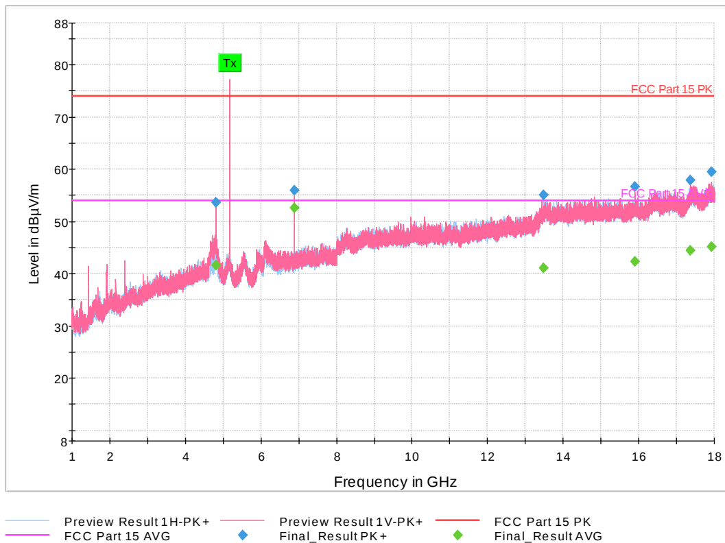
Figure 7: 1-18 GHz 802.11a Mode 5 MHz, Low Channel
