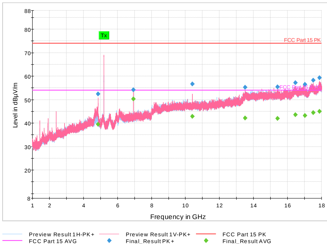
Figure 8: 1-18 GHz 802.11a Mode 5 MHz, Mid Channel
