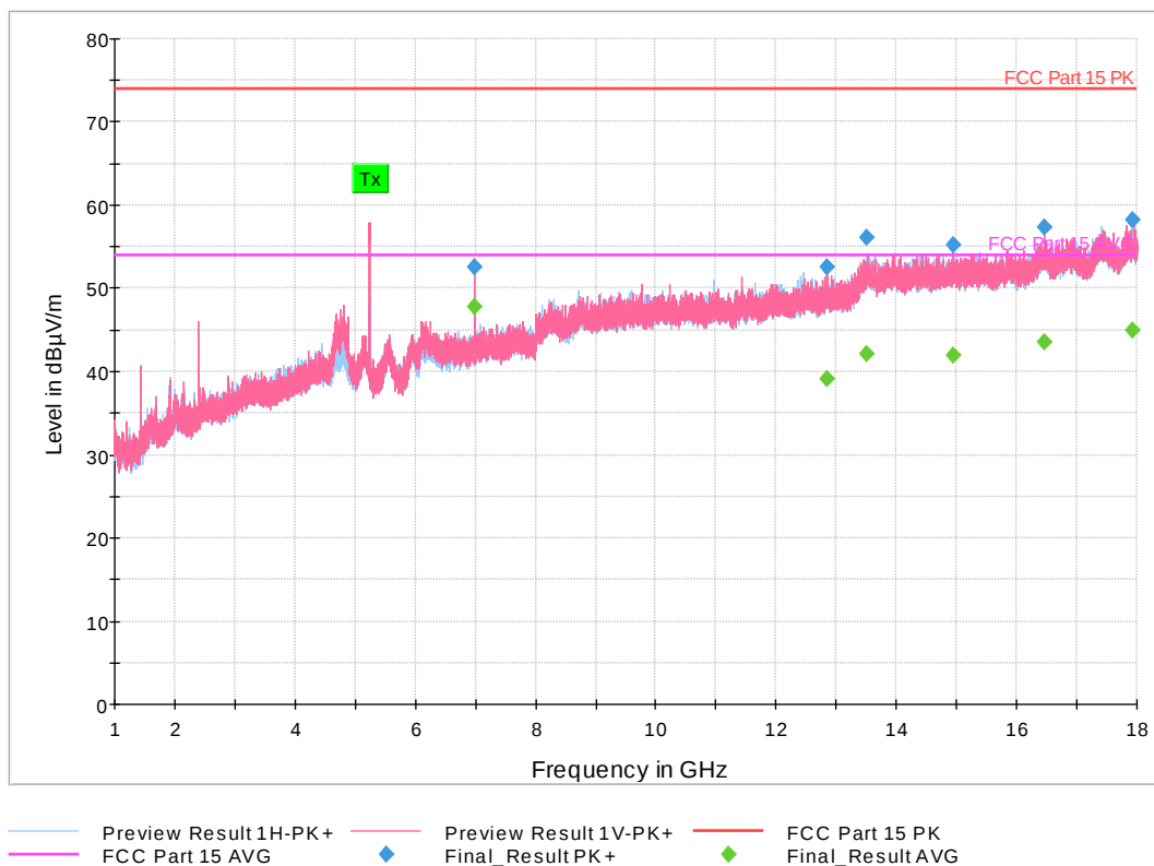
Figure 19: 1-18 GHz 802.11a Mode 20 MHz, High Channel
