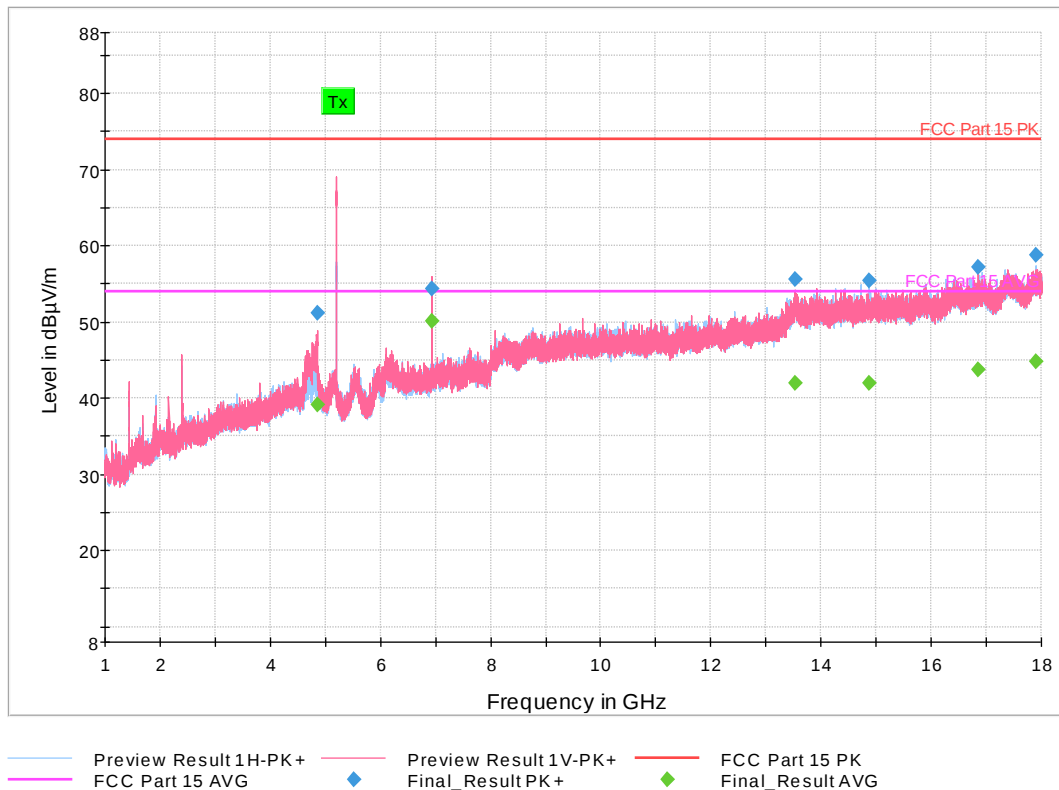
Figure 28: 1-18 GHz 802.11n HT Mode 10 MHz, Mid Channel
