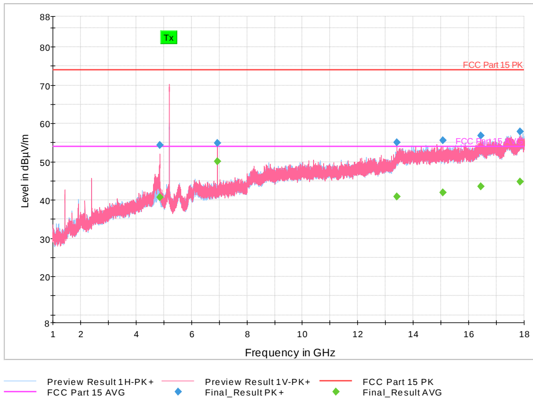
Figure 23: 1-18 GHz 802.11n HT Mode 5 MHz, Mid Channel
