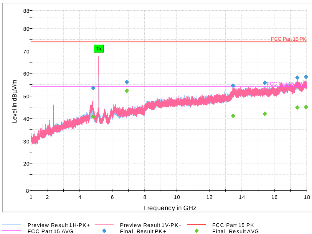
Figure 32: 1-18 GHz 802.11n HT Mode 20 MHz, Low Channel
