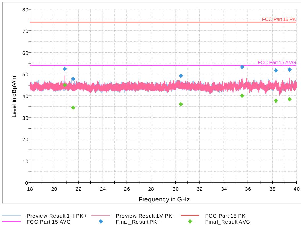
Figure 48: 18-40 GHz 802.11ac VHT Mode 40 MHz, High Channel
