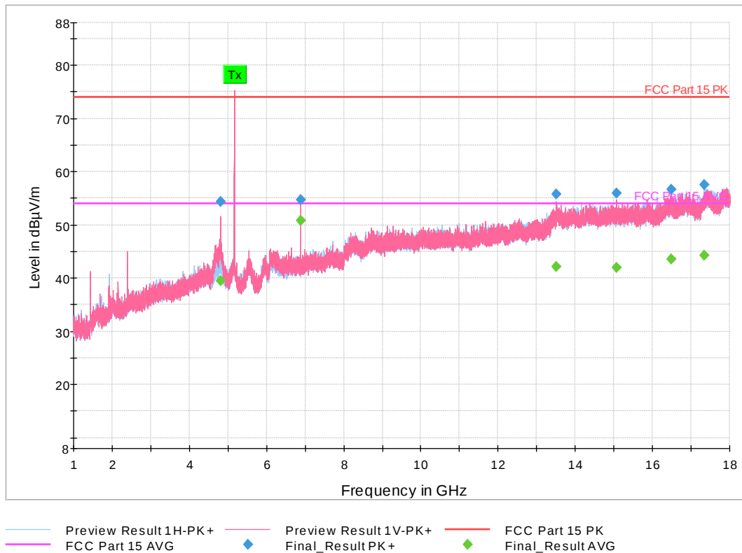
Figure 27: 1-18 GHz 802.11n HT Mode 10 MHz, Low Channel
