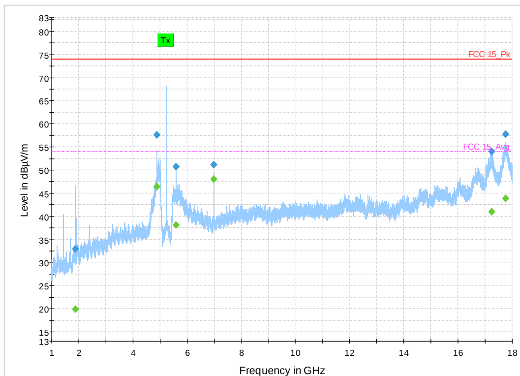
Figure 34: 1-18 GHz 802.11n HT Mode 20 MHz, High Channel
