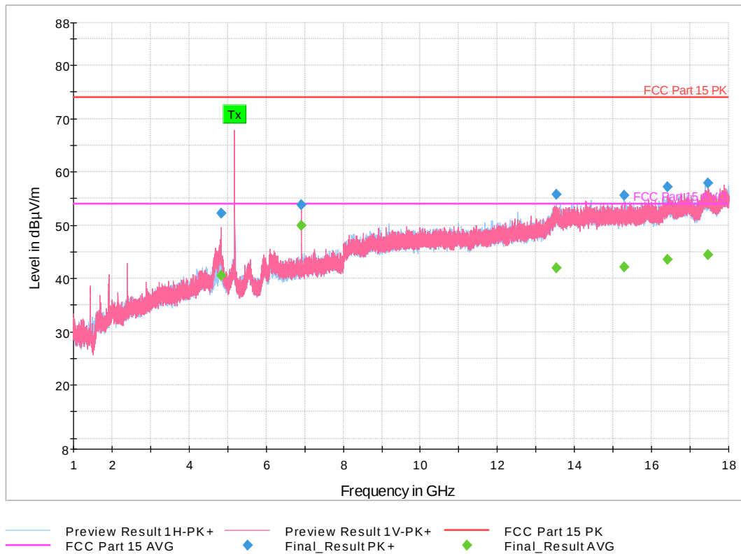
Figure 17: 1-18 GHz 802.11a Mode 20 MHz, Low Channel
