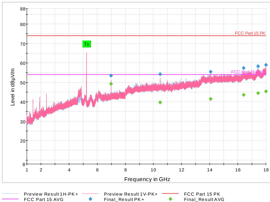
Figure 9: 1-18 GHz 802.11a Mode 5 MHz, High Channel
