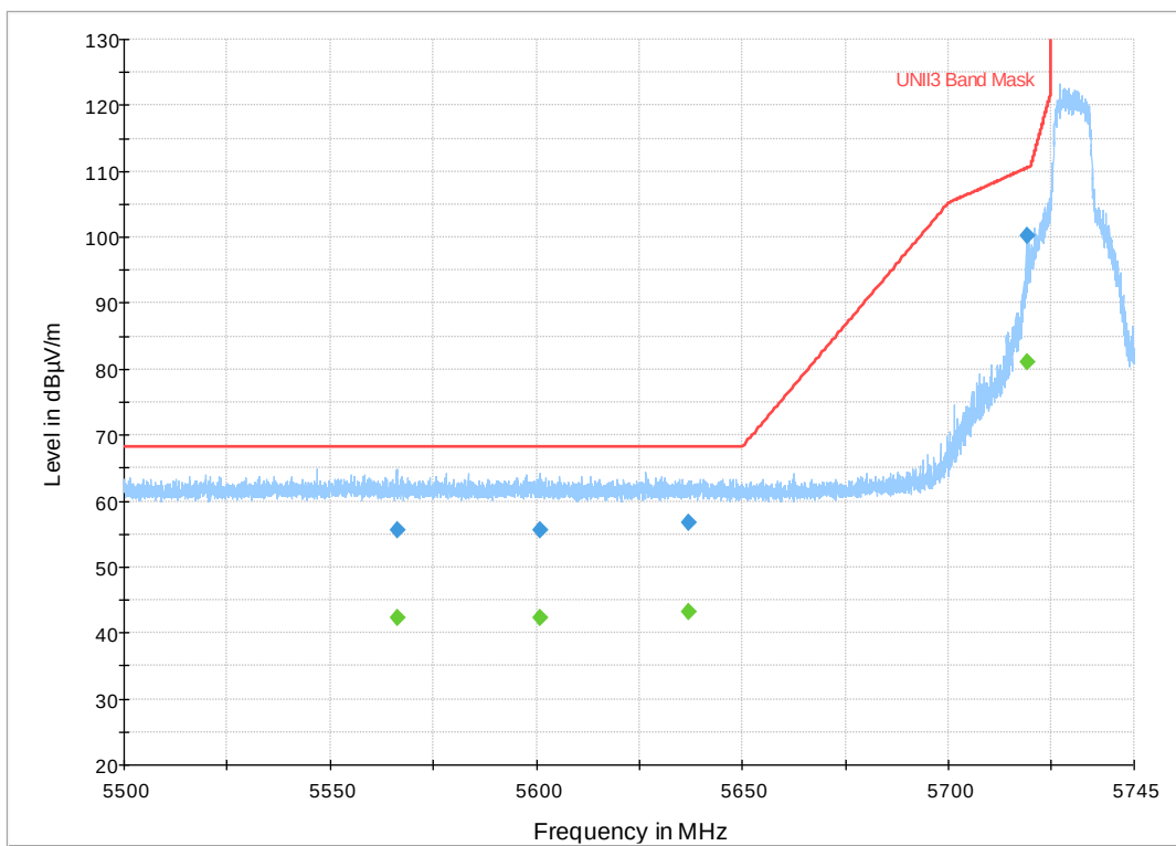
Figure 19: Low Band Edge 802.11n HT Mode 10 MHz, Low Channel
