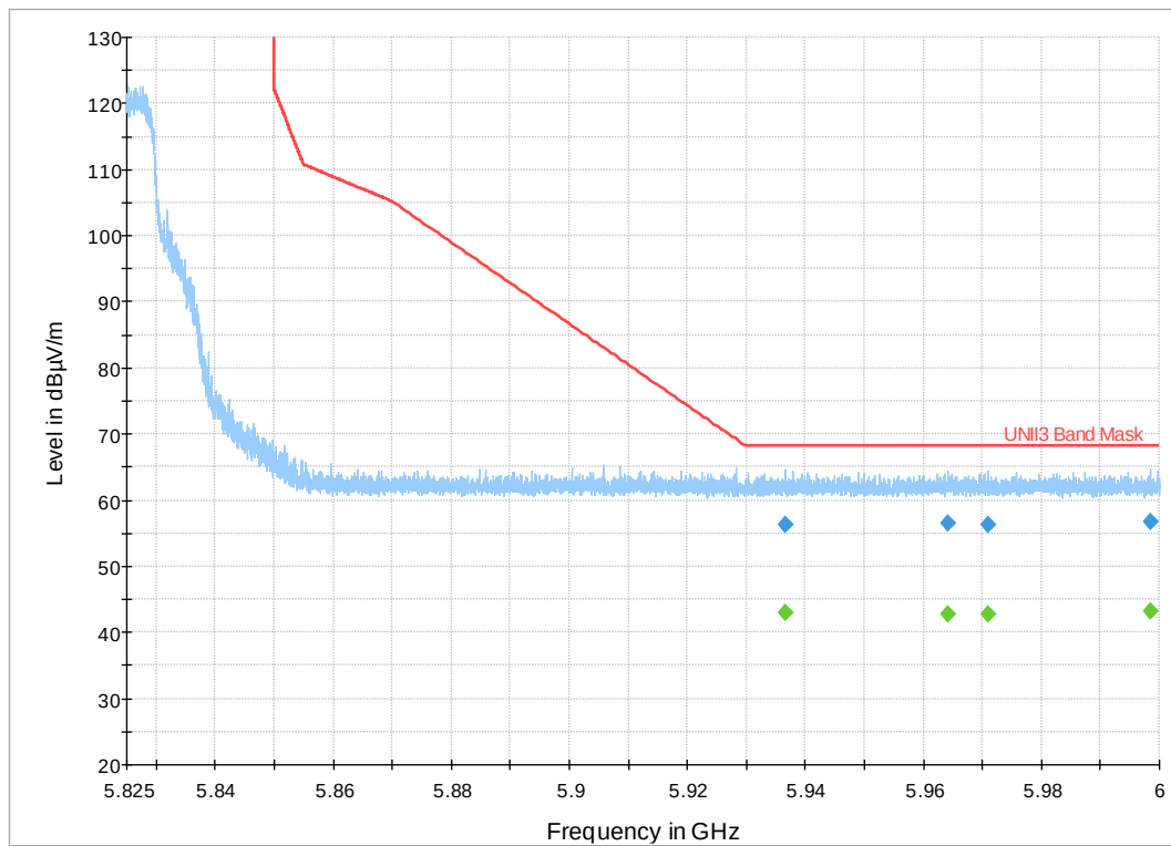
Figure 28: High Band Edge 802.11n HT Mode 10 MHz, High Channel
