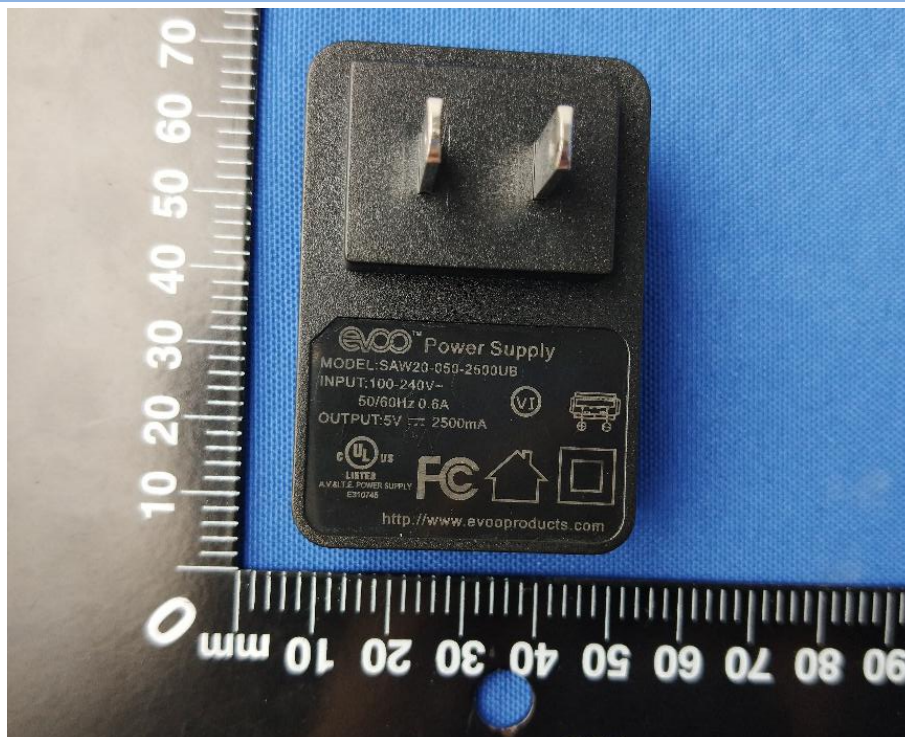
Accessory-Power Adapter
