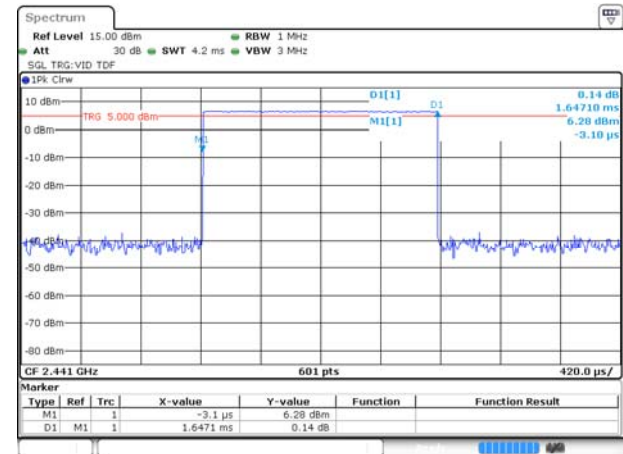
GFSK DH3
