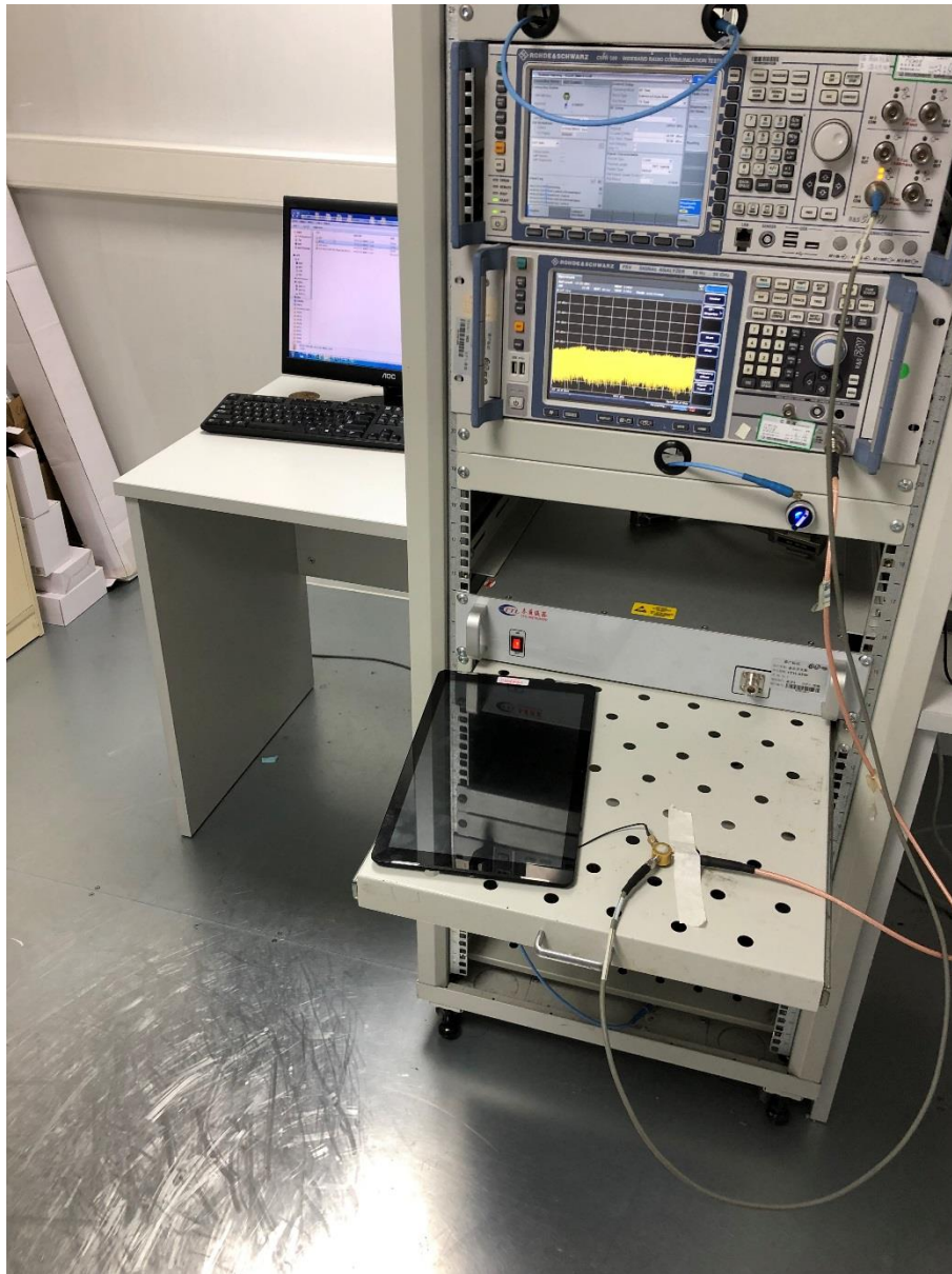
Conducted Test-BT3.0
