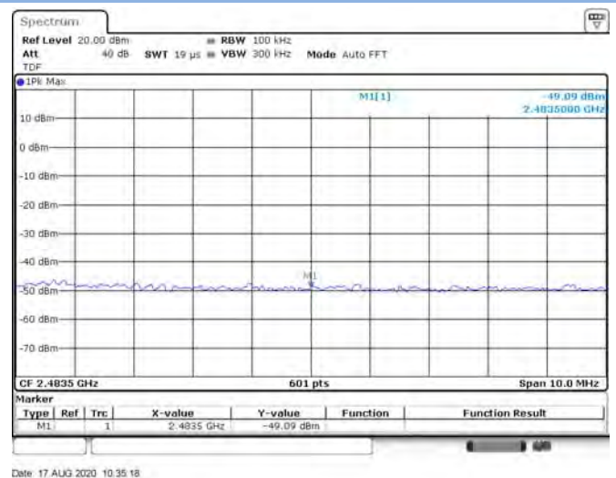
802.11b HIGH CHANNEL, Reference level
