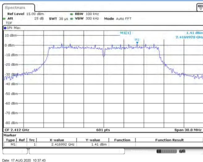
802.11g LOW CHANNEL, Carrier level
