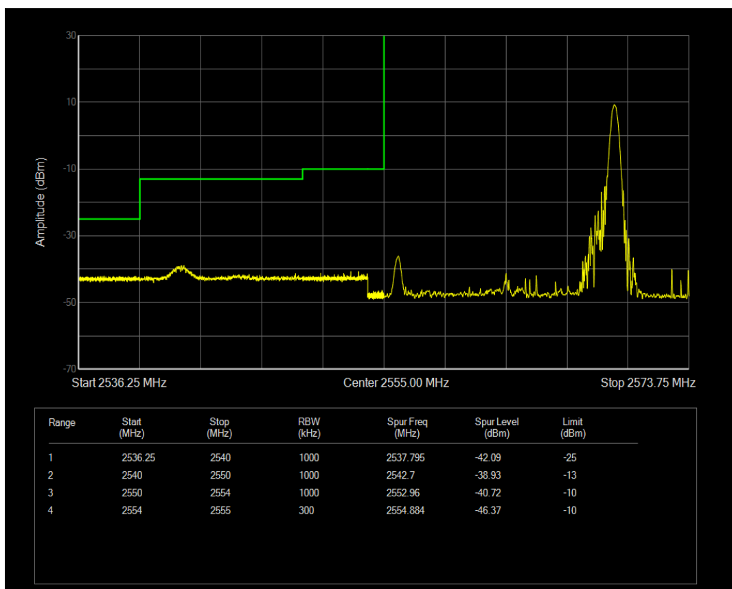
LTE Band41 QPSK BW=20MHz Channel=40340 RB Size=1 Position=#0
