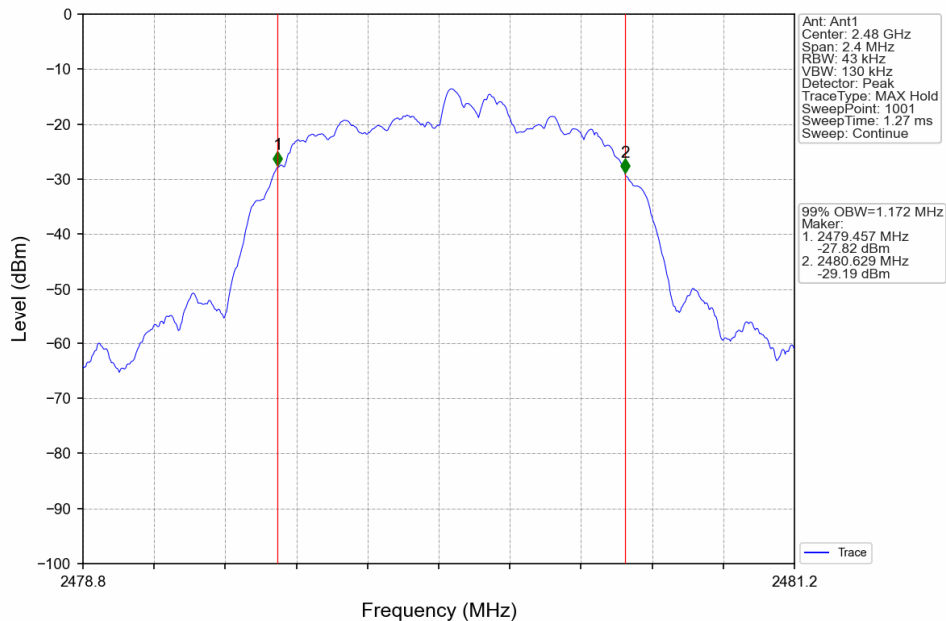
Pi/4DQPSK_2DH5_HCH_2480MHz_Ant1_NTNV
