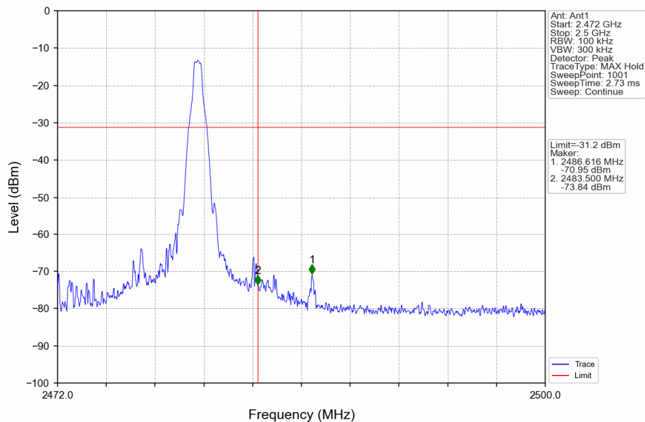
GFSK_DH5_HCH_2480MHz_Ant1_NTNV
