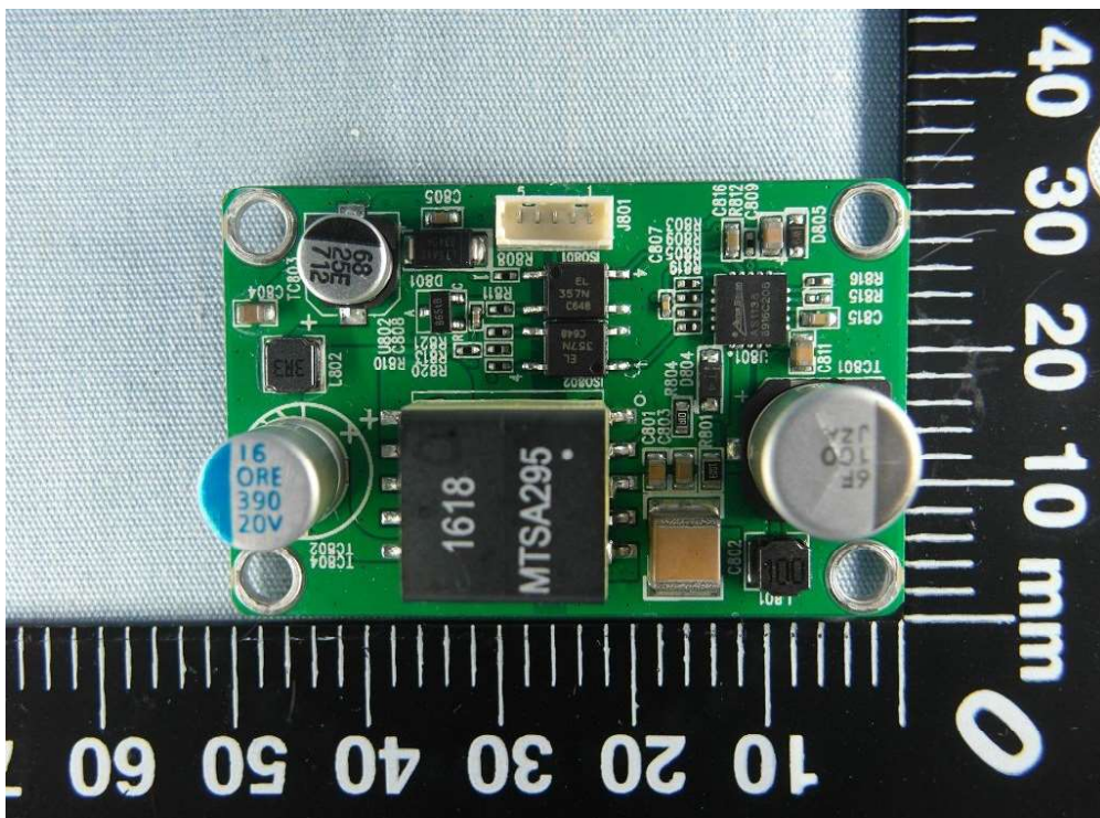
(28) EUT Photo
