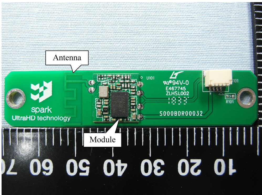
(32) EUT Photo
