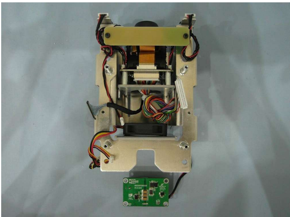
(26) EUT Photo
