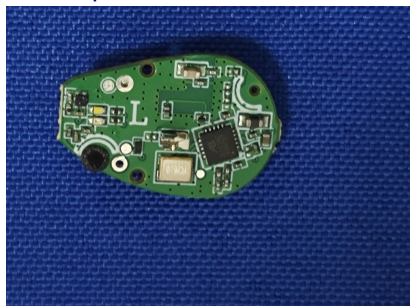
Left earphone:
