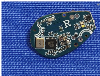
Right earphone:
