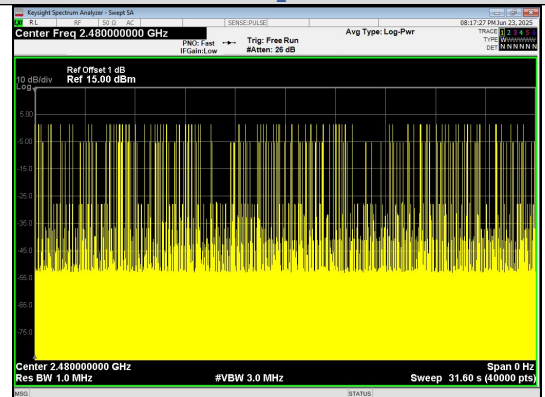
Number of Pulses in 31.6 seconds \pi/4 QPSK_2-DH5
