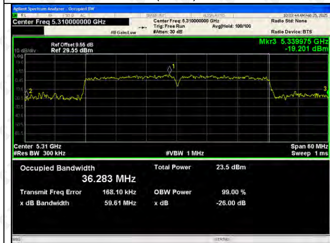
8802.11n(VH40)-5310
