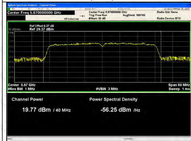
802.11n(VH40)-5670
