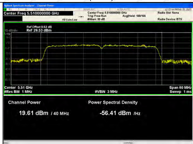
802.11n(VH40)-5510
