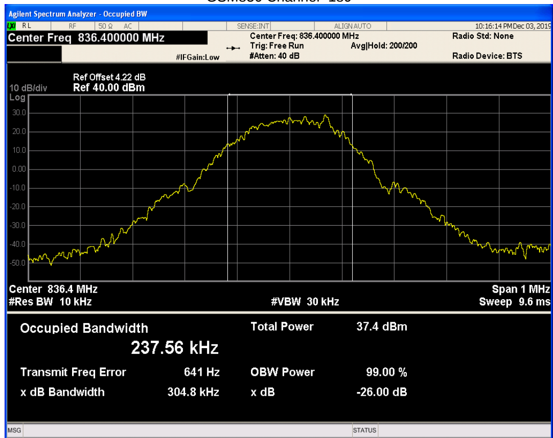
GSM850 Channel=189
