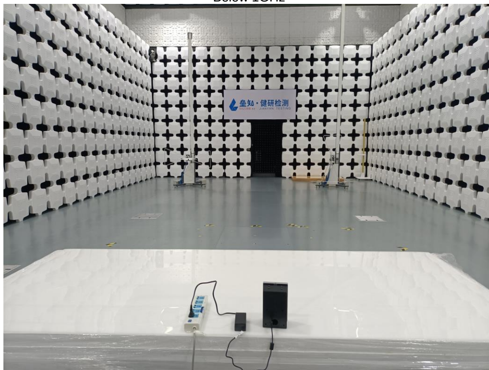
Radiated Emission(DC power supply) Below 1GHz
