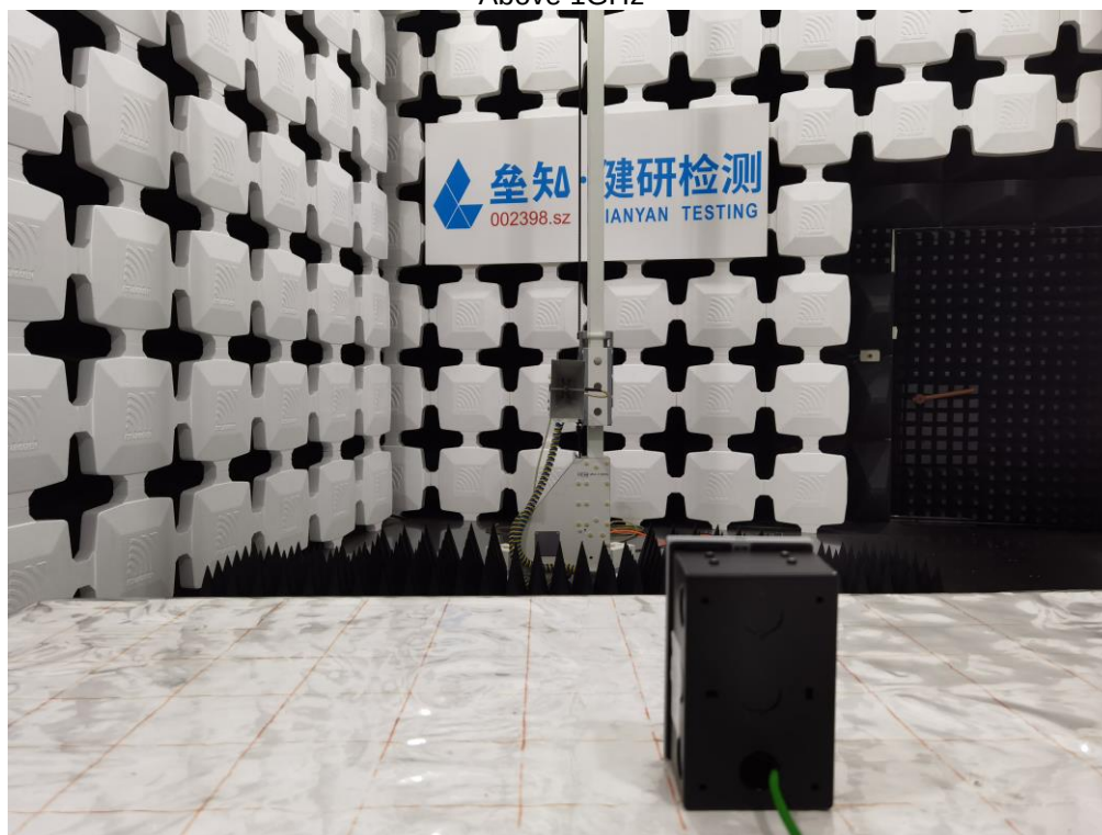
Radiated Emission(POE power supply) Above 1GHz
