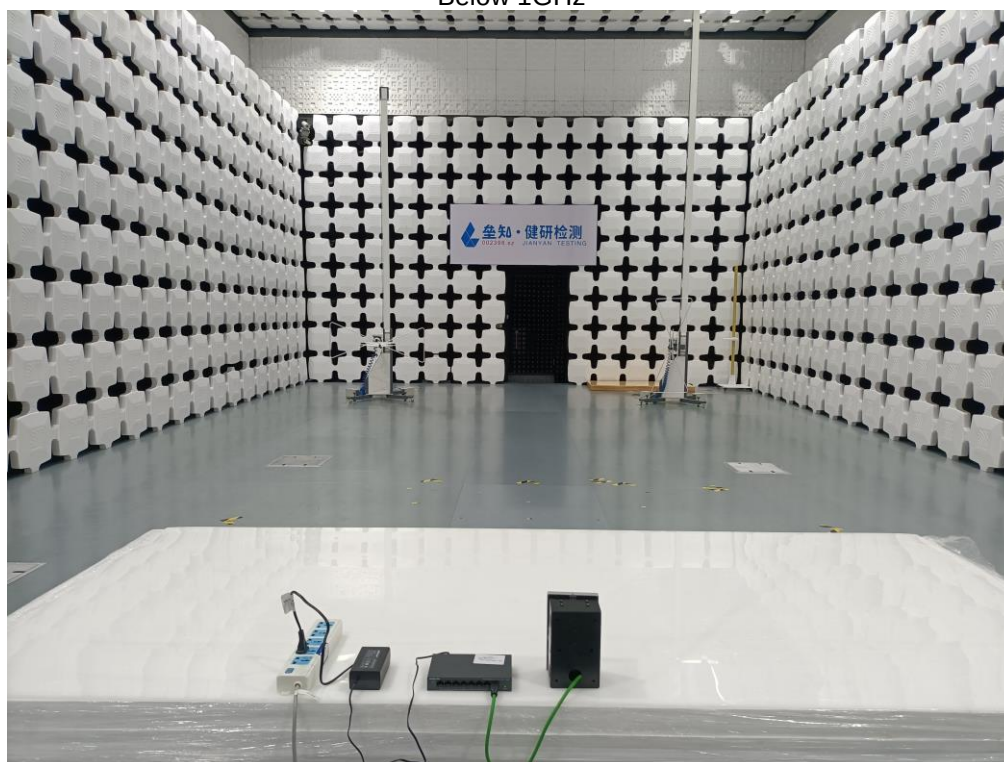
Radiated Emission(POE power supply) Below 1GHz
