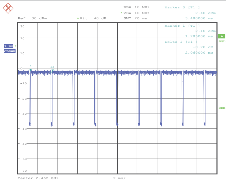
Test Graph_ ANT1/HCH Duty Cycle:
