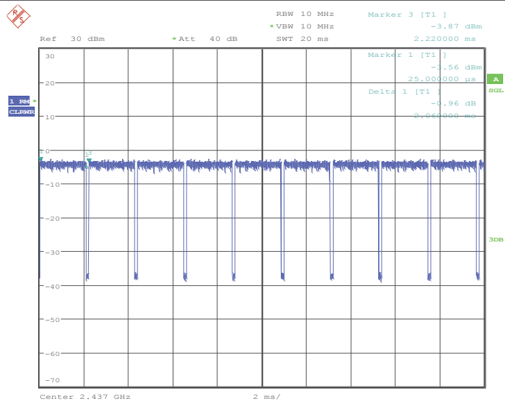
Test Graph_ ANT3/MCH Duty Cycle:
