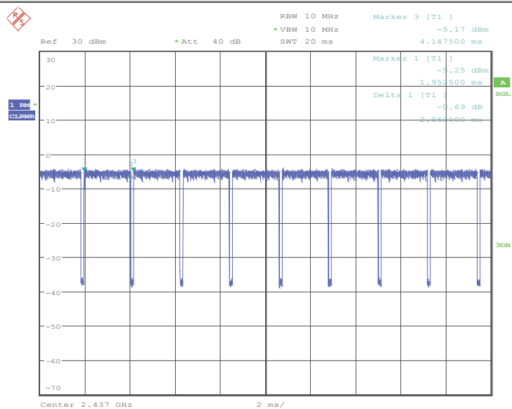
Test Graph_ ANT2/MCH Duty Cycle:
