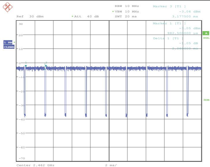
Test Graph_ ANT3/HCH Duty Cycle:
