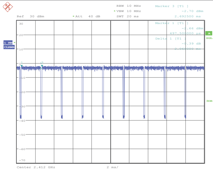
Test Graph_ ANT2/LCH Duty Cycle:
