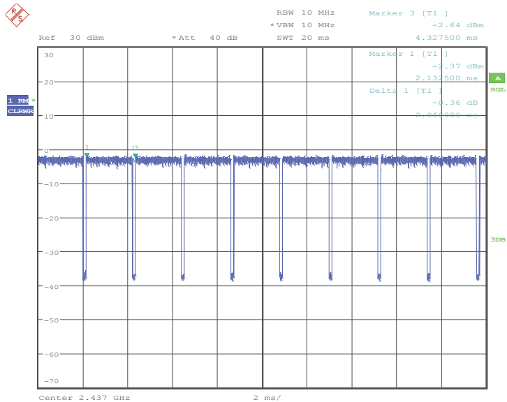
Test Graph_ ANT1/MCH Duty Cycle:
