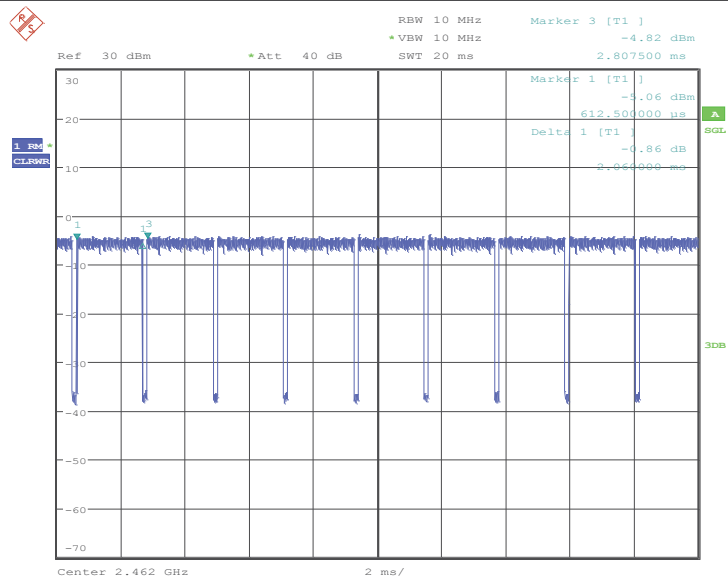
Test Graph_ ANT2/HCH Duty Cycle:
