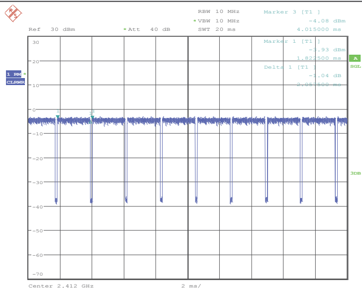
Test Graph_ ANT3/LCH Duty Cycle:
