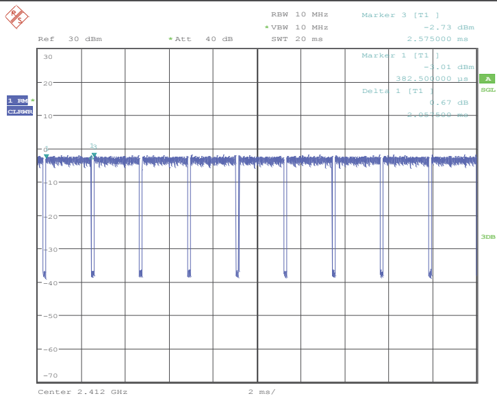
Test Graph_ ANT1/LCH Duty Cycle:
