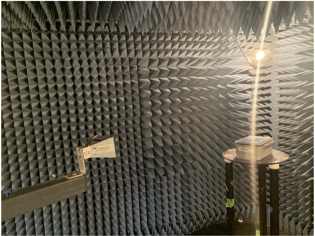
Photograph 3. Radiated Emission Test Setup - 18 GHz – 40 GHz
