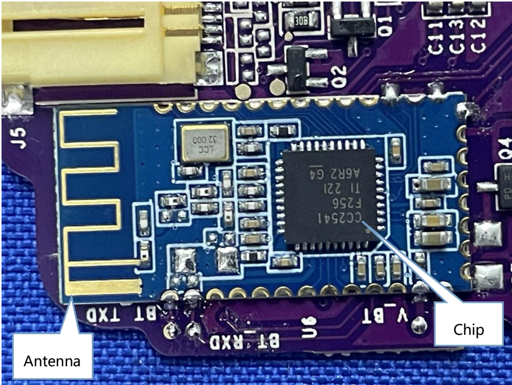
Antenna Position ***End of the report***
